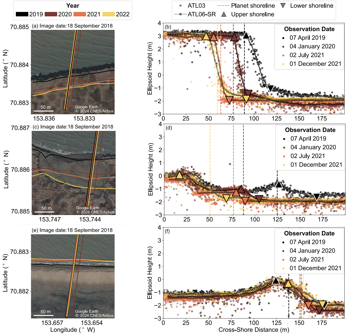
Figure 6. (a), (c), (e): Detailed view of the ICESat-2 sampling location from 2018 satellite imagery (©2024 Google Earth Imagery CNES/Airbus ) for (a) ground track 3r; (c) ground track 2r and (e) ground track 1r. The location of the Planet shoreline and corresponding ICESat-2 pass for each year is shown. (b), (d), (f): ATL03 photon clouds from each ICESat-2 pass, with the SlideRule-derived SlideRule-derived (ATL06-SR) elevation profile overlain-overlaid on the photon clouds for (b) ground track 3r; (d) ground track 2r; and (f) ground track 1r. The estimated location of the upper and lower shoreline boundary for each date is marked, along with the cross-shore locations of the Planet-derived shorelines. The colors follow the same legend as (a), (c), and (e).
