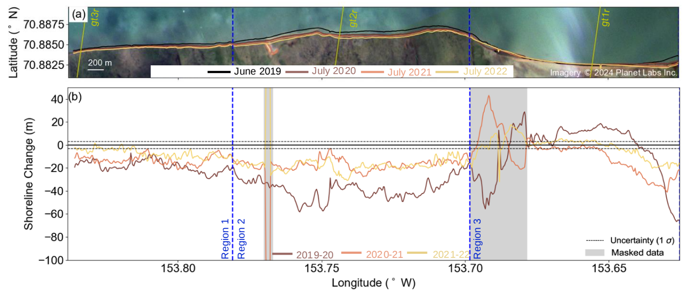
Figure 3. (a) Shorelines derived from Planet images, overlain on imagery from 07/25/2020-2020 ( ©2024 Planet Labs Inc. ). The locations of the three ICESat-2 ground track are also shown. (b) Cross-shore shoreline change calculated between successive years. Areas where there was an ambiguous land/water boundary are masked out (shaded areas) and excluded from analysis. The boundaries of the three region shown in Fig. 1 are shown as dashed lines.
