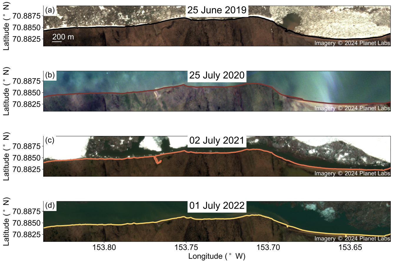
Figure 2. Planet Labs imagery (Planet Team, 2023) (©2024 Planet Labs Inc) used to estimate shoreline positions. Shorelines delineated using Otsu thresholding are overlain and show good agreement with the visible land-water boundary.
