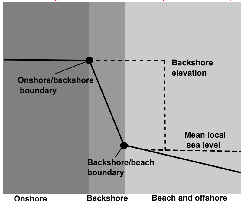
Figure A2. Illustration of the boundaries and elevation estimates described in Section 2.4
