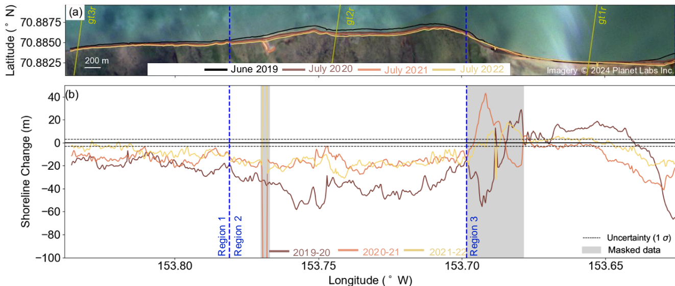
Figure 3. (a) Shorelines derived from Planet images, overlain on imagery from 07/25/2020. The locations of the three ICESat-2 ground track are also shown. (b) North-south Cross-shore shoreline change calculated between successive years. Areas where there was an ambiguous ambiguous land/water boundary are masked out (shaded areas) and excluded from analysis. The boundaries of the three region shown in Fig. 1 are shown as dashed lines.
