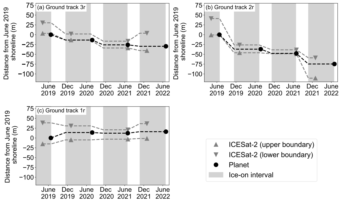
Figure 4. Time series of the position of upper and lower boundaries and coastal boundaries from ICESat-2 and the land-water boundary derived from Planet. Positions are given with respect to as the location of cross-shore distance from the Planet-derived shoreline from 25 June 2019 . Ice-on intervals are shaded. Dashed lines indicate the trajectory of the shoreline based on a linear rate of change during the open water season and no change during ice-on periods.
