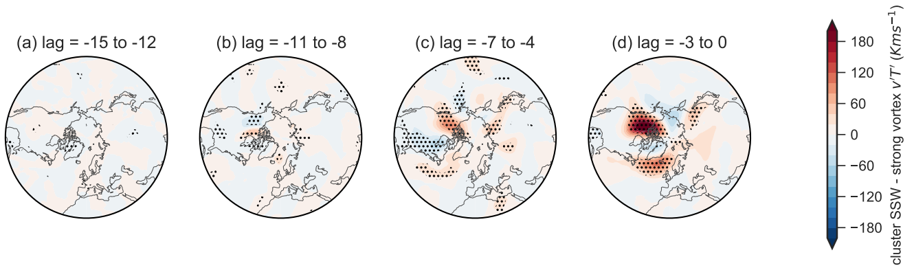
Figure A4. Difference between the SSW cluster and the strong vortex cluster in eddy heat flux ( v'T' ) at 100hPa for the hindcast of the 2018 SSW. Stippling indicates a significant difference between the two clusters by a t-test at the 95% confidence interval.
