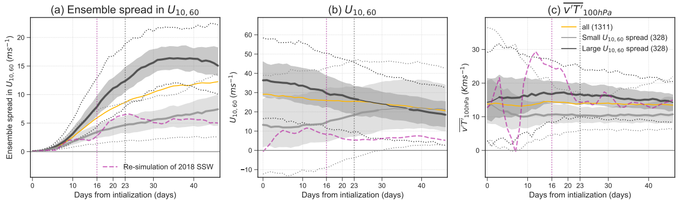
Figure 1. Evolution of (a) ensemble spread in U_{10,60} and (b) ensemble mean of U_{10,60} and (c) ensemble mean of \overline{v'T'} at 100hPa in composites of hindcasts classified as having large uncertainty (large U_{10,60} spread, black) and small uncertainty (small U_{10,60} spread, grey), respectively, for the prediction of the stratospheric polar vortex. The solid line denotes the median, the shaded region denotes the 25th to 75th percentiles, and dotted lines denote the 5th and 95th percentiles, for the large and small spread composites. The median of all hindcasts is shown in yellow. Solid lines are printed in bold when the composites are significantly different from all hindcasts at the 95% confidence interval using a t-test. The purple dashed line in (a) corresponds to the ensemble spread of the hindcast of the 2018 SSW event, and the purple dashed lines in (b) and (c) correspond to the ensemble mean of the hindcast for the 2018 SSW. Dotted vertical purple and grey lines indicate the onset and the peak of the uncertainty in U_{10,60} for the 2018 SSW event, respectively. The number of hindcasts in each composite is given in brackets in the legend.
