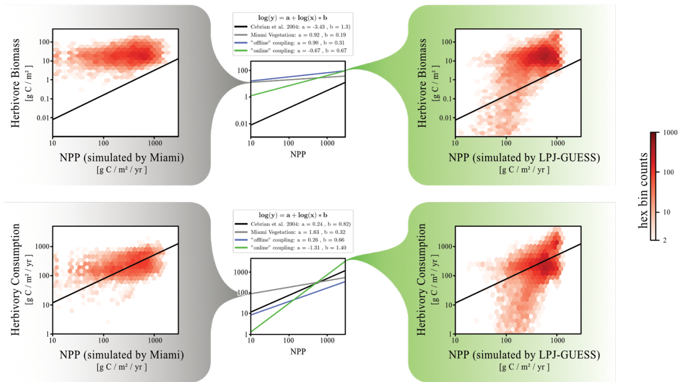
Figure 10: Power-law relationship between herbivore biomass and grid cell productivity, as well as herbivory consumptions and grid cell productivity. The red saturation of each hexagon represents the number of data points found in the model system that matches the NPP and the herbivore biomass (or herbivory consumption) of that hexagon's position in the grid. The left distributions show data from "default" Madingley (driven by the Miami model), while the right distributions show data from "online" Madingley. In the middle of the figure, power-law relationships are summarised for all three Madingley model versions. The black line in each plot displays the power-law derived by Cebrian (2004).
