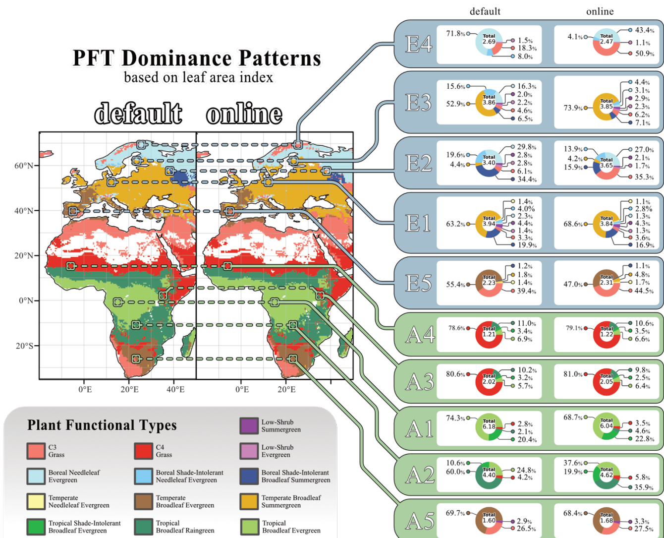
275 Figure 5: Coupling-related changes in grid cell's dominant PFT. The maps display the dominant PFT in each grid cell, determined by the PFT's LAI in the “default” and “online” simulations. Only grid cells with a total LAI greater than 1 were included in the analysis. Flanking the maps, pie charts show the contributions of all PFTs to the total LAI for ten selected locations. The “default” simulation results are presented on the left, while those from the “online” simulation are shown on the right. The figure reflects data averaged over the final 30 years of the simulations. PFT Colour coding is labelled underneath the figure.
