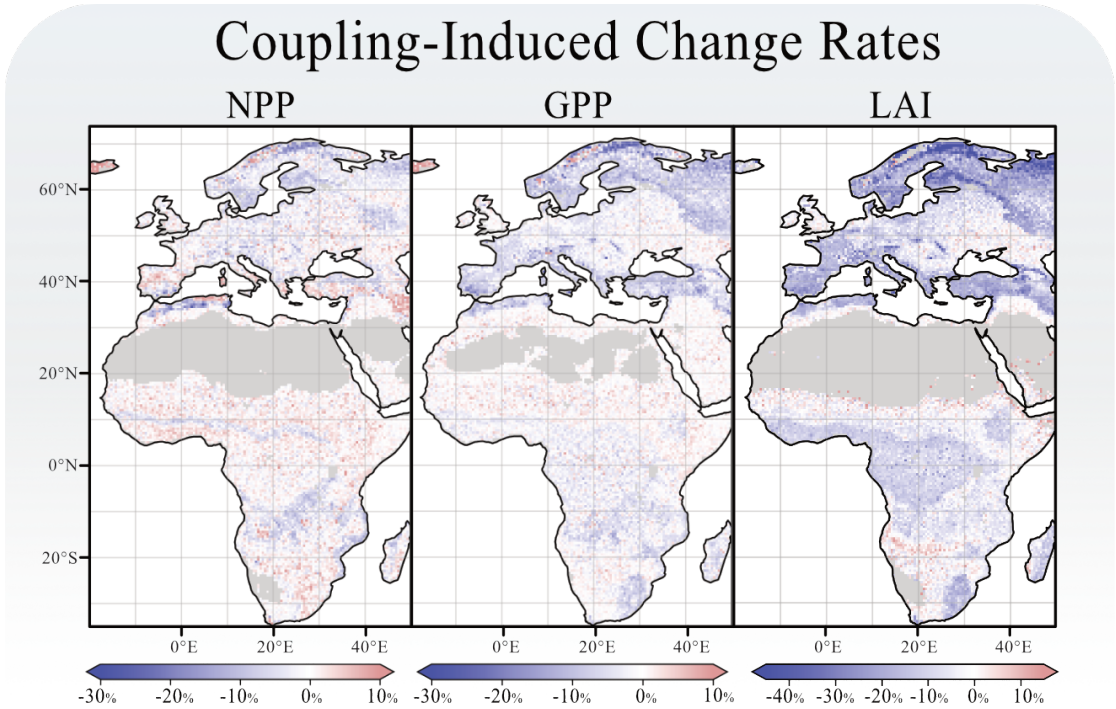
235 Figure 3: Coupling related changes in grid cell's NPP, GPP and LAI. Each panel shows the percentage-wise difference caused by the coupling. All figures were rendered over the last 30 years of the simulation.
