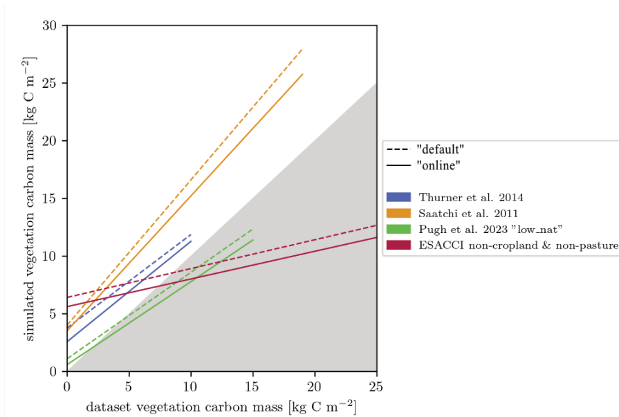
355 Figure 9: Linear fit of simulated and measured vegetation carbon mass for four datasets. The non-cropland & non-pasture dataset is based on the ESA aboveground biomass (Santoro and Cartus, 2023) and the ESA land cover datasets (ESA Land Cover Climate Change Initiative (Land_Cover_cci): Global Land Cover Maps, Version 2.0.7, 2024). AGB was converted into total vegetation carbon mass.
