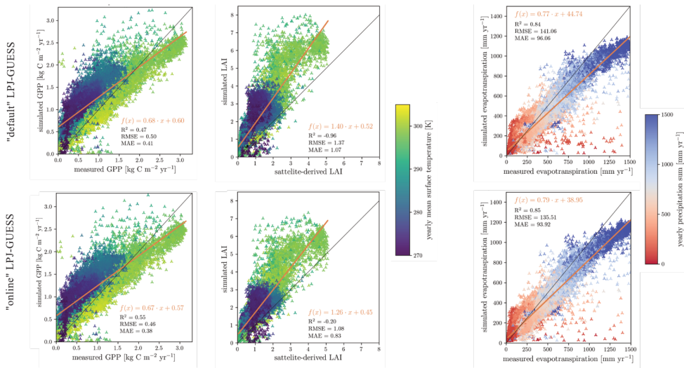
Figure 8: Left) Linear fit of simulated and measured GPP after FLUXCOM dataset (Tramontana et al., 2016). Middle) Linear fit of simulated and measured LAI after the AVHRR dataset (Fang et al., 2019). Right) Linear fit of simulated and measured evapotranspiration after the GLEAMv33a dataset (Miralles et al., 2011). All figures used model output between 1980-2014. Each marker shows the average of a grid cell over the 34-year timespan. The markers colour indicates the grid cell's yearly average near surface temperature and precipitation sum.
