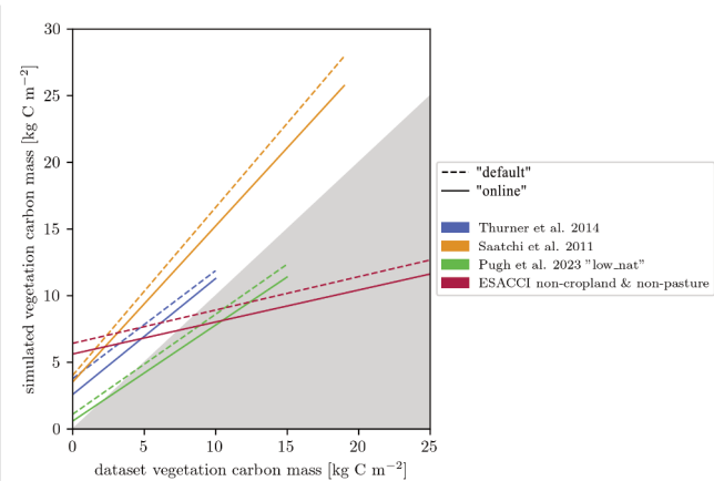
375 Figure 9: Linear fit of simulated and measured vegetation carbon mass for four datasets. The non-cropland & non-pasture dataset is based on the ESA aboveground biomass (Santoro and Cartus, 2023) and the ESA land cover datasets (ESA Land Cover Climate Change Initiative (Land_Cover_cci): Global Land Cover Maps, Version 2.0.7, 2024). AGB was converted into total vegetation carbon mass.
