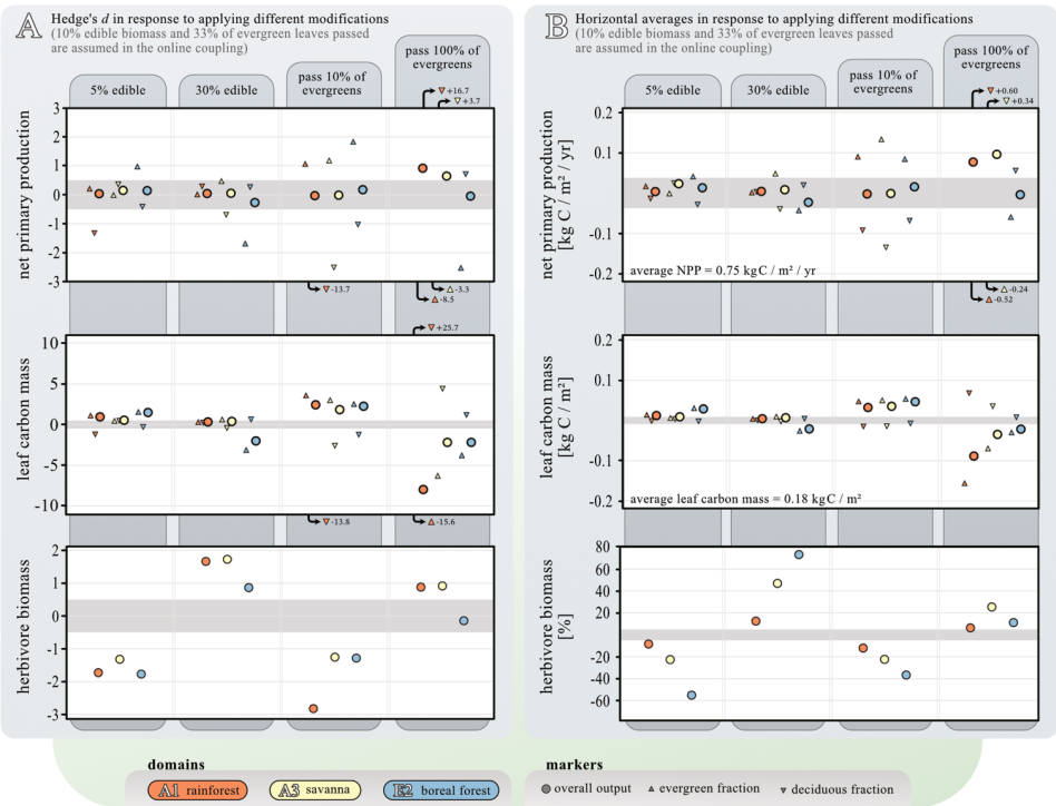
495 Figure 11: Sensitivity study of two model modifications: the amount of biomass edible for animals and evergreen vulnerability. The analysis was carried out for the simulation years 1900–1980. Both panels show data from three selected locations: orange – AF1 rainforest, yellow – AF3 savanna, and blue – EU2 boreal forest, each comprising 25 grid cells. Upward triangles indicate data of evergreen PFTs, while downward triangles indicate data of deciduous PFTs. Circles indicate data aggregated across all PFTs. 500 Panel A shows the general effect size (Hedge's d ). This data's 95% confidence intervals are similar within each metric: NPP ( \pm 0.3 SD), leaf carbon mass ( \pm 0.4 SD), and herbivore biomass ( \pm 0.2 SD). Small effect sizes are assumed for Hedge's d < 0.5 (indicated by gray background shading). Panel B shows changes in domain-wide averages in response to the same two modifications. To set absolute values into perspective, the average NPP and leaf carbon mass across all three model domains and ensembles is given. Average responses smaller than 5% are indicated by gray background shading.
