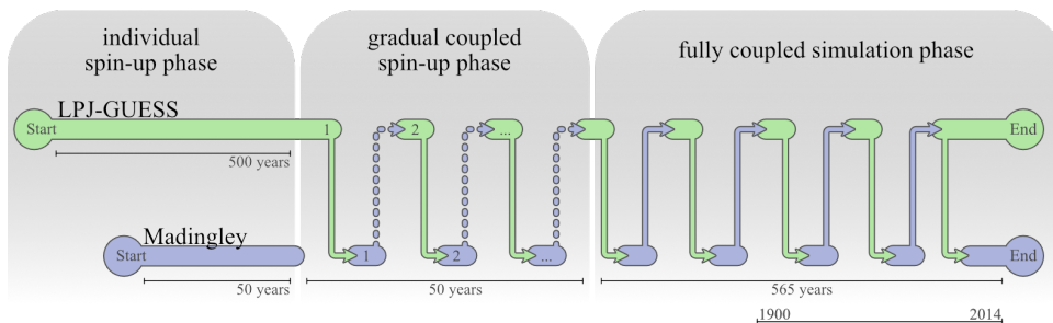
200 Figure 2: Runtime structure of the coupled simulations. File transfer is indicated by arrows occurring after each month. First, LPJ-GUESS completes a timestep and passes data to Madingley, then enters a waiting state. Madingley subsequently runs the same timestep using the received data and returns herbivory data to LPJ-GUESS. The number of data exchanges shown is illustrative and does not represent actual model runtime or performance.
