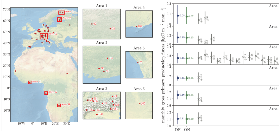
575 Figure 7: (Left) Distribution of FLUXNET eddy covariance measurement sites over the model domain with selected Areas and station numbers. (Right) Comparison between “default” LPJ-GUESS (DF), the “online” coupled simulation (ON) and the FLUXNET measurements with station number. The displayed GPP fluxes are monthly fluxes from the selected area which contains the FLUXNET sites. Simulated GPP are for the period 1994 to 2014. The time spans of the corresponding eddy flux data (within that same period is provided by the separate FLUXNET stations and can be found in Figure S4. Background map “Shaded Relief and Water large 3.2.0” by Natural Earth 1 (download under https://www.naturalearthdata.com/downloads/10m-natural-earth-1/10m-natural-earth-1-with-shaded-relief-and-water/ ). 580
