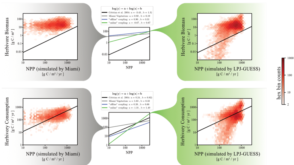
630 Figure 10: Power-law relationship between herbivore biomass and grid cell productivity, as well as herbivory consumptions and grid cell productivity. The red saturation of each hexagon represents the number of data points found in the model system that matches the NPP and the herbivore biomass (or herbivory consumption) of that hexagon's position in the grid. The left distributions show data from "default" Madingley (driven by the Miami model), while the right distributions show data from "online" Madingley. In the middle of the figure, power-law relationships are summarised for all three Madingley model versions. 635 The black line in each plot displays the power-law derived by Cebrian (2004).
