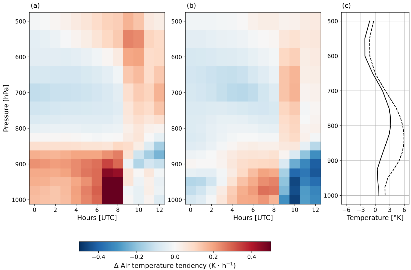
Figure 6. Mean differences (high-low BBA days) of the hourly tendency of air temperature ( \text{K} \cdot \text{h}^{-1} ) at each time step for 16 pressure levels in the AN (a) and in the CN (b) during the BBA season (2004–2018). (c) Vertical profiles of the mean differences (high-low BBA days) of air temperature (K) at 08:00 UTC for 16 pressure levels in the AN (solid line) and CN (dashed line).
