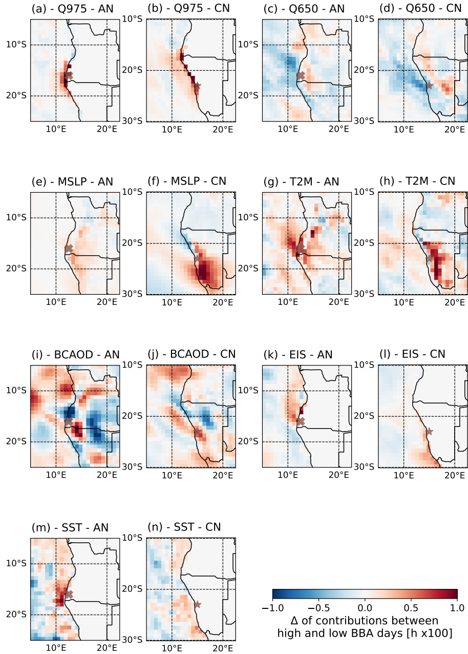
Figure 9. Ensemble mean differences (high-low BBA days) of spatial contributions (hours x100) for each predictor:( a, b ) specific humidity at 975 hPa with subsurface regions masked, ( c, d ) specific humidity at 650 hPa, ( e, f ) mean sea level pressure, ( g, h ) 2m temperature, ( i, j ) black carbon AOD, ( k, l ) estimated inversion strength, ( m, n ) sea surface temperature. In the AN ( a, c, e, g, i, k, m, o ) and the CN ( b, d, f, h, j, l, n, p ). The brown cross (resp. star) represents the center of the AN (resp. CN).
