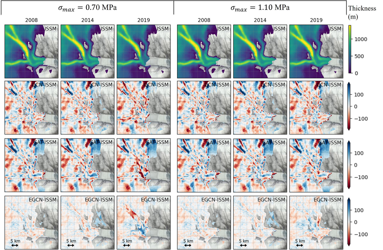
Figure 5. Maps of ISSM-simulated ice thickness and difference in ice thickness between GNN emulators and ISSM simulations (GCN, GAT, and EGCN from top to bottom) for 0.70 and 1.10 MPa test \sigma_{\max} values of set A.
