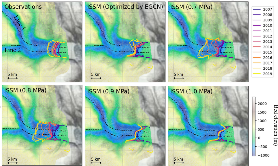
Figure 7. Annual movement of ice front observed by satellite imagery and modeled by ISSM with different \sigma_{\max} parameterizations: optimal \sigma_{\max} values from EGCN and constant \sigma_{\max} values (0.7, 0.8, 0.9, and 1.0 MPa).
