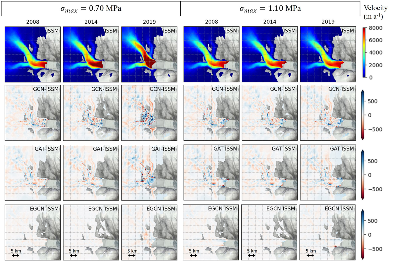
Figure 4. Maps of ISSM-simulated ice velocity and difference in ice velocity between GNN emulators and ISSM simulations (GCN, GAT, and EGCN from top to bottom) for 0.70 and 1.10 MPa test \sigma_{\max} values of set A.
