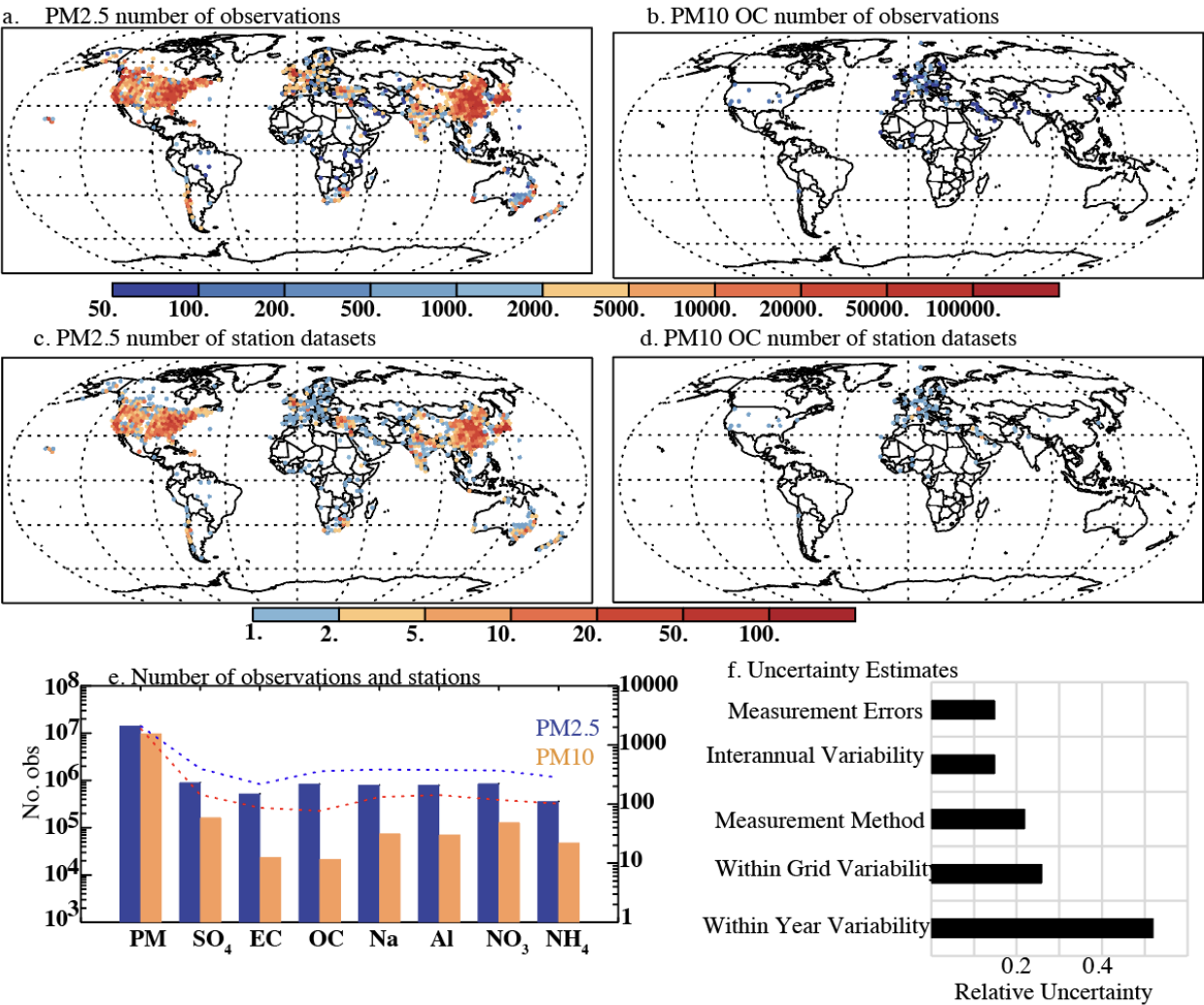
1587 Figure 1: Distribution of observations in the data base, showing the number of observations of PM 2.5 (a) and 1588 PM 10 organic carbon (OC) (b) (with the colors indicating different numbers using the top color bar), as well as 1589 the number of stations within each 2x2 grid locations for PM 2.5 (c) and PM 10 OC (d) (using the second color bar), 1590 showing that there is much more PM 2.5 or PM 10 data, in contrast to speciated data. e) The number of observations 1591 (bars) for total particulate matter (PM) or speciated data is summarized for the PM 2.5 (blue) and PM 10 (orange) 1592 fraction using the left-hand side y-axis. The number of stations included in the study is shown as a dotted line (e) 1593 and uses the right-hand size y-axis. f) Normalized (1 standard deviation over the mean) observational uncertainty 1594 for PM 2.5 from measurement errors, interannual variability, measurement method, within grid variability and
