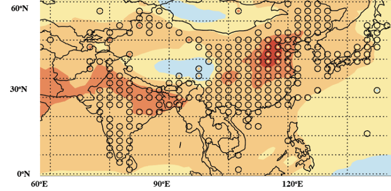
c. PM 2.5 ug/m 3
