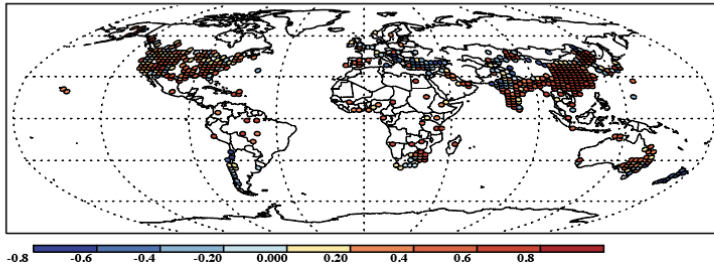
b. Seasonal Correlation PM10
