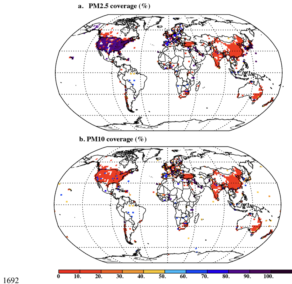
1693 Figure 10: Observational coverage (%) for gridded observations, showing within each grid box (2°x2°) the % of 1694 the constituents that are measured assuming that PM, SO 4 2- , BC, OM, Na, Al, NO 3 - , and NH 4 + are required to 1695 constrain the PM distribution for (a) PM 2.5 and (b) PM 10 .
