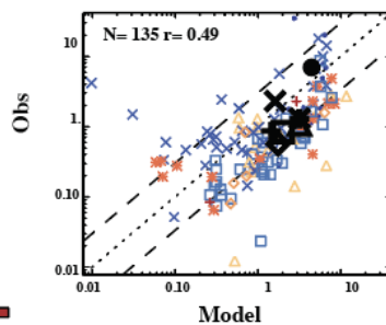
h. Na PM10 \mu\text{g}/\text{m}^3
