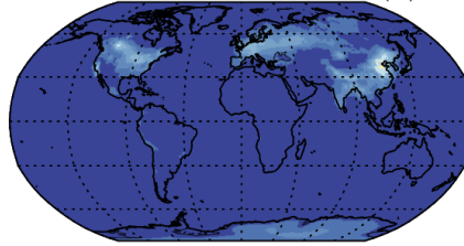
d. PM 10 concentration new sources (%)
