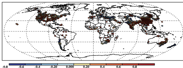
b. Seasonal Correlation PM10
