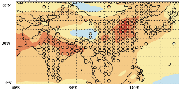
c. PM 2.5 ug/m 3
