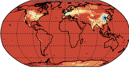
c. PM 10 concentration default sources (%)
