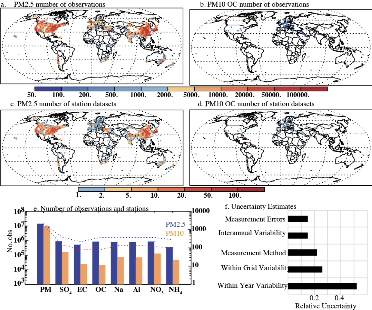
1582 Figure 1: Distribution of observations in the data base, showing the number of observations of PM 2.5 (a) and 1583 PM 10 organic carbon (OC) (b) (with the colors indicating different numbers using the top color bar), as well as 1584 the number of stations within each 2x2 grid locations for PM 2.5 (c) and PM 10 OC (d) (using the second color bar), 1585 showing that there is much more PM 2.5 or PM 10 data, in contrast to speciated data. e) The number of observations 1586 (bars) for total particulate matter (PM) or speciated data is summarized for the PM 2.5 (blue) and PM 10 (orange) 1587 fraction using the left-hand side y-axis. The number of stations included in the study is shown as a dotted line (e) 1588 and uses the right-hand size y-axis. f) Normalized (1 standard deviation over the mean) observational uncertainty 1589 for PM 2.5 from measurement errors, interannual variability, measurement method, within grid variability and
