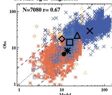
d. PM 2.5 ug/m 3 (ungridded)
