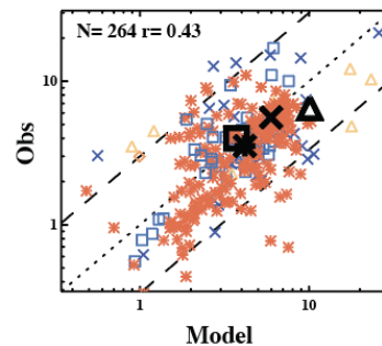
h. Na PM 2.5 \mu\text{g}/\text{m}^3
