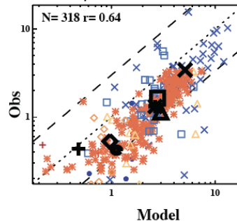
b. \text{SO}_4 PM 2.5 \mu\text{g}/\text{m}^3
