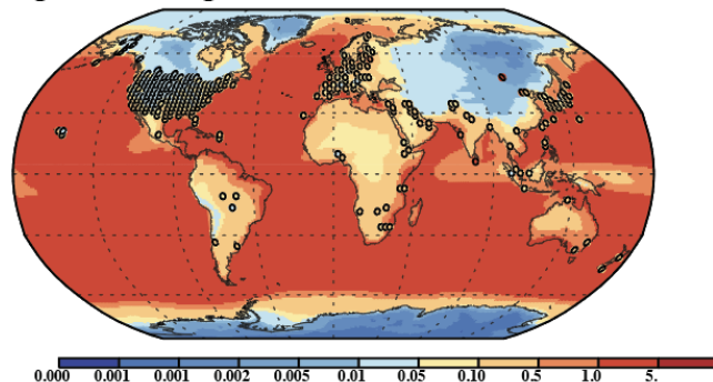
g. Na PM 2.5 \mu\text{g}/\text{m}^3
