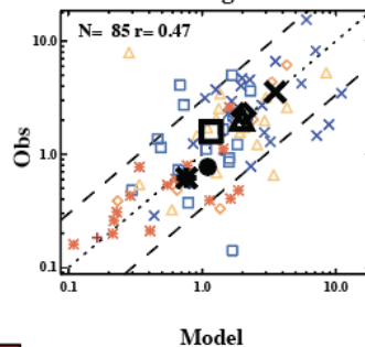
d. BC PM10 \mu\text{g}/\text{m}^3
