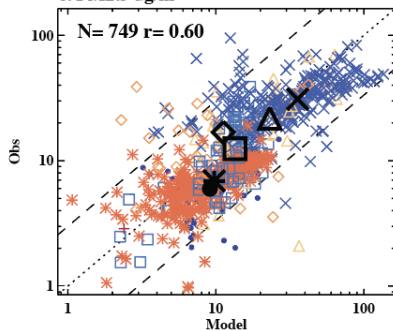
c. PM 2.5 ug/m 3
