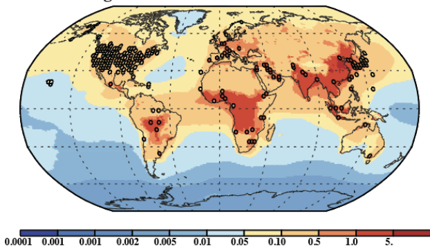
e. OM PM 2.5 \mu\text{g}/\text{m}^3
