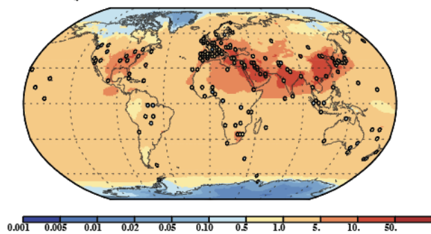
c. BC PM10 \mu\text{g}/\text{m}^3
