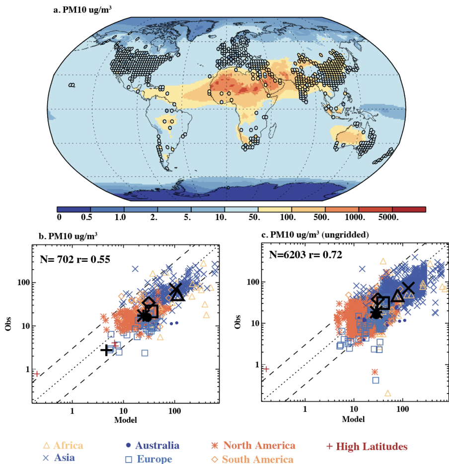
Figure 6: Model results and gridded observations for PM 10 in \mu\text{g}/\text{m}^3 spatially mapped globally (a). A comparison of the model (x-axis) to the observations (y-axis) is shown for the gridded data (b) and including all stations (c). In the scatter plots, the colors and symbols indicate the regions, the bold black symbols are the average across each region (indicated by the symbol), the dotted line is the 1:1 line and dashed lines are the factor of 3 uncertainty estimates. More statistics are shown in Table S7, and maps focused on different regions are shown in Fig. S10
