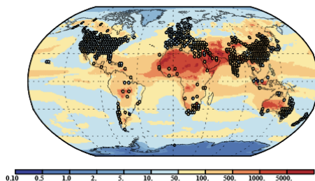
e. Seasonal Std. Dev. PM10
