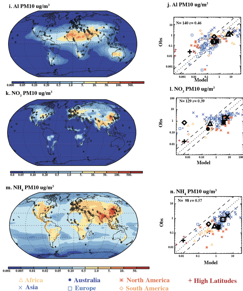
Figure 7: Model results and gridded observations for different types of \text{PM}_{10} in \mu\text{g}/\text{m}^3 spatially mapped globally where the model is plotted as the background and the observations are circles with the colors indicating the amount \text{PM}_{10} using the same scale for (a) \text{SO}_4^{+2} , (c) BC (black carbon), (e) OM (organic material=1.8 times organic carbon (OC)), (g) Na, (i) Al, (k) \text{NO}_3^- , (m) \text{NH}_4^+ . A scatter plot comparison of the model (x-axis) to the observations (y-axis) is shown for the gridded observational data for (b) \text{SO}_4^{+2} , (d) BC (f) OM, (h) Na, (j) Al, (l) \text{NO}_3^- , (n) \text{NH}_4^+ . In the scatter plots, the colors and symbols indicate the regions, the bold black symbols are the average across each region (indicated by the symbol), the dotted line is the 1:1 line and the dashed lines are the
