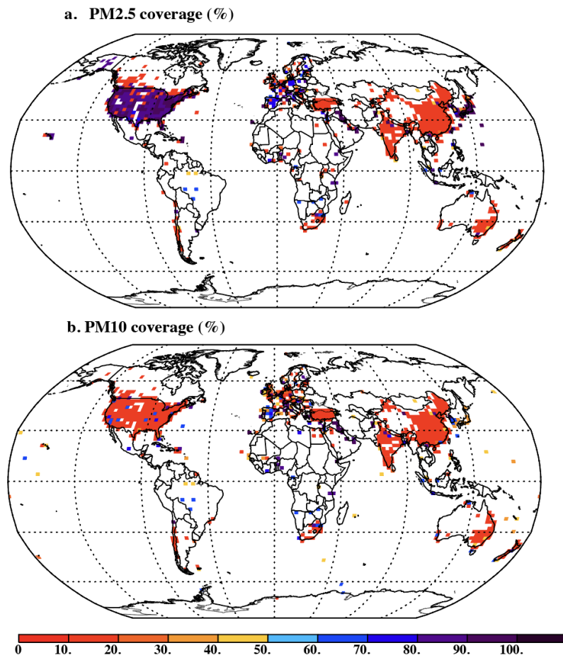
1687 1688 Figure 10: Observational coverage (%) for gridded observations, showing within each grid box (2°x2°) the % of 1689 the constituents that are measured assuming that PM, SO 4 2- , BC, OM, Na, Al, NO 3 - , and NH 4 + are required to 1690 constrain the PM distribution for (a) PM 2.5 and (b) PM 10 .
