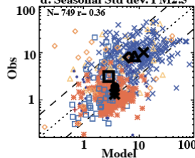
d. Seasonal Std dev. PM2.5
