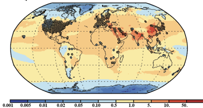
c. BC PM 2.5 \mu\text{g}/\text{m}^3
