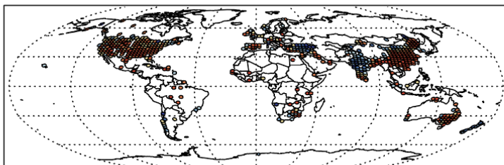
c. Seasonal Std. Dev. PM2.5
