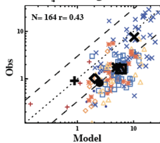
b. \text{SO}_4 PM10 \mu\text{g}/\text{m}^3
