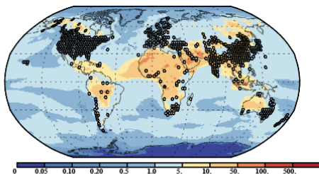
e. Seasonal Std. Dev. PM10
