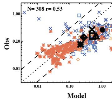
h. Na PM 2.5 \mu\text{g}/\text{m}^3
