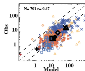
f. Seasonal Std. Dev. PM10
