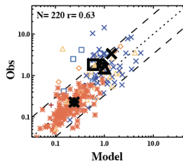
d. BC PM 2.5 \mu\text{g}/\text{m}^3
