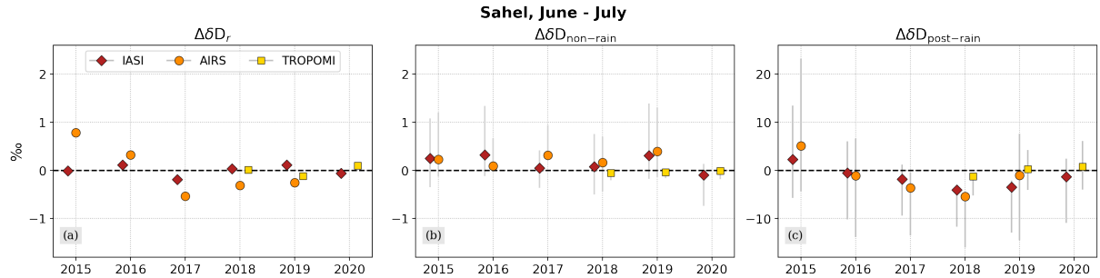
Figure 11. Results from the decomposition analysis to characterise the impact of the anomalies in rain fraction (a), non-rain events (b) and post-rain events (c) on the overall \delta\text{D} anomalies for IASI, AIRS and TROPOMI for the respectively available years. The scatters represent the mean values of the respective anomaly contributions and the grey bars denote the 1\sigma spread around the mean (only plotted for non-rain and post-rain). The ranges of the y-axes have been individually selected with respect to the data variability per sub-figure. A detailed description of the decomposition method is given in Section 2.2.
