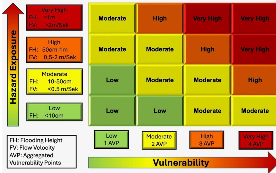
Figure 1: Systematic framework matrix for determining the flood risk that a sensitive infrastructure is facing (own figure).
