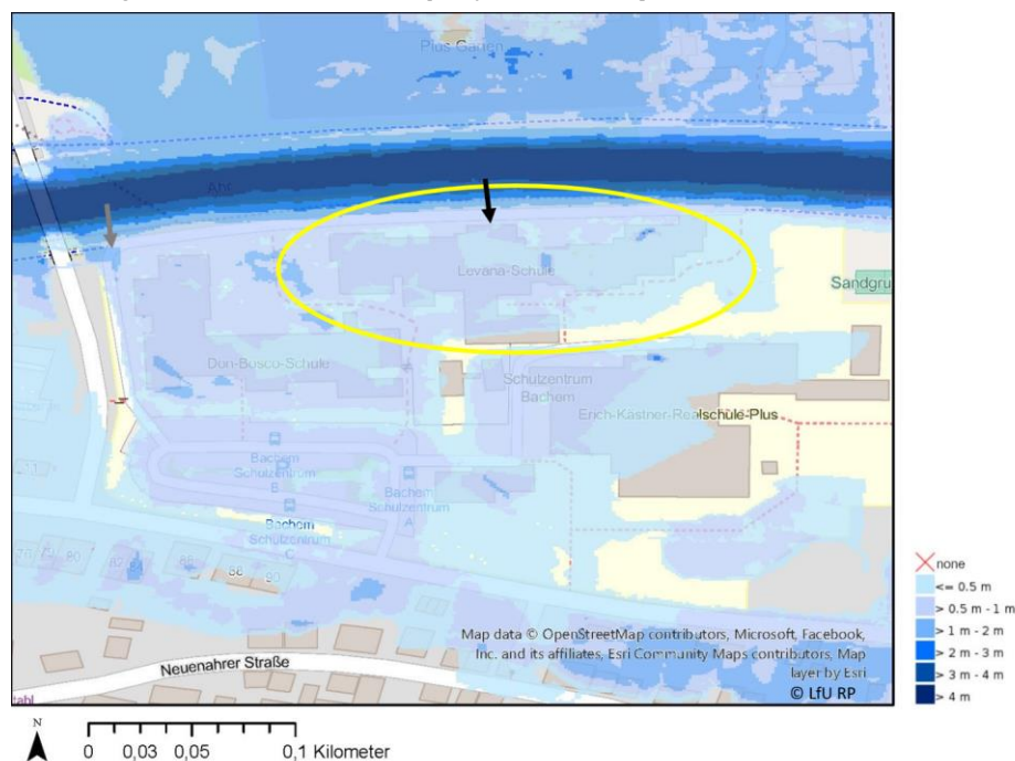
Figure 3: Depiction of the HQ-100 floodplains, revised by the State Office for the Environment Rhineland-Palatinate ( Landesamt für Umwelt Rheinland-Pfalz (LfU RP) ) after the 2021 flood, in the vicinity of the Levana School ( Hochwassergefahrenkarte Rheinland-Pfalz, © LfU, https://wasserportal.rlp-umwelt.de/kartendienste ).
