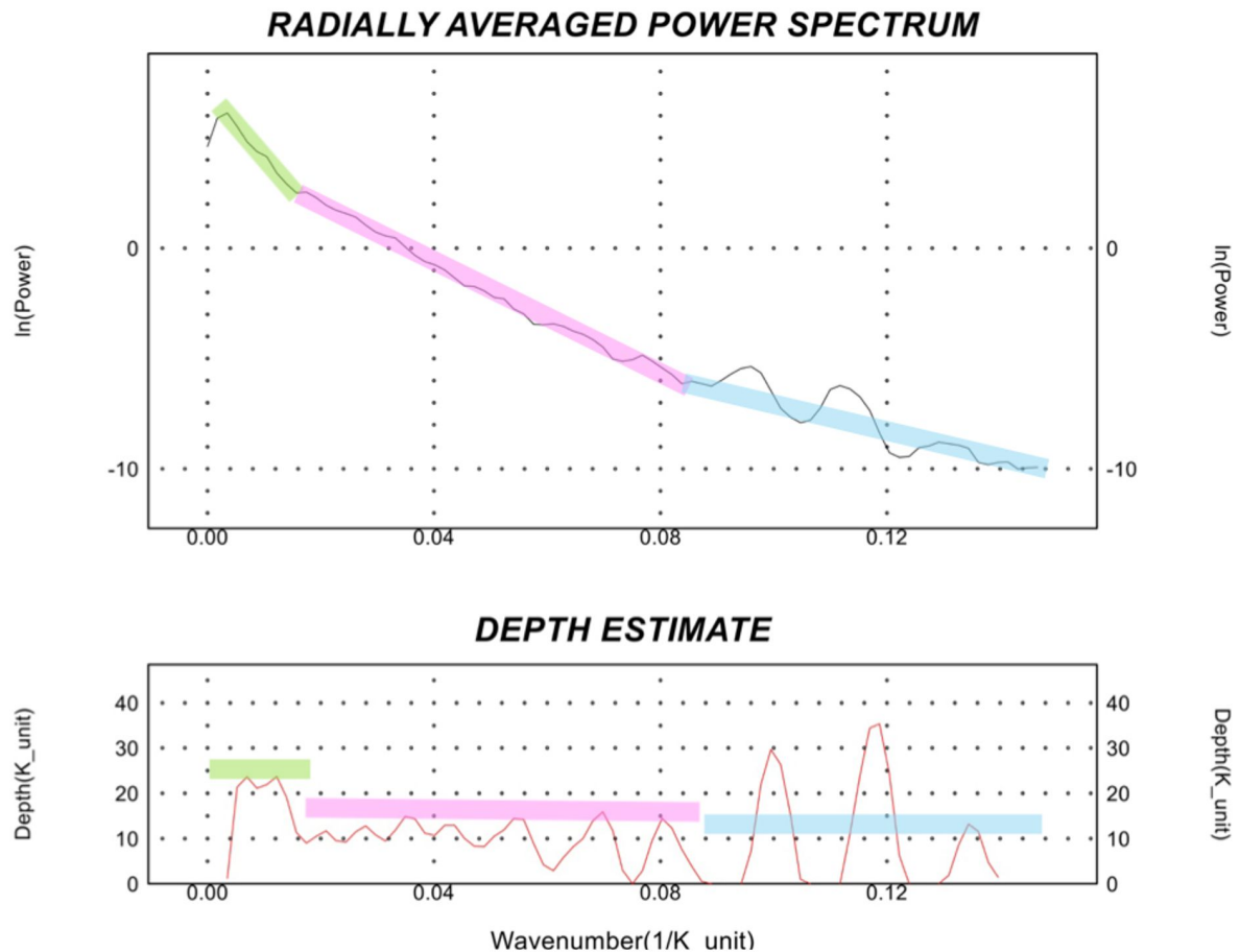
Fig.6. Radially averaged power spectrum of the RTP magnetic field. The wavelength range spans from 7.14 to 125 1000 km. The maximum depth values reach 35 km.
