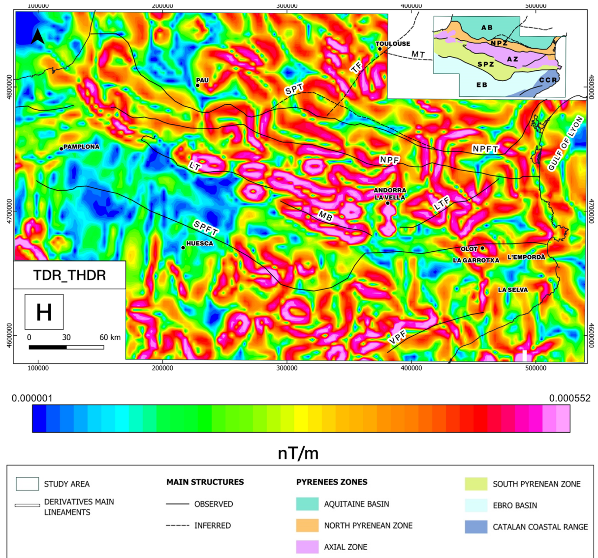
275 Fig.4. (A) Vertical derivative map (VDR_Z). (B) Horizontal derivative in X map (HDR_X). (C) Horizontal derivative 280 in Y map (HDR_Y). (D) Horizontal derivative in N110°E map (HDR_110). (E) Horizontal derivative in N200°E map (HDR_200). (F) Analytic Signal map (AS). (G) Tilt derivative map (TDR). (H) Horizontal derivative of the tilt derivative map (TDR_THDR). In the upper right corner, a simplified version of Fig.1. In addition, the main lineaments of each derivative and main structures of the study area are also represented. The main Pyrenean zones are differentiated by diverse texture patterns. MT: Mazamet Thrust, TF: Toulouse Fault, SPT: Sub-Pyrenean Thrust, NPFT: North Pyrenean Frontal Thrust, NPF: North Pyrenean Fault, LTF: La tet Fault, MB: Morreres Back Thrust, LT: Larra Thrust, SPFT: South Pyrenean Frontal Thrust, VPF: Valles-Penedes Fault. UTM coordinates in m, Zone 31N, ETRS89 datum.
