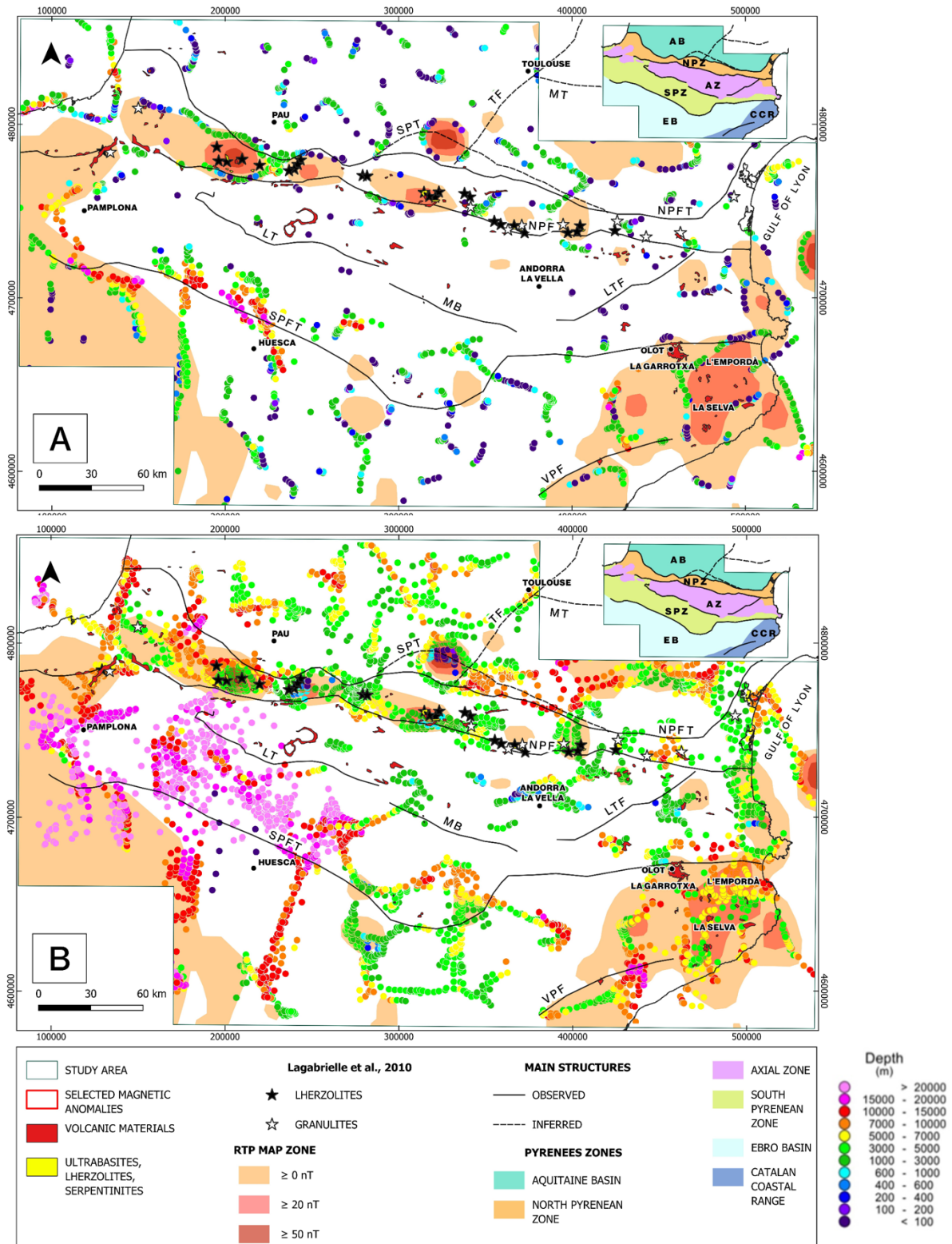
Fig.5. RTP above 0 nT map in addition to (A) Euler solution for SI:0 WS:5; (B) Euler solution for SI:1 WS:10. In the upper right corner, a simplified version of Fig.1. Main structures and Pyrenean zones differentiated by diverse texture patterns are also represented. MT: Mazamet Thrust, TF: Toulouse Fault, SPT: Sub-Pyrenean Thrust, NPFT: North Pyrenean Frontal Thrust, NPF: North Pyrenean Fault, LTF: La tet Fault, MB: Morreres Back Thrust, LT: Larra Thrust, SPFT: South Pyrenean Frontal Thrust, VPF: Valles-Penedes Fault. Volcanic materials, Iherzolites, Lagabrielle et al., (2009) Iherzolite and granulite mapping, Gulf of Lyon, La Selva, L'Empordà, La Garrotxa and Olot are highlighted. UTM coordinates in m, Zone 31N, ETRS89 datum.
