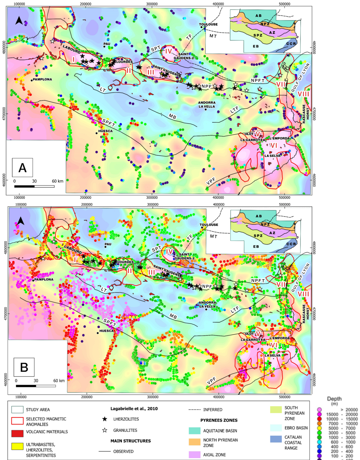
395 Fig.8. Reduced to the pole magnetic map of the study area with the (A) Euler solution for SI:0 WS:5; (B) Euler solution for SI:1 WS:10 on top. In the upper right corner, a simplified version of Fig.1. Main structures and Pyrenean zones differentiated by diverse texture patterns are also represented. MT: Mazamet Thrust, TF: Toulouse Fault, SPT: Sub-Pyrenean Thrust, NPFT: North Pyrenean Frontal Thrust, NPF: North Pyrenean Fault, LTF: La tet Fault, MB: Morrerres Back Thrust, LT: Larra Thrust, SPFT: South Pyrenean Frontal Thrust, VPF: Valles-Penedes Fault. Volcanic materials, Iherzolites, Lagabrielle et al., (2009) Iherzolite and granulite mapping are displyed. I: Labourd, II: Lourdes, III: Saint Gaudens, IV: Saint Gaudens-2, V: Olot, VI: L'Emporda-La Selva, VII: East Coast, VIII: Rascasse Horst. 400
