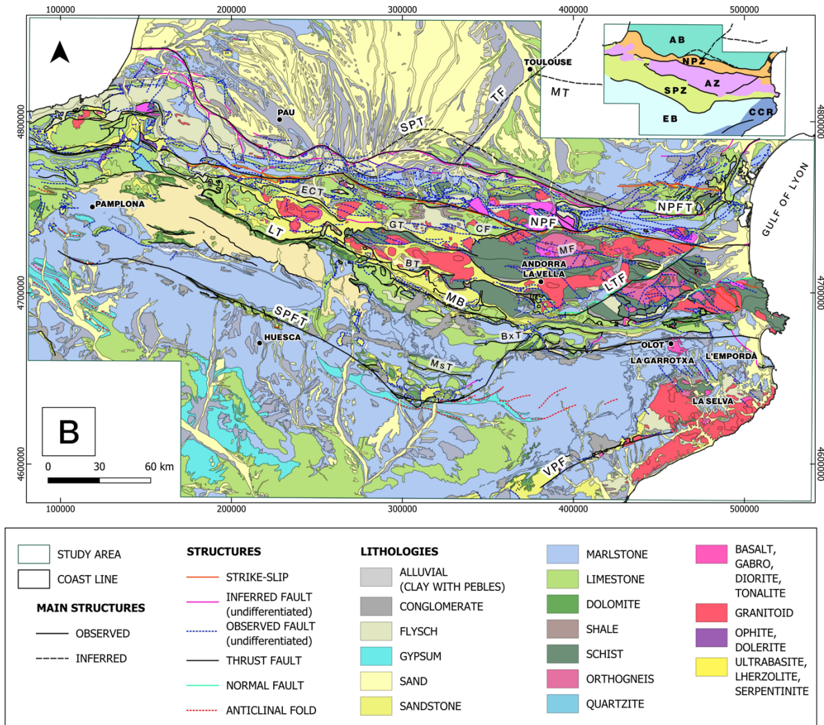
150 Fig.2. (A) Chronological and structural map (Modified from BRGM-IGME, 2009) (B) Lithological and structural (Modified from BRGM-IGME, 2009) of the Pyrenees study area. In the upper right corner, a simplified version of Fig.1. NPFT: North Pyrenean Frontal Thrust, NPF: North Pyrenean Fault, ECT: Eaux-Chaudes Thrust, GT: Gavarnie Thrust, CF: Couflens Fault, MF: Merens Fault, BT: Bono thrust, BxT: Boixols Thrust, MsT: Montsec Thrust, SMT: Sierra Marginales Thrust, LT: Larra Thrust, MB: Morreres Back Thrust, LTF: La Tet Fault, SPT: Sub-Pyrenean Thrust, MT: Mazamet Thrust, TF: Toulouse Fault, SPFT: South Pyrenean Frontal Thrust, VPF: Valles-Penedes Fault. 155 UTM coordinates in m, Zone 31N, ETRS89 datum.
