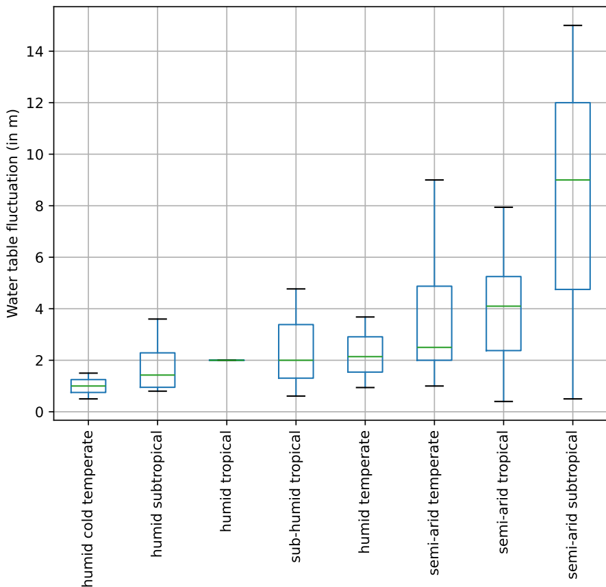
Figure 5. Estimates of water table fluctuation range (WFR) as a function of climatic conditions in modern systems. In this box-plot representation, the green line represents the mean value, the blue box encompasses values from the lower quartile to the upper quartile, while the black whiskers end at the lowest and highest values of the dataset.
