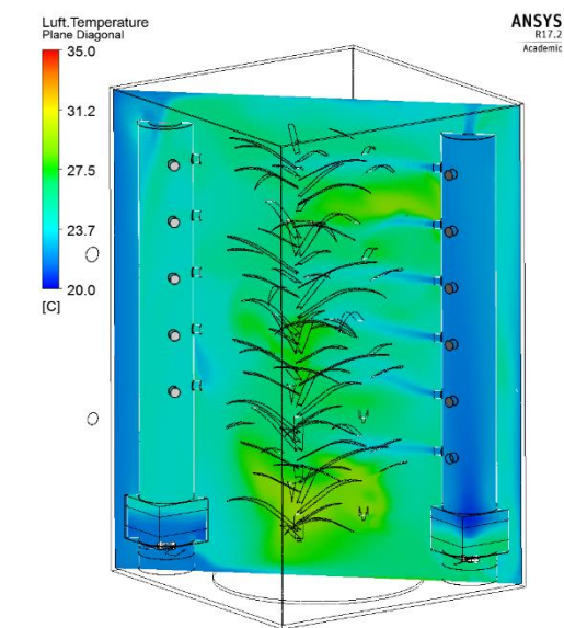
Figure 9: Temperature distribution within the plant chamber for the third and then actually realized cooling concept.
