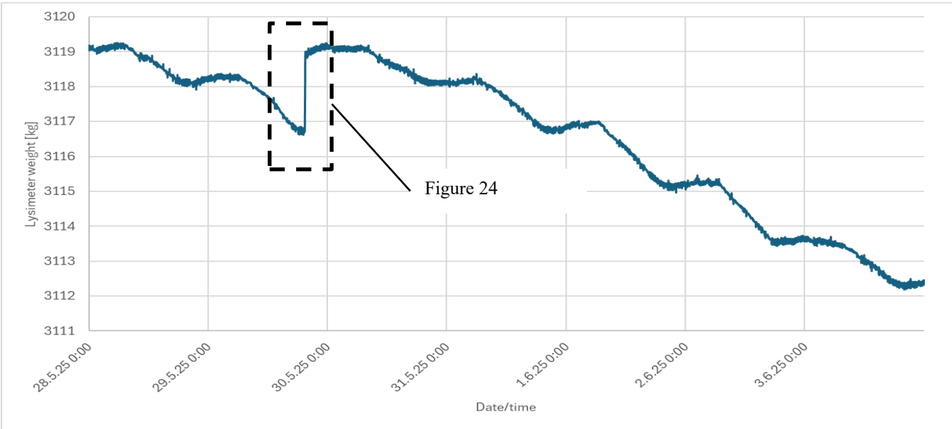
Figure 23: Lysimeter weight over the 7-day experiment period.
