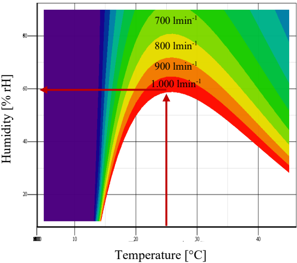
405 Figure 10: Required supply air volume flow to keep the humidity constant depending on the plant chamber temperature.
