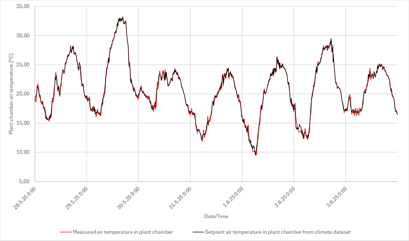
Figure 19: Temperature curve of the air temperature in the plant chamber over a 7-day period.
