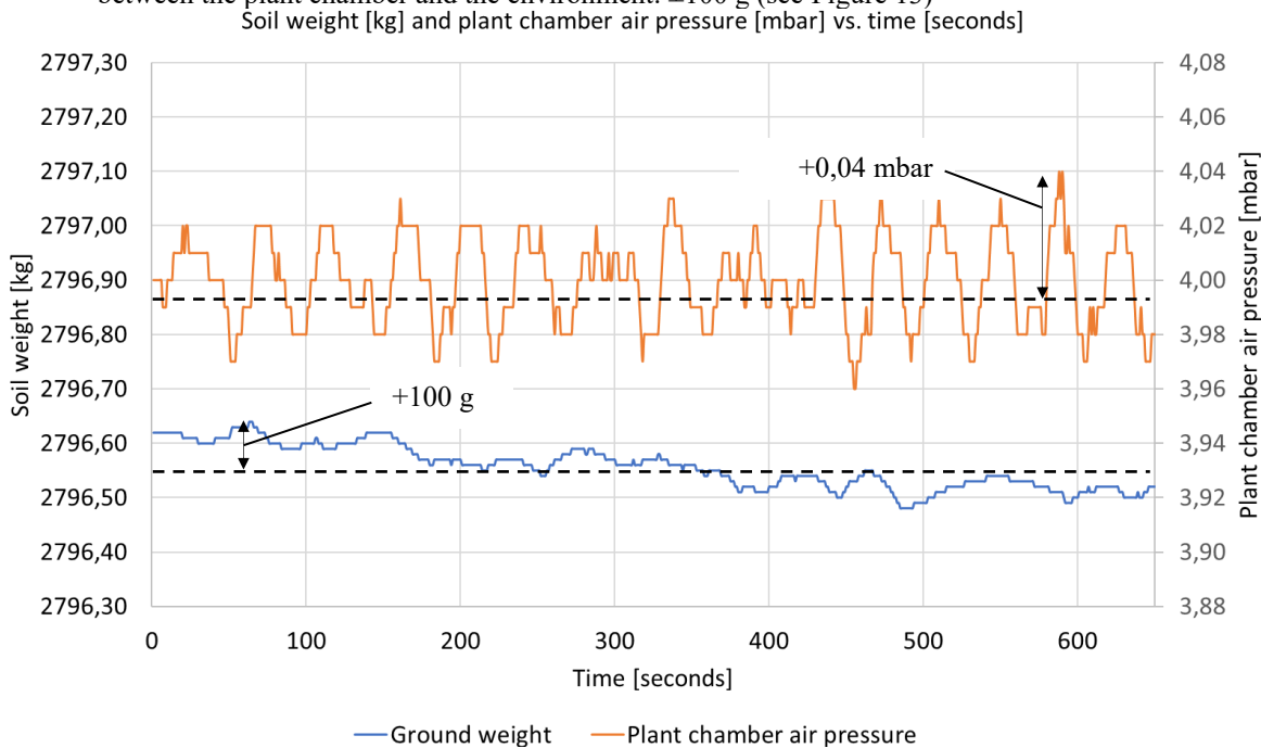
Figure 13: Lysimeter weight and air pressure inside the plant chamber.
