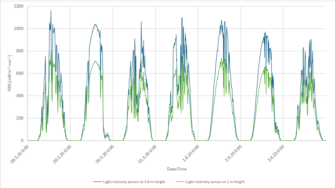
Figure 17: Intensity of photosynthetically active radiation (PAR) over the 7-day experimental period, measured at two different heights in the plant chamber (1 m and 1.6 m above the soil surface).
