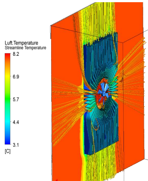
Figure 8: Second concept: heat sink in the side wall of the plant chamber.
