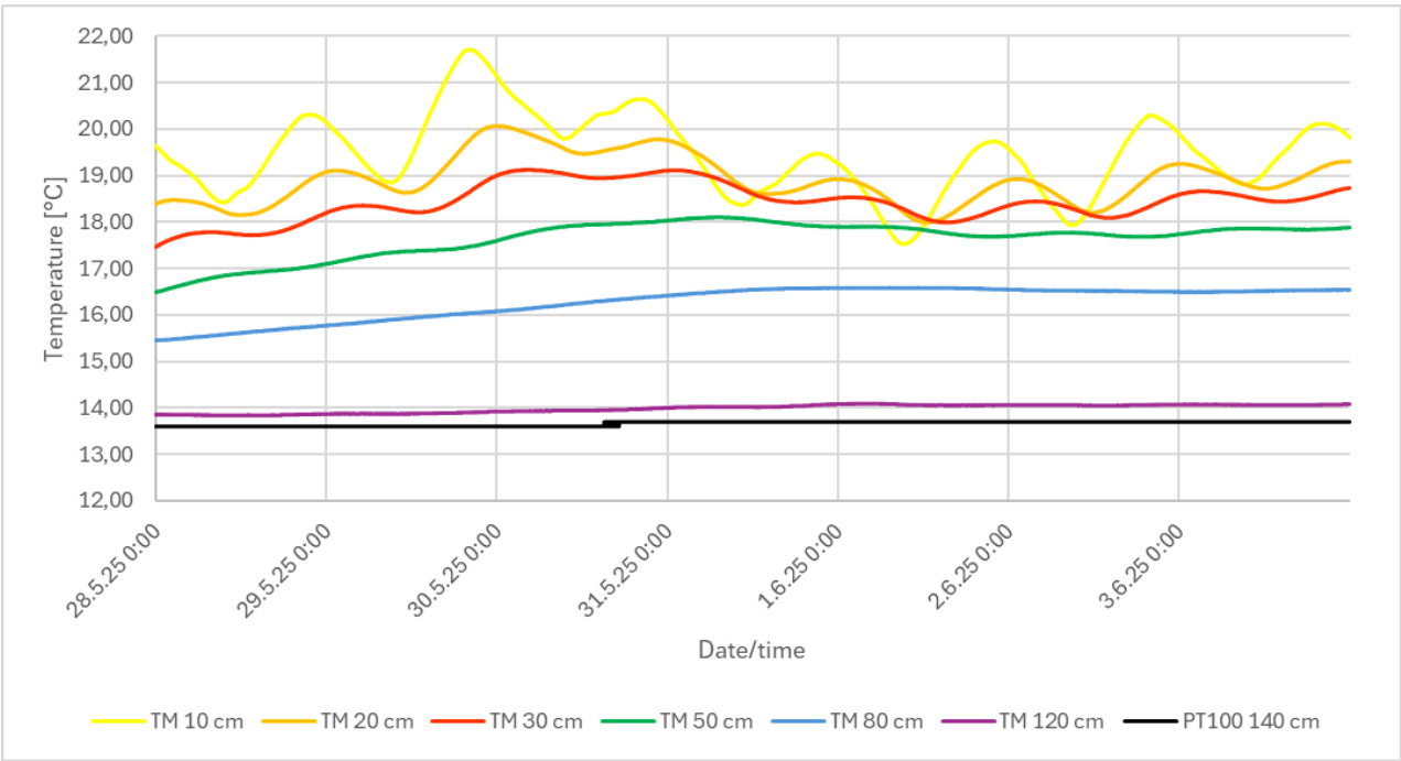
740 Figure 25: Soil temperature at different depths over the 7-day experimental period.
