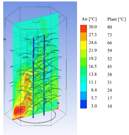
Figure 75: Result of CFD simulation.
