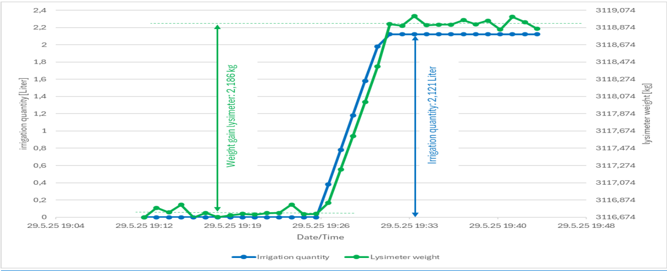
780 Figure 24: Comparison of the weight increase of the lysimeter at the time of irrigation the measured amount of water applied.
