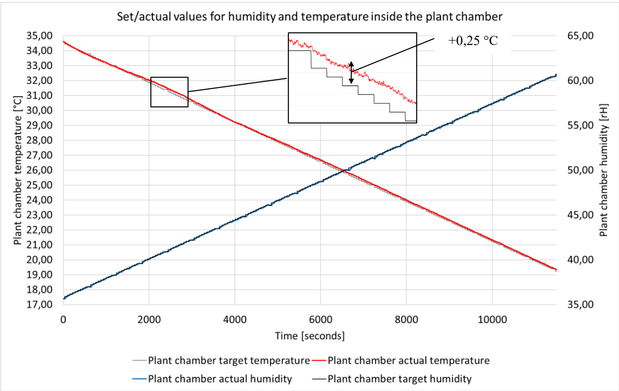
280 Figure 64: Measured temperature and humidity curve inside the plant chamber.
