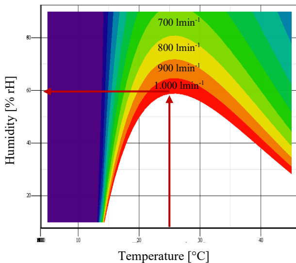
Figure 8 Figure 10 : Required supply air volume flow to keep the humidity constant depending on the plant chamber temperature.
