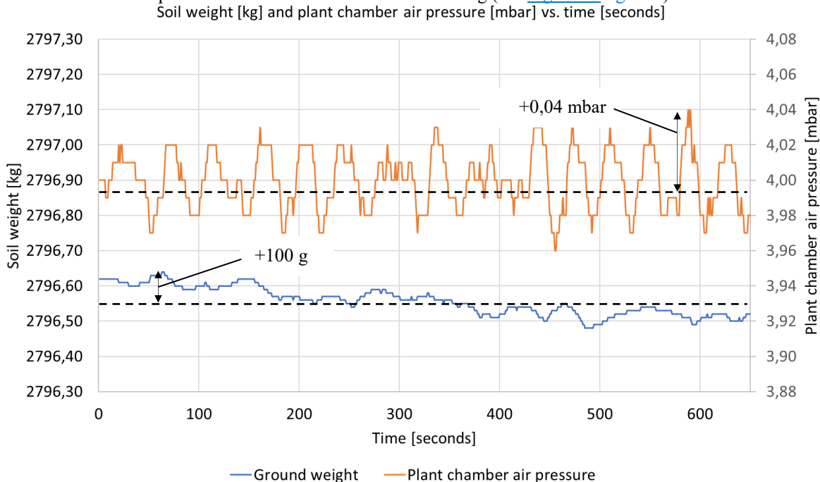
535 Figure 139: Lysimeter weight and air pressure inside the plant chamber.
