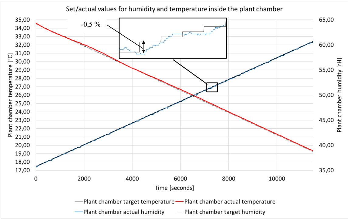
Figure 9 Figure 11 : Control accuracy of the plant chamber humidity.
