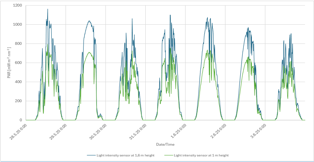
705 Figure 17: Intensity of photosynthetically active radiation (PAR) over the 7-day experimental period, measured at two different heights in the plant chamber (1 m and 1.6 m above the soil surface).
