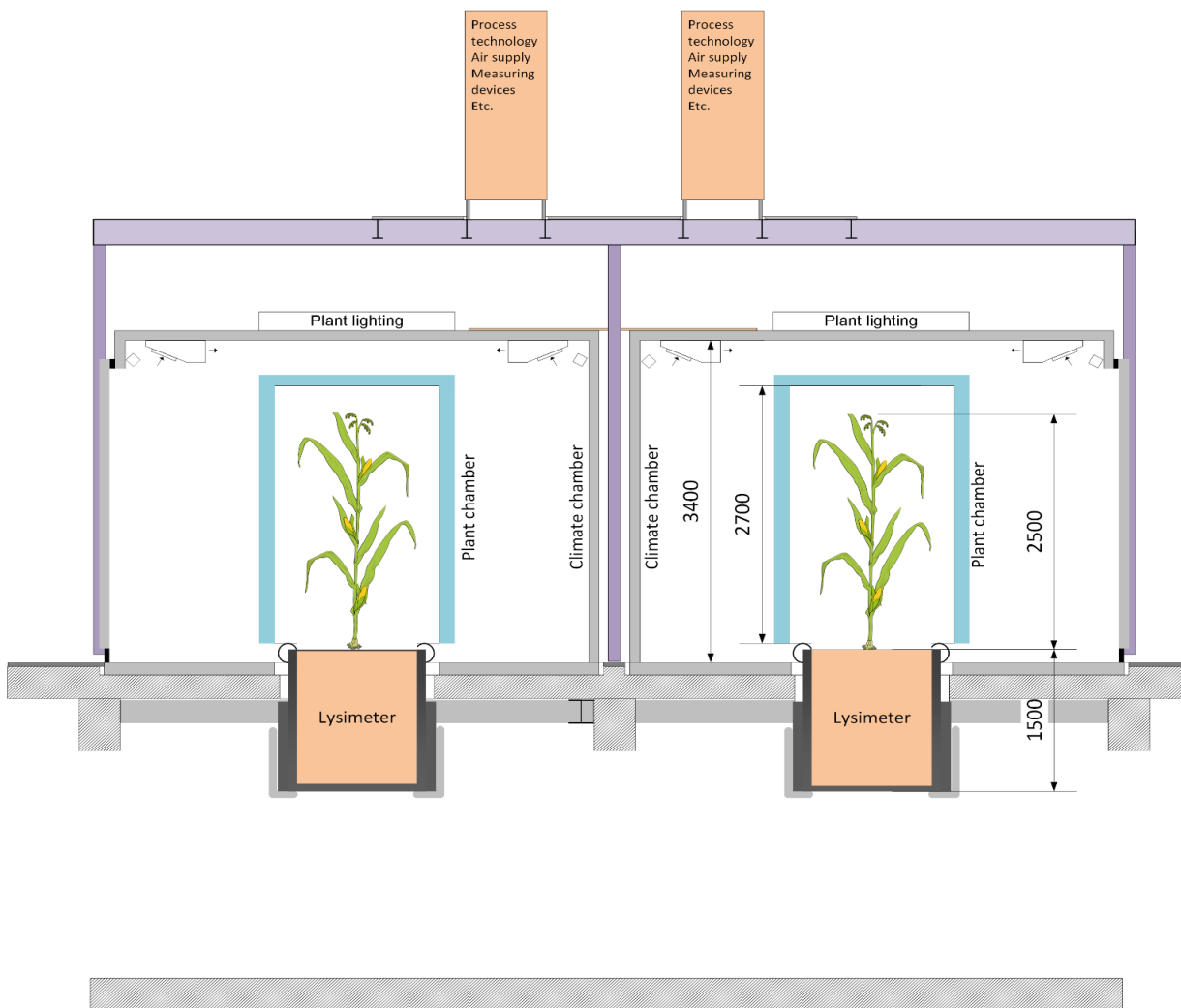
Figure 3: Schematic Cross-sectional view (A-A in Figure 2) of the experimental research infrastructure AgraSim.
