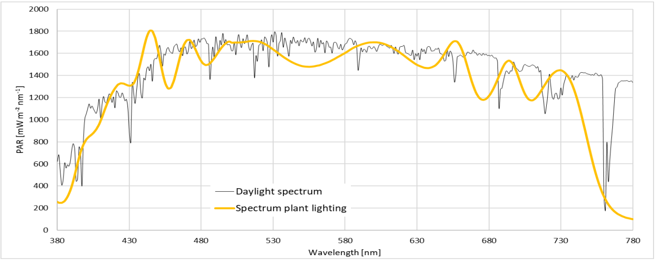
Figure 18: Comparison of the light spectrum of the plant lighting and the measured daylight spectrum.
