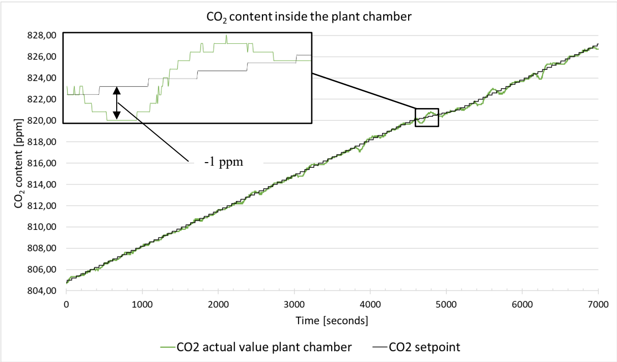
Figure 128: Target/actual comparison of CO 2 control within the plant chamber.
