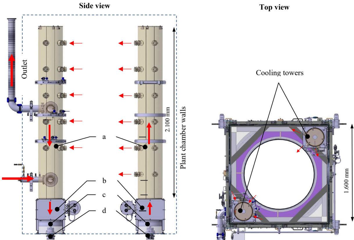
Figure 53: Cooling tower inside the plant chamber.
