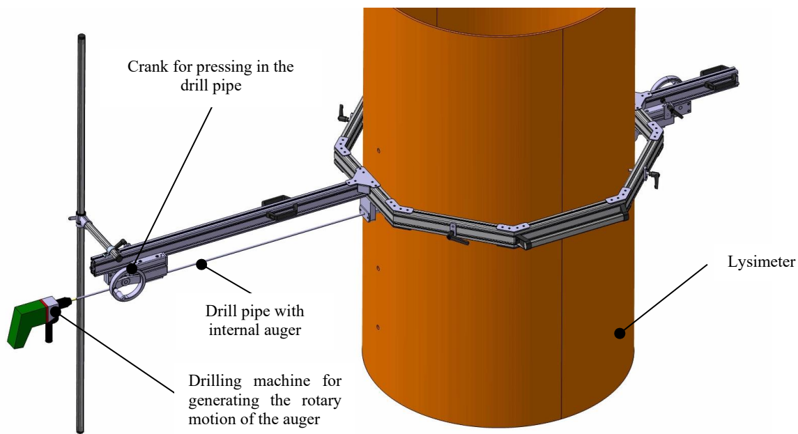
Figure 1544: Drilling rig to create the boreholes for the microporous hoses and to pull the microporous hoses into the soil.
