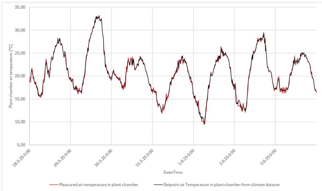
Figure 19: Temperature curve of the air temperature in the plant chamber over a 7-day period.
