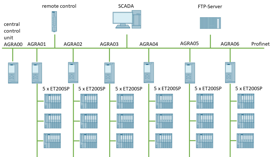
Figure 2643: Setup of the network for the entire AgraSim system.
