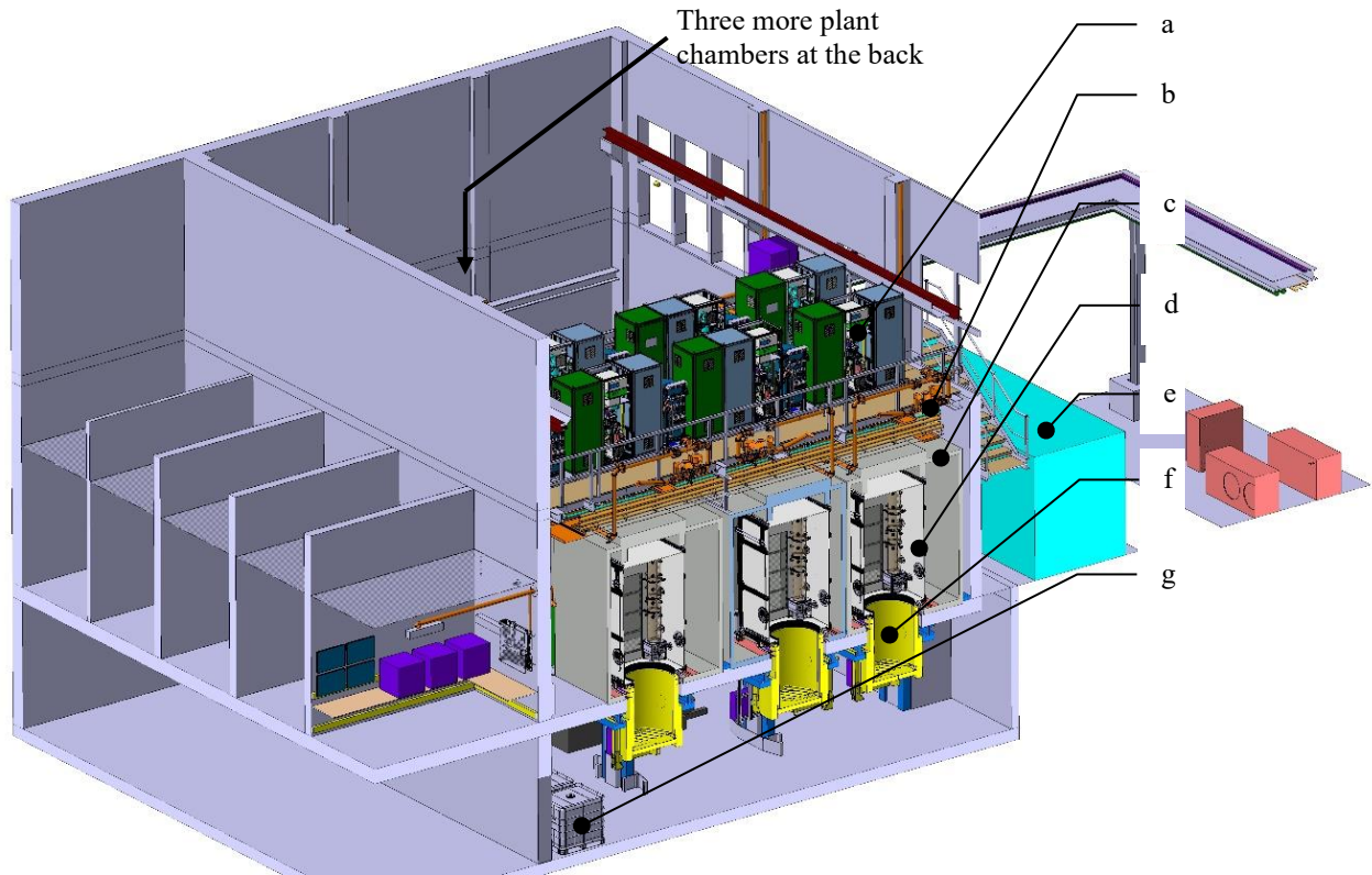
Figure 1: Setup of the experimental research infrastructure AgraSim.
