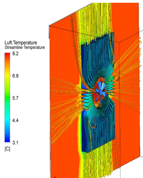
Figure 86: Second concept: heat sink in the side wall of the plant chamber.
