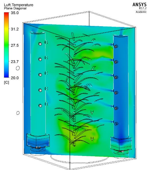
Figure 27: Temperature distribution within the plant chamber for the third and then actually realized cooling concept.
