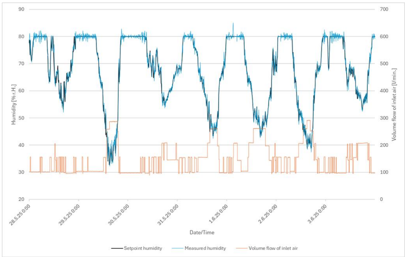
Figure 20: Relative humidity and air flow in the plant chamber over a 7-day period.
