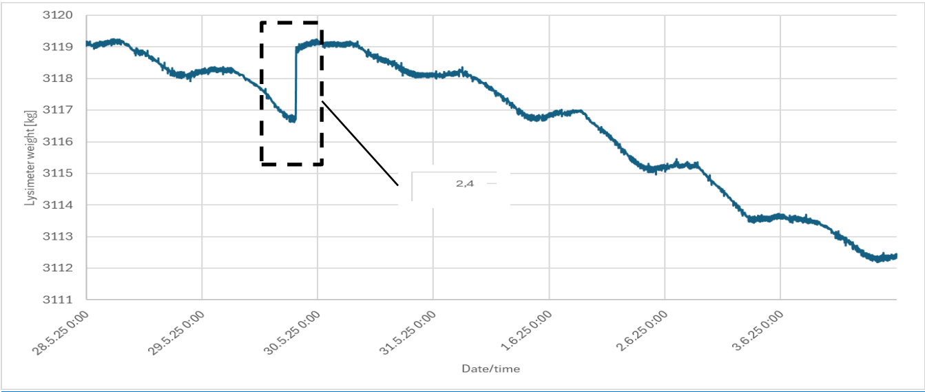
Figure 23: Lysimeter weight over the 7-day experiment period.
