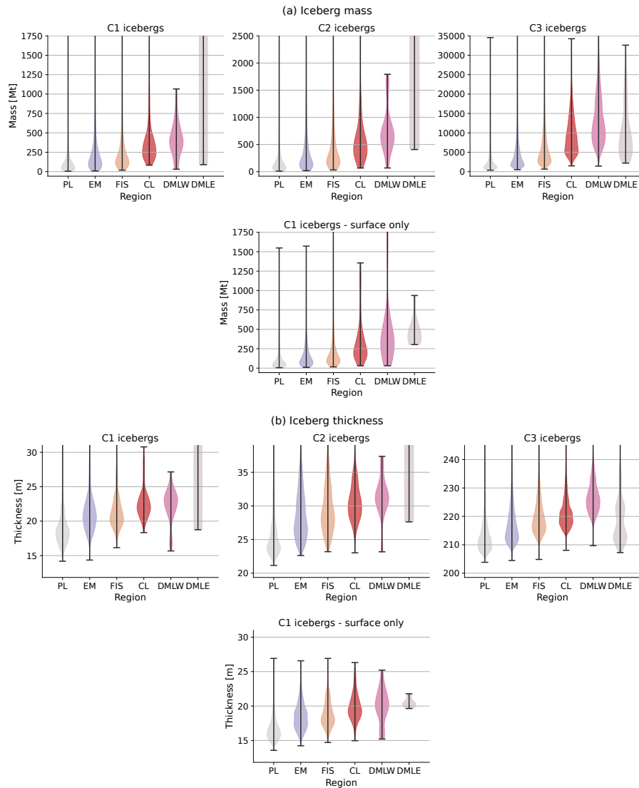
Figure 6. Visualisation (violin plot) of the distribution-mass and thickness distributions obtained during-with backward simulations for the (a) minimum iceberg mass and (b) minimum iceberg thickness in each coastal region (Fig. 1) where PL = Palmer Land, EM = Ellsworth Mountains, FIS = Filchner Ice Shelf, CL = Coats Land, and DML = Dronning Maud Land (W = west, E = east). Top rows: results of the main backward simulations ran for iceberg size classes C1, C2 and C3. Bottom rows: results of the sensitivity simulation ran for size class C1 when using only surface fields. The number of data points per region are given in Table B1 (Appendix B) and the full range of possible values is shown in Figure C1 (Appendix C).
