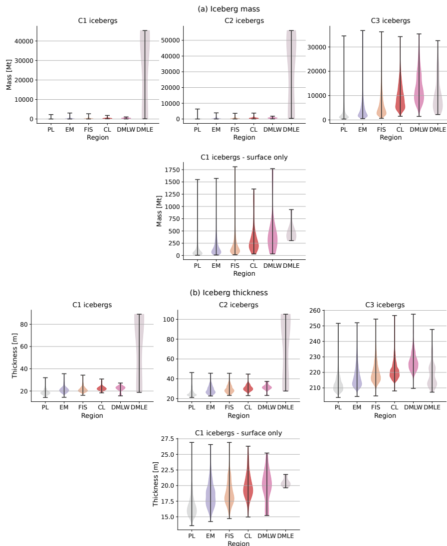
Figure C1. Visualisation (violin plot) of the complete distribution-mass and thickness distributions obtained during-with backward simulations for the (a) minimum iceberg mass and (b) minimum iceberg thickness in each coastal region (Fig. 1), where PL = Palmer Land, EM = Ellsworth Mountains, FIS = Filchner Ice Shelf, CL = Coats Land, and DML = Dronning Maud Land (W = west, E = east). Top rows: results of the main backward simulations ran for size classes C1, C2 and C3. Bottom rows: results of the sensitivity simulation ran for size class C1 when using only surface fields. See Figure 6 for more details in the lower range.
