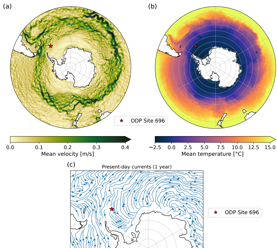
Figure D1. Regional time-mean (one year) ocean properties from the MOi hydrodynamics model (Gasparin et al., 2018) for the (a) velocity in the surface layer, (b) temperature at the surface (~ 0-200 m), and (c) ocean streamlines.
