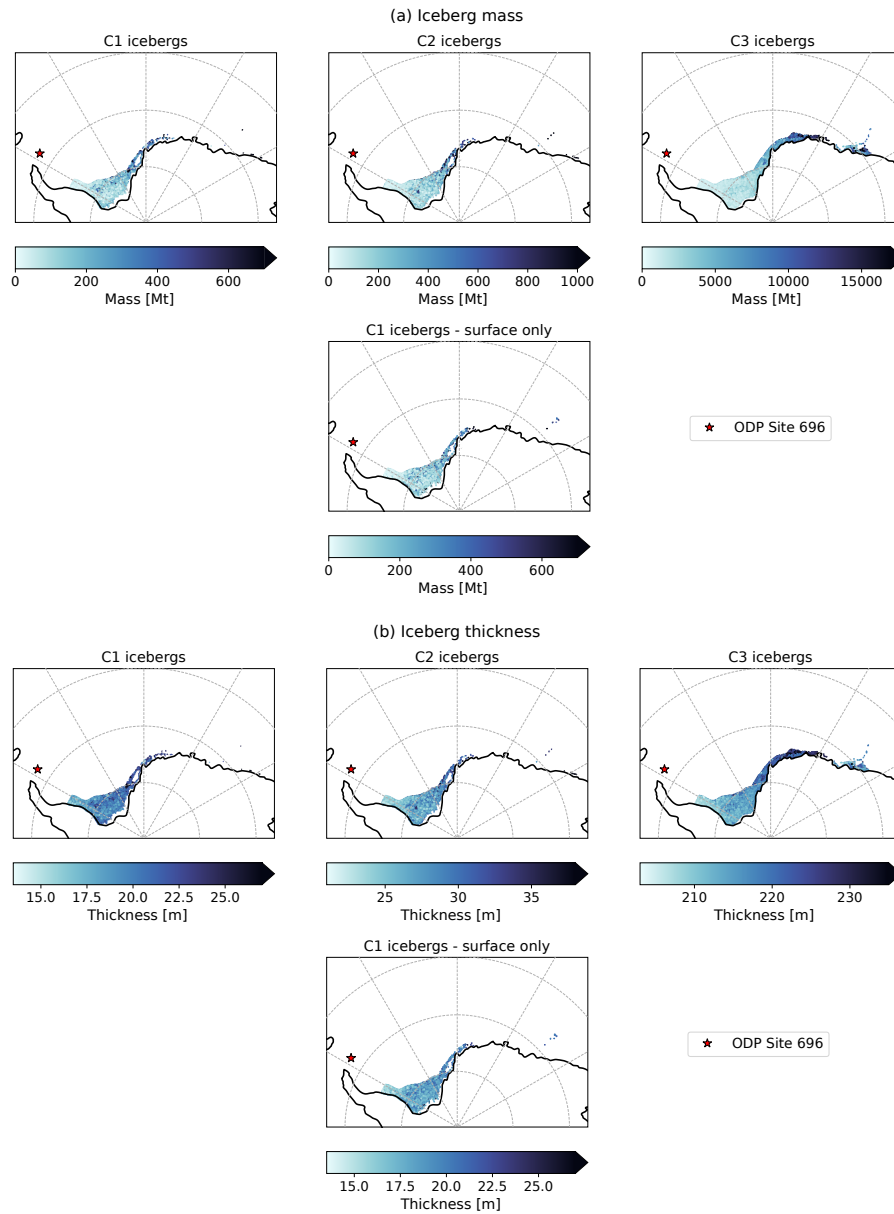
Figure 5. Spatial distribution-mass and thickness distributions obtained during-with backward simulations for (a) iceberg mass and (b) iceberg thickness within the defined coastal region of the Southern Weddell Sea based on Carter et al. (2017) (Fig. 1). Top rows: results of the main backward simulations ran for iceberg size classes C1, C2 and C3. Bottom rows: results of the sensitivity simulation for iceberg size class C1 using only surface fields. The total number of datapoints per simulation are given in Table B1 (Appendix B). Note that the marker of ODP Site 696 is roughly a quarter of the size of the SOM.
