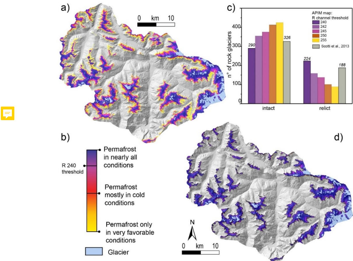
Figure 3. Likely extent of permafrost in the study area. a) original Alpine Permafrost Index Map (APIM; Boeckli et al., 2012); b) likelihood classes of permafrost occurrence based on the APIM RGB colour code; c) frequency of periglacial landforms with or without permafrost as a function of different threshold values of the R (red channel) value, compared with the “intact” and “relict” classes of Scotti et al (2013); d) permafrost extent considering a R threshold of 240.
