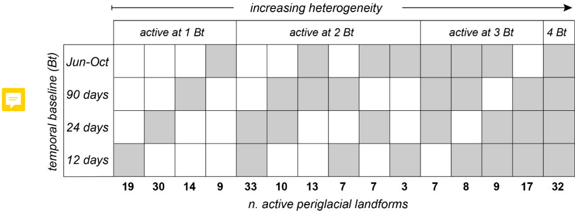
Figure 8. Periglacial landforms active on different temporal baselines (classification with AI_T : 0.4; see text for explanation). From left to right, landforms are active on an increasing number of temporal baselines, suggesting increasingly spatial and/or temporal complexity.
