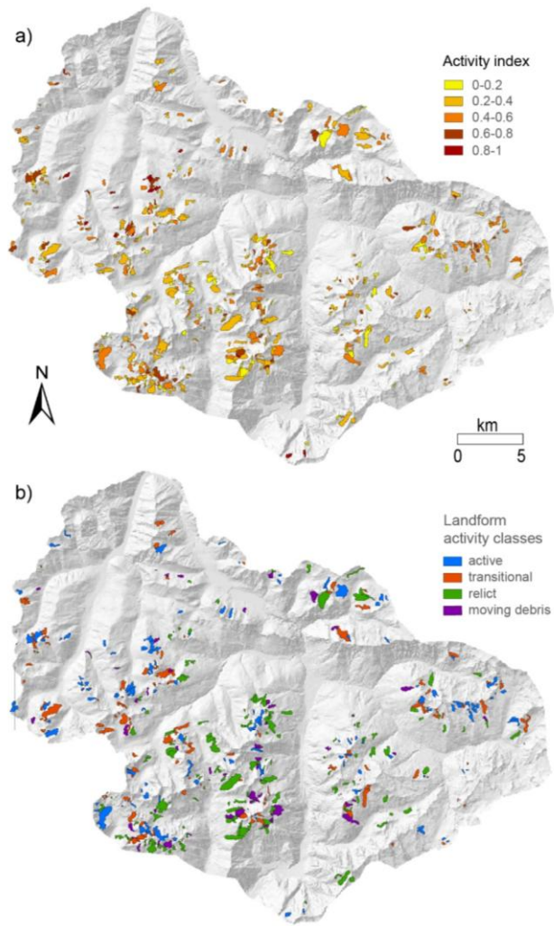
Figure 6. Maps of Activity Index and landform activity classes on a temporal baseline of 24 days; a) polygons classified according to the computed values of Activity Index (0-1);- b) reclassified map obtained considering an AI threshold at 0.4 and the presence of permafrost.
