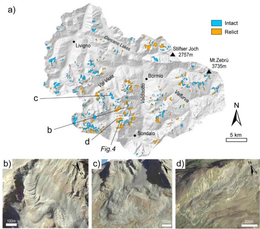
140 Figure 2. Geomorphological classification of periglacial landform activity. a) distribution of activity classes according to Scotti et al., 2013; b,c) intact landforms; d) relict landforms. Landform locations are shown in a). Imagery: Google, ©2021 Maxar Technologies.
