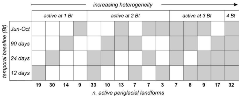
Figure 8. Periglacial landforms active on different temporal baselines (classification with AIT: 0.4; see text for explanation). From left to right, landforms are active on an increasing number of temporal baselines, indicated by grey boxes, suggesting increasingly spatial and/or temporal complexity.
