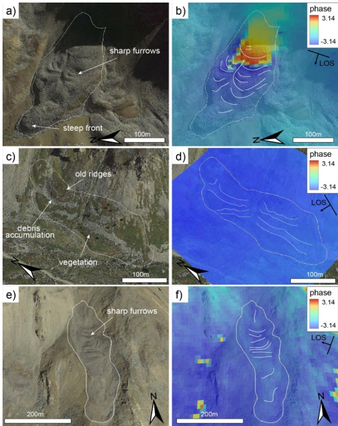
605 Figure 9: comparison between geomorphological and DInSAR-based activity assessment. a) active rock glacier (Bt=24days, AI=0.87), with sharp furrows, ridges and steep front, associated to clear fringe patterns testifying to the activity of the upper part of the rock glacier (b); c) relict rock glacier (Bt=120days, AI=0.19) characterized by abandoned, subdued and vegetated morphological evidence, mirrored in d) by the absence of DInSAR signal; e) active rock glacier with sharp furrows and lobes, for which the SAR sensor is blind (C index = 0.2) resulting in f) a strong underestimation of activity underestimation of its movement (Bt=24days, AI=0.23). Portrayed DInSAR signals are from individual interferograms (not stacked) without APS corrections. Imagery: Google, ©2021 Maxar Technologies. 610
