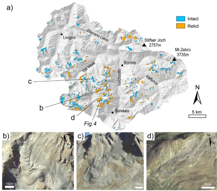
255 Figure 2. Geomorphological classification of periglacial landform activity. a) distribution of activity classes according to Scotti et al., 2013; b,c) intact landforms, d) relict landforms. Landform locations are shown in a). Imagery: Google, ©2021 Maxar Technologies.
