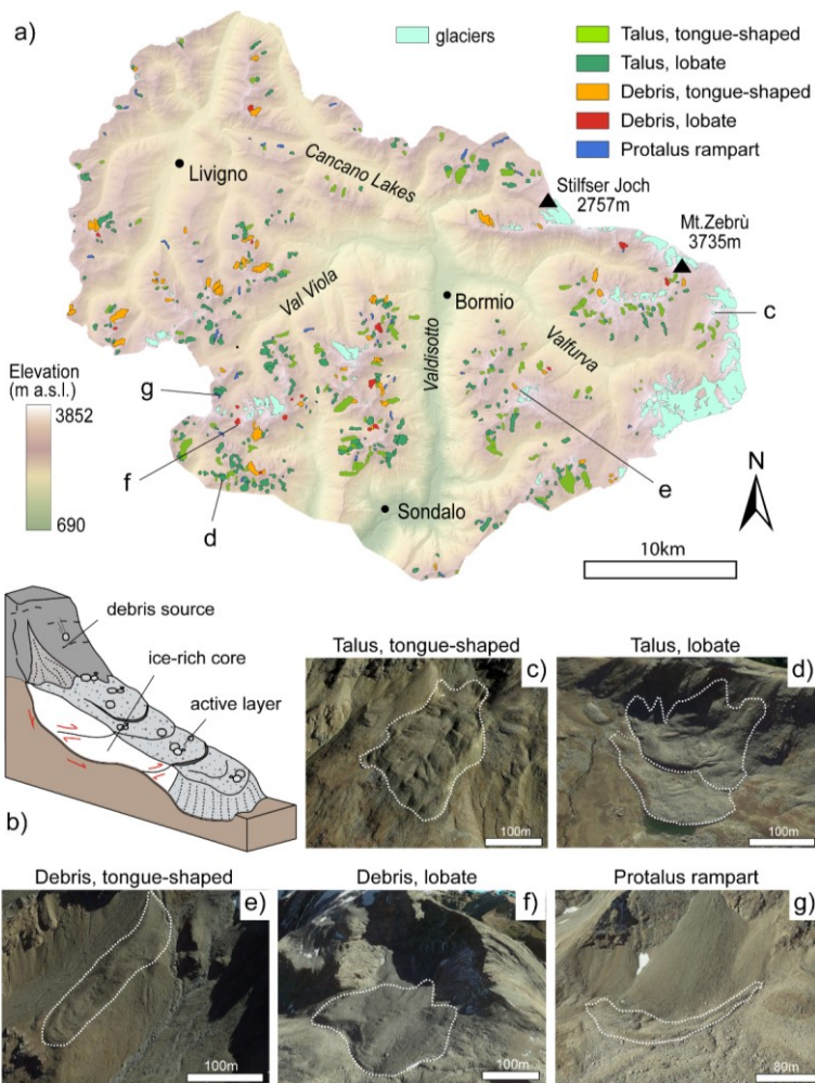
210 Figure 1: distribution and geomorphological classification of periglacial features mapped in the study area (after Scotti et al., 2013). a) inventory map (polygons); b) simplified sketch of an intact rock glacier; c-g) examples of mapped periglacial features, locations shown in a). Imagery: Google, ©2021 Maxar Technologies.
