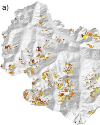
ha eliminato: results Figure 6. Maps of Activity Index and landform activity classes on a temporal baseline of 24 days; a) polygons classified according to the computed values of Activity Index (0-1); b) reclassified map obtained considering an AI threshold at 0.4 and the presence of permafrost.
