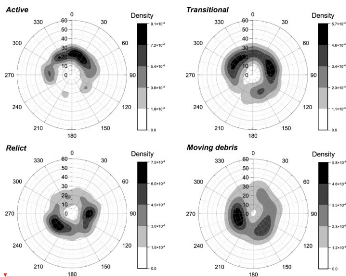
Figure 10. Stereographic (polar) diagrams showing the distribution of the average topographic aspect (i.e. azimuth) and slope (i.e. dip) computed for each mapped periglacial features, falling in different activity classes according to our methodology (Bt=24 days). The relative abundance of periglacial features is expressed in terms of point density.
