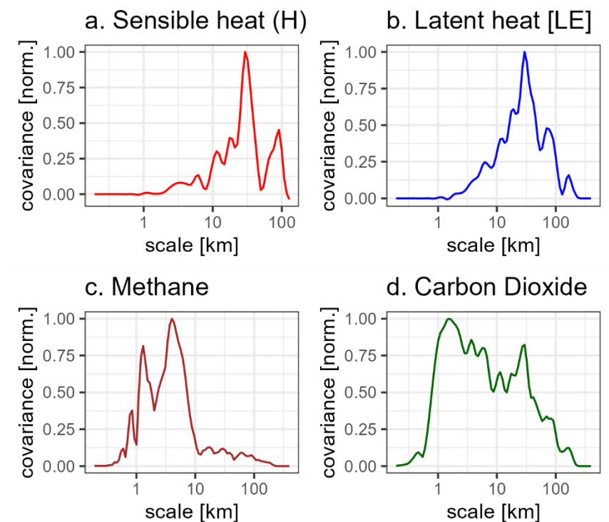
Figure RC2.1: Averaged cospectra from flight legs 29 th of August 2018 and 21 st of August 2019 (in total 11 flight legs were available, for sensible heat only 6 legs were available as no fast Temperature sensor was installed in 2018).
