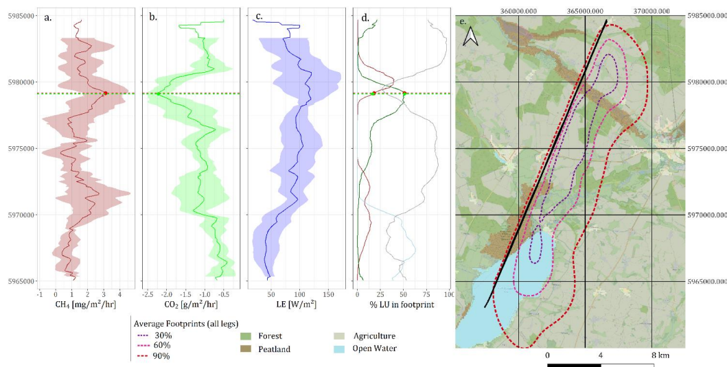
Figure 12: Transect with measured \text{CO}_2 , \text{CH}_4 and LE (latent heat) fluxes over a heterogeneous landscape in Northeast Germany (close to Demmin; date: 29 th August 2018). The location of the transect is shown in figure 12e (background: open street maps). Flux data in graph a – c is based on airborne flight data from 5 flight legs, where thicker lines show the median fluxes and the coloured areas surrounding these lines, indicating the standard deviation of these fluxes. Besides the measured fluxes, land use cover and average footprints (based on footprints from all 5 individual legs) are shown in subfigure d and e. The land use classification presented in this map (subfigure e) is a simplified version of the Corine cover classification of 2018 (Corine Land Cover (CLC) 2018, Version 2020_20u1 (European Environment Agency, 2020)).
