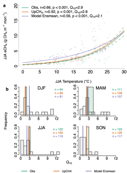
410 Figure 4. Temperature sensitivity of simulated seasonal eCH 4 across locations of FLUXNET-CH 4 sites. a. Model ensemble mean ('Model Ensmean') of simulated eCH 4 against seasonal mean temperature for the JJA season along the temperature gradient at the locations of FLUXNET-CH 4 sites in comparison to the estimates from eddy covariance measurements ('Obs'; Fig. S10; Table S4) and UpCH 4 . Each dot represents the value at one site for an individual year when observations are available. The unit of the simulated CH 4 emissions is g CH 4 m -1 month -1 per standard wetland area to exclude the effect of inundation on eCH 4 . The exponential fitted curves are shown. b. Histogram of the seasonal Q 10 for the 16 individual models for the months DJF, MAM, JJA, and SON. Sample sizes are shown in the plot. The Q 10 values derived from FLUXNET-CH 4 , UpCH 4 , and the model ensemble mean are vertical solid lines, with a width of the bar for 'Obs' indicating the uncertainty range of Q 10 based on measurement uncertainty.
