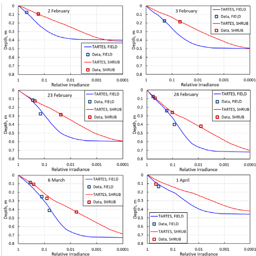
Figure 10. Data and simulations of irradiance profiles at FIELD and SHRUB for 390 nm. The scale of the Y axis varies because snow depth varied. One to three data points were obtained, depending on the number of sensors buried. The X-scale has been inverted to start at the snow surface. The size of the data points represent the error bars.
