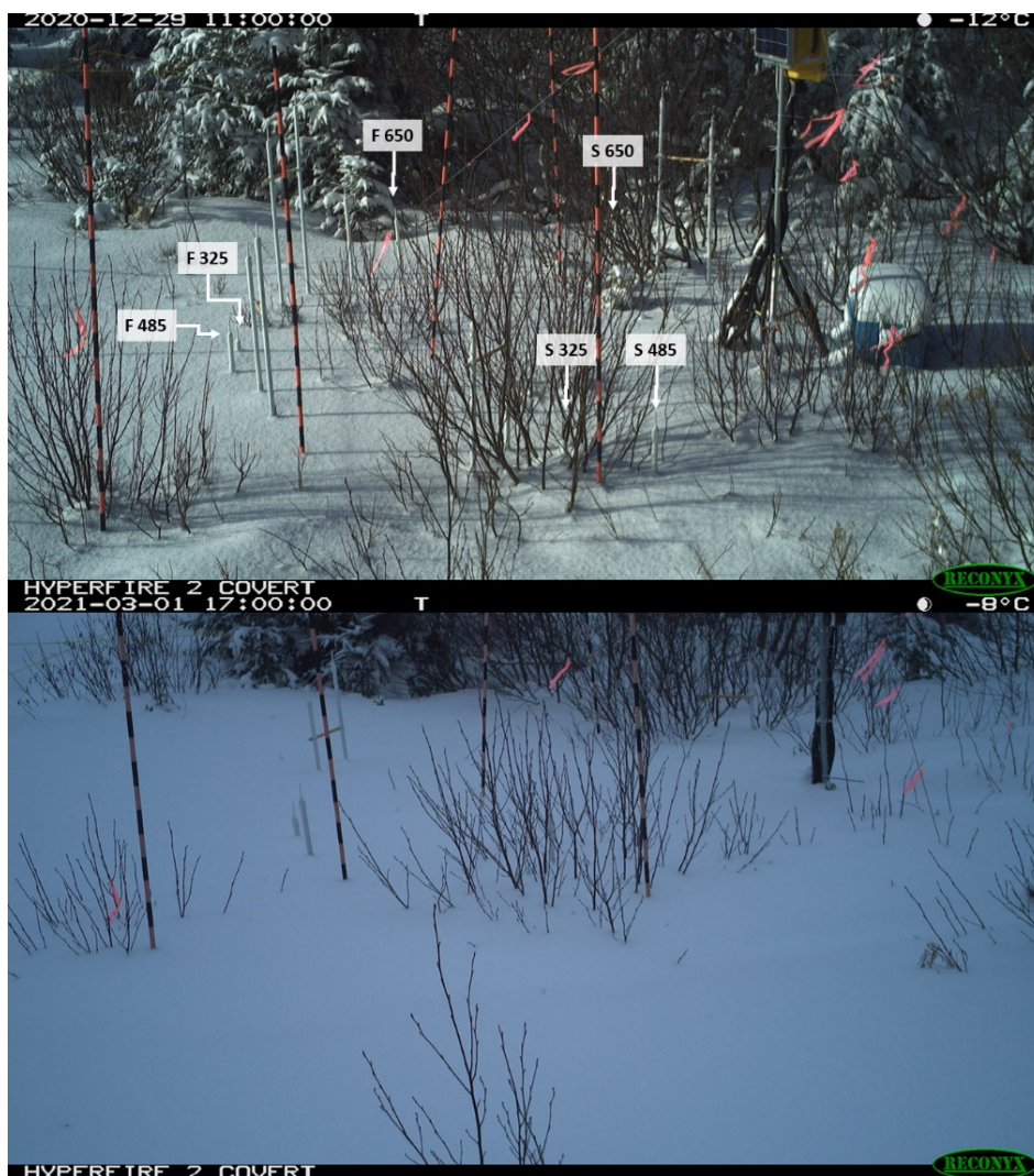
Figure 2. Photographs of the site showing the positions of the sensors. (top) On December 29, 2020, when no sensor was covered by snow. The six sensors whose data were used here are indicated. S325, S485 and S650 are in the SHRUB spot at heights of 325, 485 and 650 mm. F325, F485 and F650 are in the FIELD site. (bottom) Same view at peak snow height on March 1 st , 2021, when the six sensors were buried. Note that the snow bent the branches, modifying the branch environment of the S sensors visible on top.
