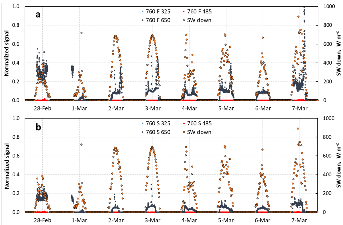
255 Figure 9. Time series of normalized irradiance I_{r,i}/I_{0r} at 760 nm for the sensors at 325, 485 and 650 mm, when all three were buried. The downwelling solar irradiance (SW down) from the CNR4 is also shown. (a) FIELD, (b) SHRUB. The signals from the sensors at 325 and 485 mm are too low for detection.
