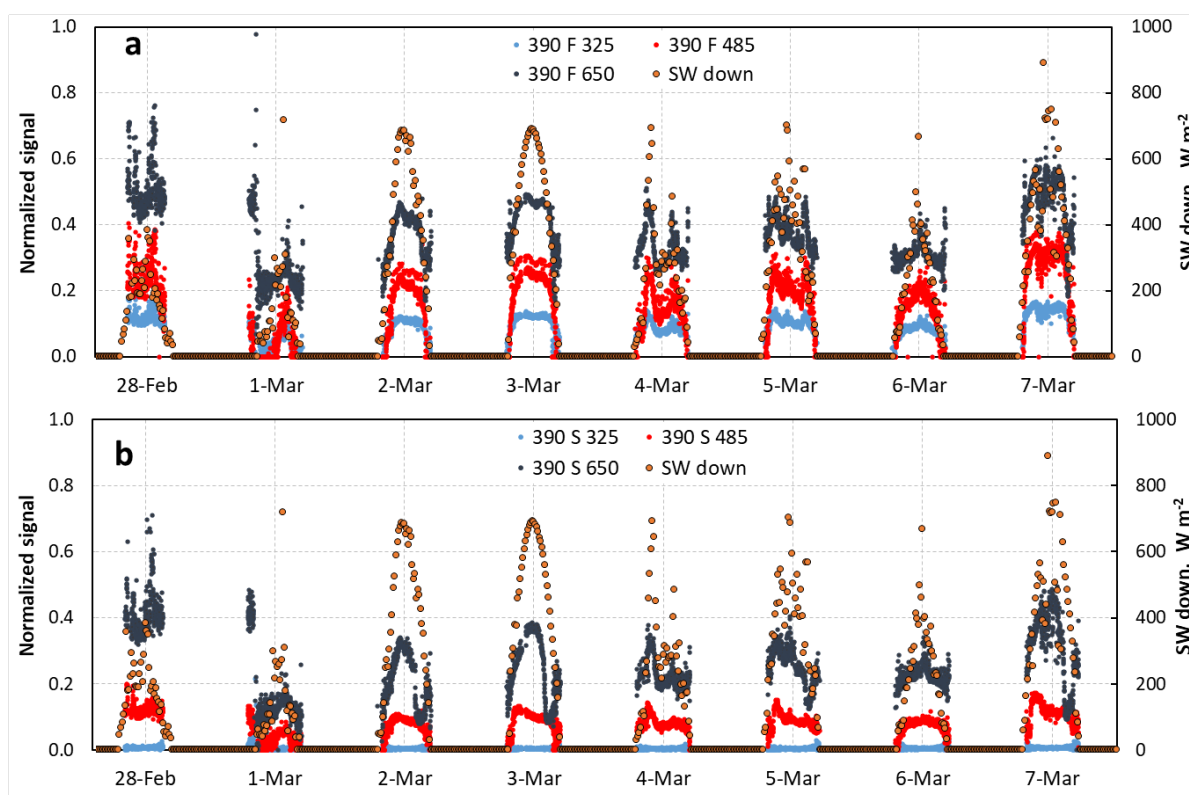
240 Figure 7. Time series of normalized irradiance I_{r,i}/I_{0b} at 390 nm for the three sensors at 325, 485 and 650 mm heights, when these three sensors were buried. The downwelling solar irradiance (SW down) from the CNR4 is also shown. (a) FIELD, (b) SHRUB. 390 F 325 is the signal for the 390 nm (blue) wavelength of the FIELD sensor at the 325 mm level. 390 S 325 is the same, but for the SHRUB sensor. SW down is the downwelling shortwave radiation measured by the CNR4.
