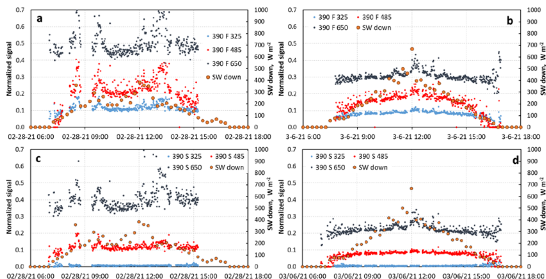
250 Figure 8. Daily evolution of the normalized irradiance I_{r,i}/I_{0b} under mostly overcast conditions. (a) FIELD, February 28 th (b) FIELD, March 6 th (c) SHRUB, February 28 th (d) SHRUB, March 6 th .
