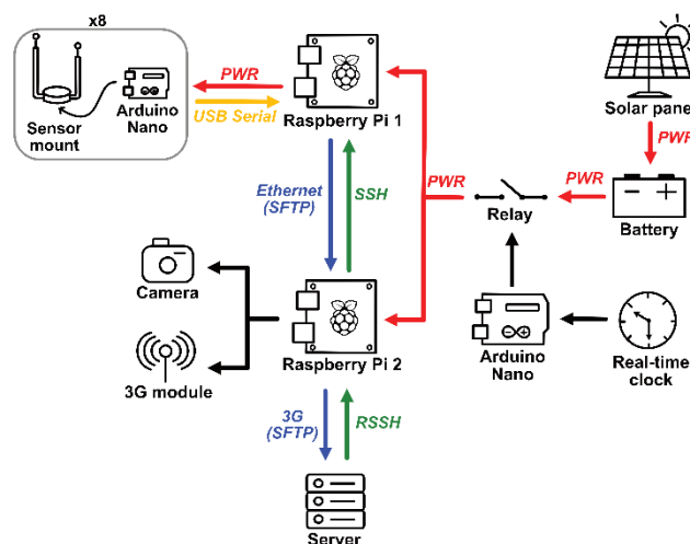
150 Figure 3. Schematic of the signal acquisition and transmission system. The Raspberry Pi 1 received the data stream from each of the eight sensor pairs, while the Raspberry Pi 2 handled data transmission over internet to the server. The whole system was operated exclusively during daytime hours (7AM-6PM).
