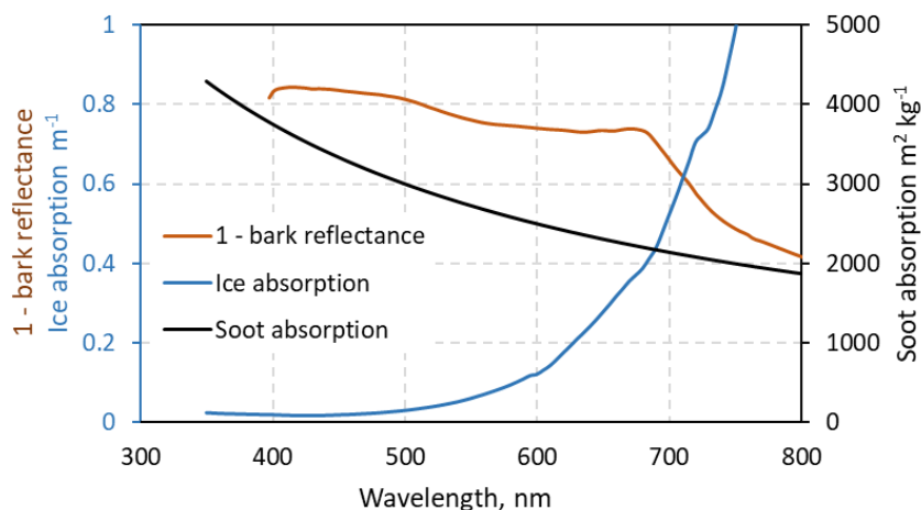
210 Figure 4. Absorption coefficients of ice and soot used in this study. The reflectance of Alnus incana bark provided by (Juola et al., 2022a) is also shown.
