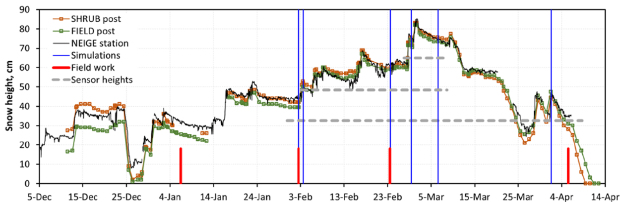
Figure 6. Time series of snow height at the striped poles placed at the study site and determined daily from time lapse images. Snow height monitored by an ultrasonic gauge at the NEIGE station 1.75 km away is also shown. Dates of field work when snow density and specific surface area were measured are indicated with bold red vertical bars. Dates for which irradiance profiles were simulated
