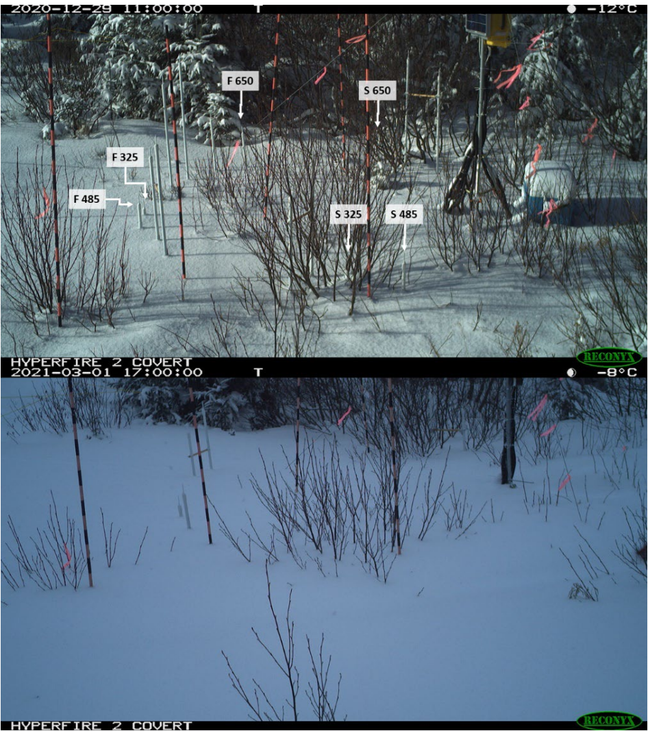
125 Figure 2. Photographs of the site showing the positions of the sensors. (top) On December 29, 2020, when no sensor was covered by snow. The six sensors whose data were used here are indicated. S325, S485 and S650 are in the SHRUB spot at heights of 32.5, 48.5 and 65 cm. F325, F485 and F650 are in the FIELD site. (bottom) Same view at peak snow height on March 1 st , 2021, when the six sensors were buried. Note that the snow bent the branches, modifying the branch environment of the S sensors visible on top.
