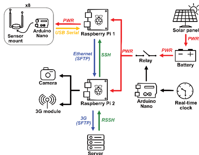
155 Figure 3. Schematic of the signal acquisition and transmission system. The Raspberry Pi 1 received the data stream from each of the eight sensor pairs, while the Raspberry Pi 2 handled data transmission over internet to the server. The whole system was operated exclusively during daytime hours (7AM-6PM). PWR: Power; SSH: Secure Shell protocol; RSSH: Reverse SSH protocol; SFTP: SSH File Transfer Protocol.
