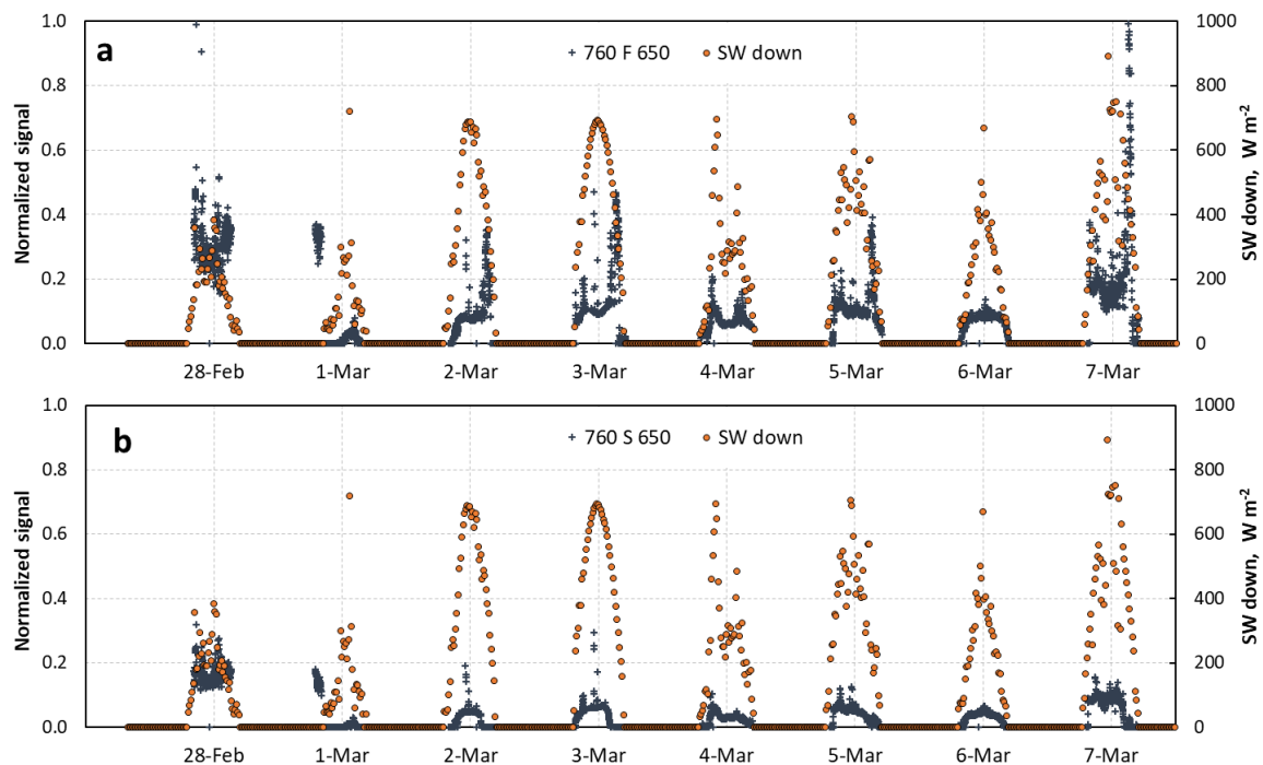
Figure 9. Time series of normalized irradiance I_{r,i}/I_{0r} at 760 nm for the sensor at 65 cm. The downwelling solar irradiance (SW down) from the CNR4 radiometer is also shown. (a) FIELD, (b) SHRUB. The signals from the sensors at 32.5 and 48.5 cm are too low for detection and are not shown.
