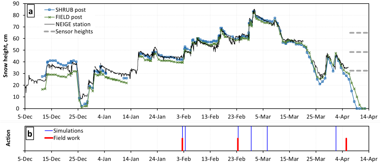
245 Figure 6. Time series of snow height and actions relevant to snow investigations. (a) Snow height at the striped poles placed at the study site and snow height monitored by an ultrasonic gauge at the NEIGE station 1.75 km away. The heights of the three sensors that provided irradiance data are also shown. (b) Dates for which irradiance profiles were simulated and field work dates, when snow density and specific surface area profiles were measured.
