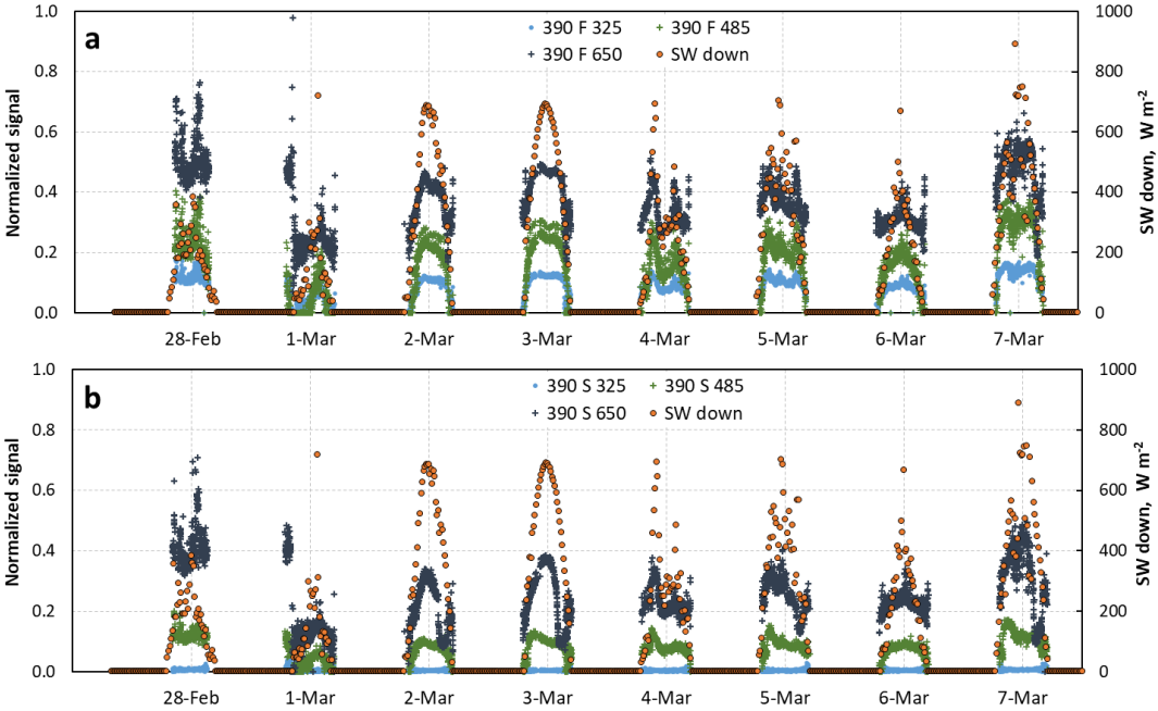
Figure 7. Time series of normalized irradiance I_{r,i}/I_{0b} at 390 nm for the three sensors at 32.5, 48.5 and 65 cm heights, when these three sensors were buried. The downwelling solar irradiance (SW down) from the CNR4 radiometer is also shown. (a) FIELD, (b) SHRUB. 390 F 325 is the signal for the 390 nm (blue) wavelength of the FIELD sensor at the 32.5 cm level. 390 S 325 is the same, but for the SHRUB sensor. SW down is the downwelling shortwave radiation measured by the CNR4.
