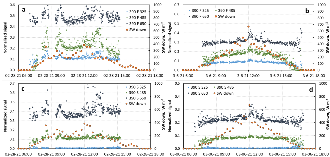
Figure 8. Daily evolution of the normalized irradiance I_{r,i}/I_{0b} under mostly overcast conditions. (a) FIELD, February 28 th (b) FIELD, March 6 th (c) SHRUB, February 28 th (d) SHRUB, March 6 th . For the February 28 th data, the time range 10:30 to 12:30 was used. For the March 6 th data, the time range 7:00 to 16:00 was used, with the exclusion of the 11:30–13:00 time range.
