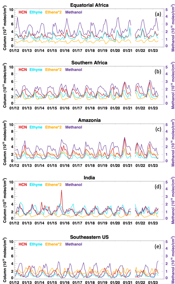
565 Figure 7: Monthly mean VOC timeseries (2012-2023) as detected from SNPP-CrIS using the ROCRv2 retrieval. Data are shown for (a) equatorial Africa, (b) southern Africa, (c) Amazonia, (d) India, and (e) and the southeastern US, with regions mapped in Fig. S3. Quantities shown represent above-background column enhancements derived at a globally-fixed P_{90} value as described in-text.
