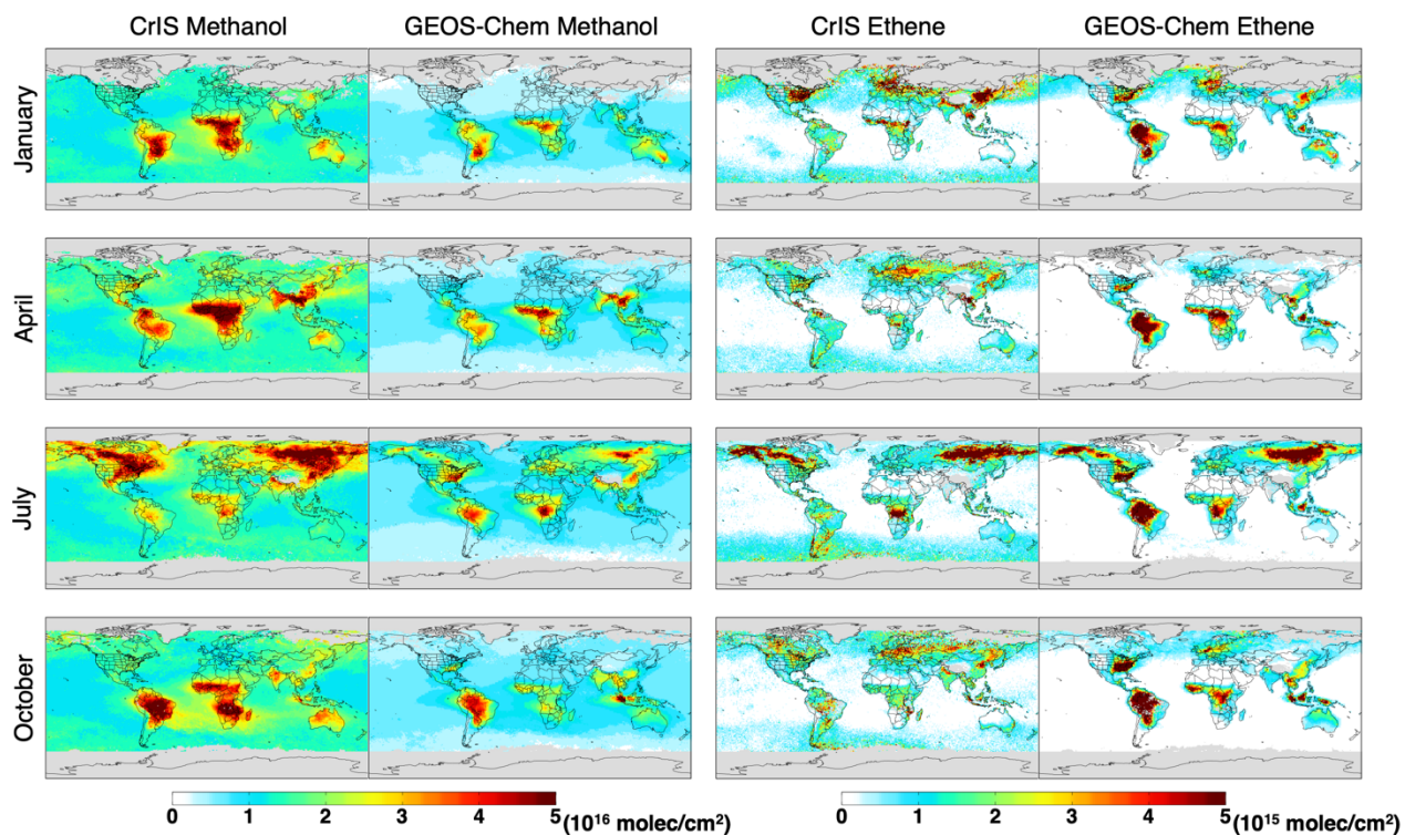
590 Figure 12: Global methanol and ethene column distributions as observed by CrIS and simulated by GEOS-Chem for January, April, July, and October 2019. The CrIS data are adjusted to the model-predicted P_{90} values in each case. Both datasets are screened as described in-text.
