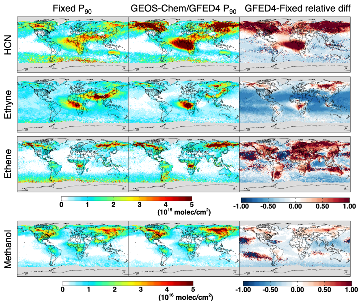
580 Figure 10: Accounting for variable vertical VOC profiles in the CrIS retrievals. Plotted are CrIS-retrieved column enhancements as derived for July 2019 when using a globally fixed P_{90} (left column), or when accounting for P_{90} variability based on a GEOS-Chem simulation using GFEDv4 biomass burning emissions (middle column). Right column shows the relative difference between the two (GFEDv4-fixed P_{90} column).
