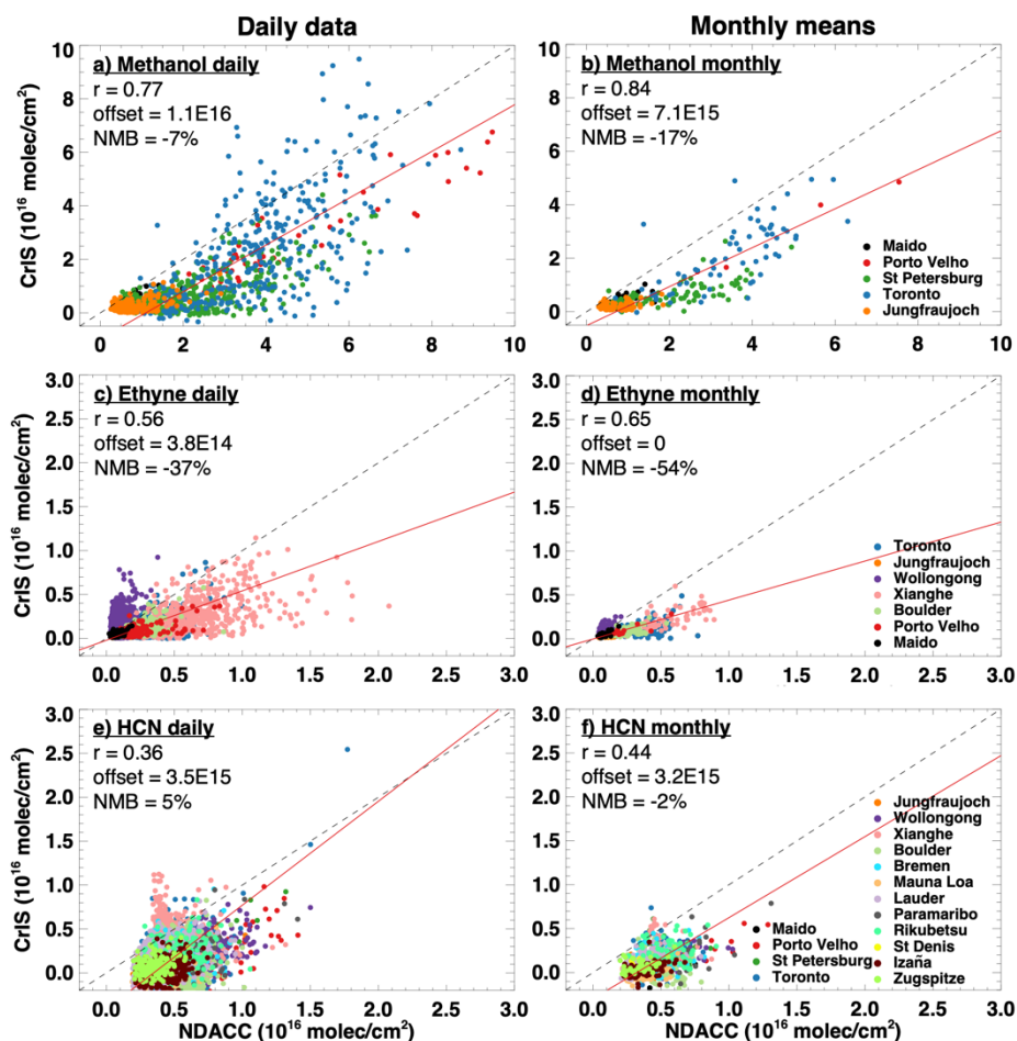
585 Figure 11: Evaluation of the CrIS VOC retrievals against NDACC ground-based FTIR measurements. Data shown compare the CrIS column enhancements against the NDACC total columns on both a daily (left column) and monthly mean (right column) basis. CrIS retrievals have been interpolated to the NDACC-retrieved P_{90} values and corrected for CrIS/NDACC elevation differences as described in the text. Normalized mean biases (NMB) are computed for the offset-corrected data.
