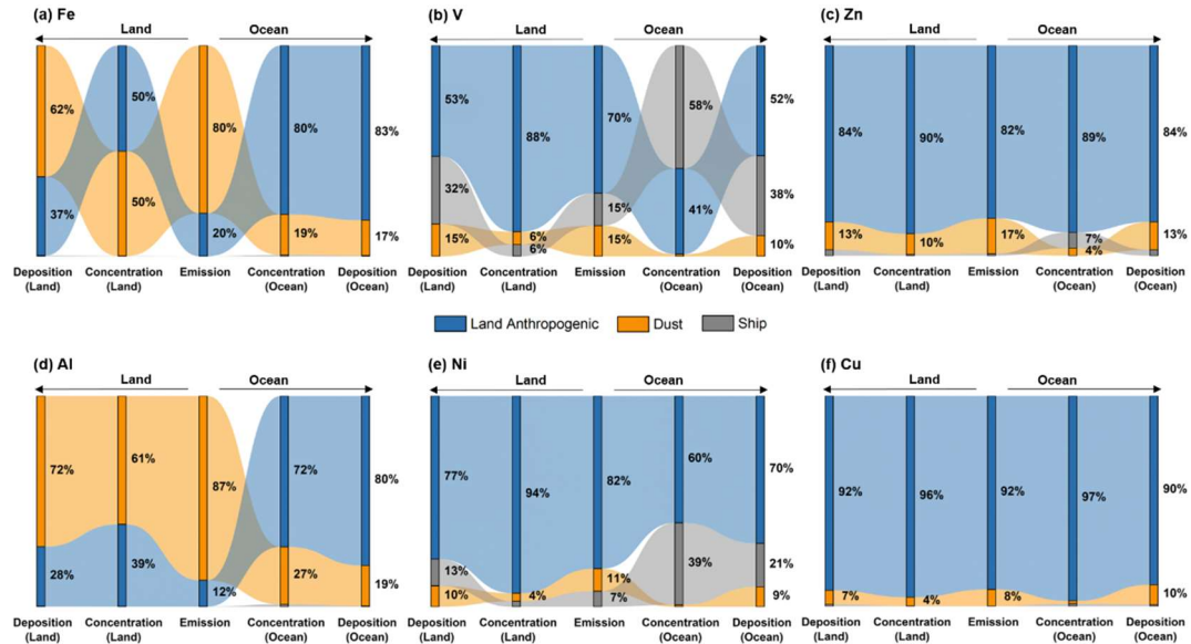
Figure 9: Evolution of the relative contributions of the land anthropogenic, ship, and dust sources to emissions, seasonal mean atmospheric concentrations , and annual deposition fluxes of Fe (a), V (b), Zn (c), Al (d), Ni (e), Cu (f) (Concentrations and depositional fluxes labelled "Ocean" in the figure were for the oceans only, and concentrations and depositional fluxes labelled "Land" were for land only).
