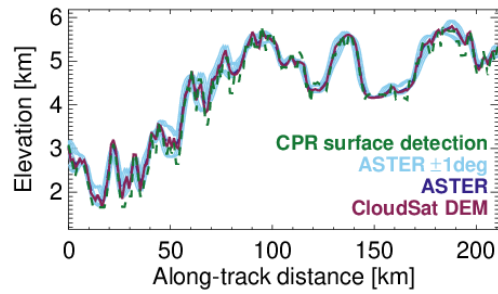
305 Figure 7. Comparison between different elevation heights corresponding to the L1 CloudSat surface detection height, the ASTER DEM simulated surface elevations with and without \pm 1 degree along- and cross-track offsets and the DEM information reported in the CloudSat 2B-GEOPROF product.
