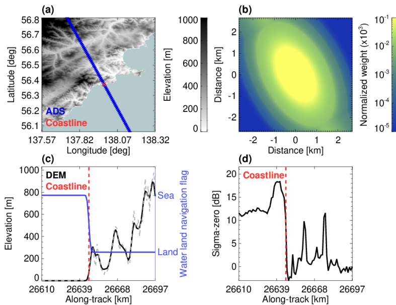
125 Figure 1. An example of the geolocation evaluation tool using actual CloudSat CPR data. Panel (a) shows the CloudSat orbit path (blue dots) defined by the Attitude Determination System (ADS) with the identified coastline crossing location (red dot) over the ASTER DEM. Panel (b) shows the CloudSat CPR's along-track integrated footprint rotated according to the orbit inclination in ascending mode. Panel (c) shows the original DEM (grey dashed line), the simulated DEM using the satellite's footprint (black line), the coastline location (red dashed line) and a simulated water land navigation flag (blue line). Panel (d) shows the coastline location (red dashed line) and the actual measured normalized surface radar cross section ( \sigma_0 ) measured by the CloudSat CPR (black line).
