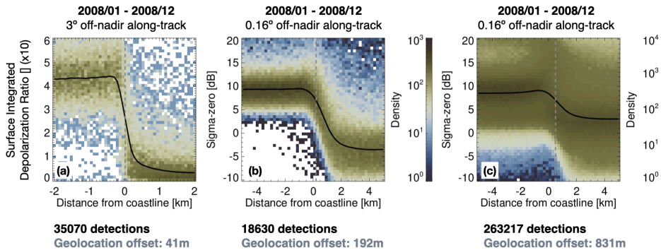
220 Figure 4. Histogram of (a) CALIPSO CALIOP 532nm surface integrated depolarization ratio ( \delta ) and (b) CloudSat CPR normalized radar surface cross section ( \sigma_0 ), as a function of distance from the coastline, using measurements from 2008 over the selected coastal areas. Panel (c) presents the CloudSat results when applied to the global coastlines dataset. The black line represents the median of the signal while the grey dashed line indicates the overall coastline detection.
