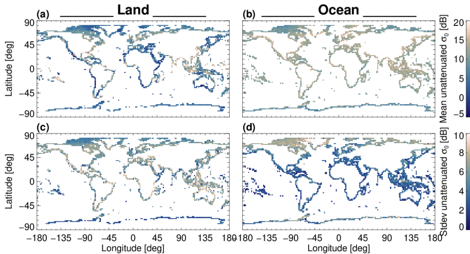
Figure 2. Climatological CloudSat CPR \sigma_0 statistics (mean and standard deviation) over land (panels a and c) and ocean (panels b and d).
