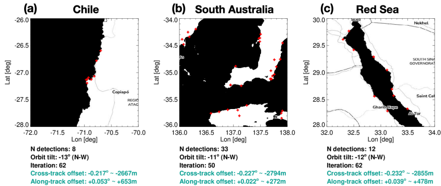
345 Figure 8. Examples of the coastline geolocation assessment using CloudSat data from July to September 2020. The red dots represent the detections. The base maps are © OpenStreetMap contributors 2015, distributed under the Open Data Commons Open Database License (ODbL) v1.0.
