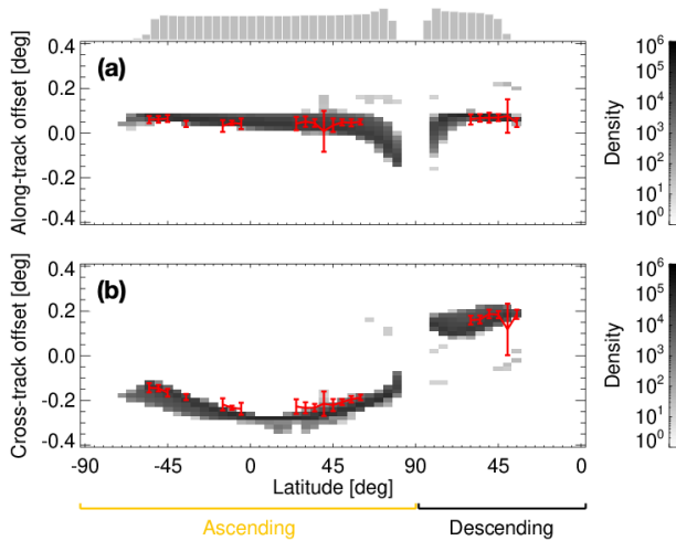
390 Figure 11. (a) along- and (b) cross-track validation offsets. The background histogram illustrates the validation geolocation offsets, based on the latitude/longitude differences between the two CloudSat datasets — before and after the star tracker catalogue correction — covering data from July to September 2020. The red lines represent the 95% confidence intervals of the results obtained from the geolocation tools.
