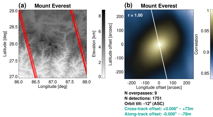
Figure 6. The CloudSat geolocation assessment around the Mount Everest. Panel a illustrates the area with significant elevation gradients, with red lines representing the CloudSat overpasses from January to March 2008. The statistical
