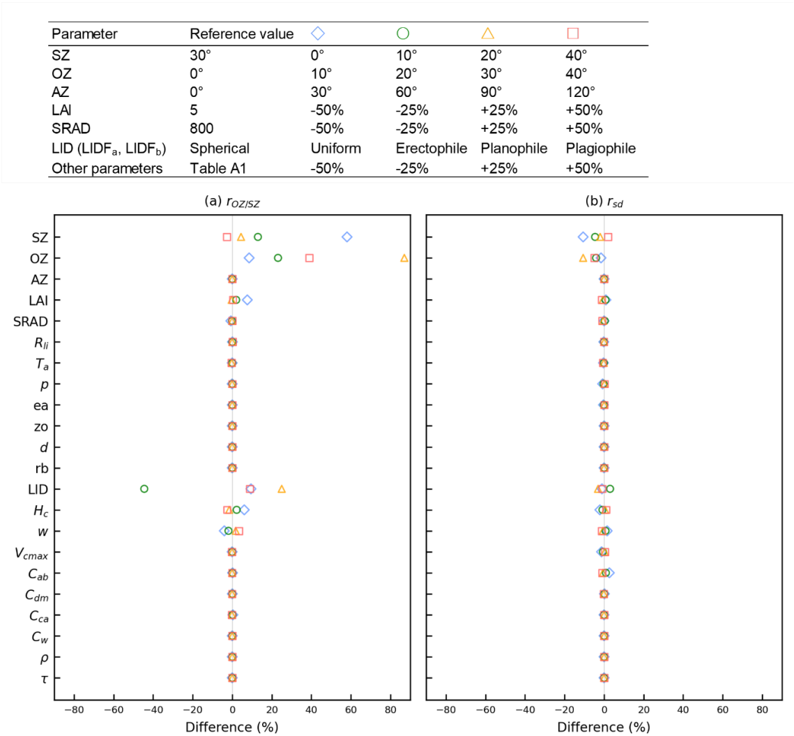
Figure B1. The impact of r_{oz/sz} and r_{sd} on SIF calculations ( F in Eq. (1)) when changing each input parameter in Table A1. The impact was estimated using SCOPE by changing input parameters as shown in the upper table. The difference of 0 indicates that the simulation results from LUT and SCOPE are identical when parameters that are not used in LUT.
