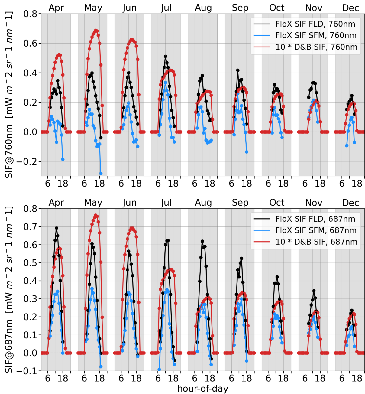
Figure 10. Average hourly diurnal cycle by month of SIF in the far-red ( upper panel ) and red ( lower panel ) for evergreen trees (PFT 3) at Majadas de Tietar for months April to December in 2021. D&B simulations (red) against measurements: retrievals made with Fraunhofer line discrimination (black) and spectral fitting method (blue).
