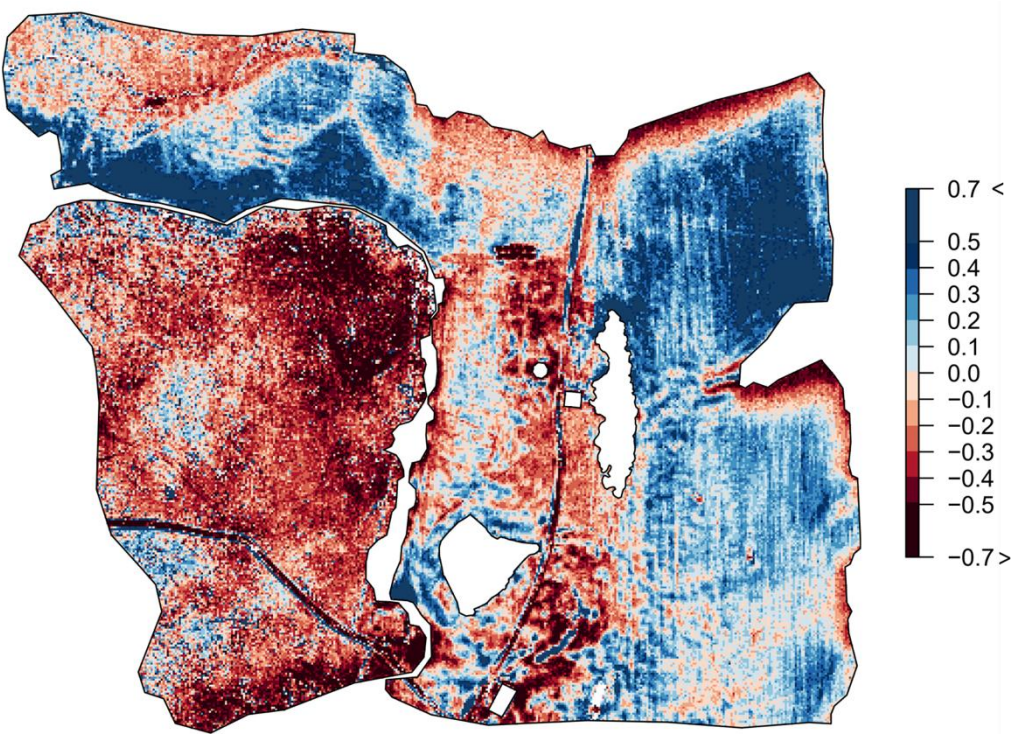
335 Figure 6 The snow depth mean relative difference (MRD) map generated by averaging the eight relative difference maps from the UAS lidar-based snow depth maps from February 4th to March 7th.
