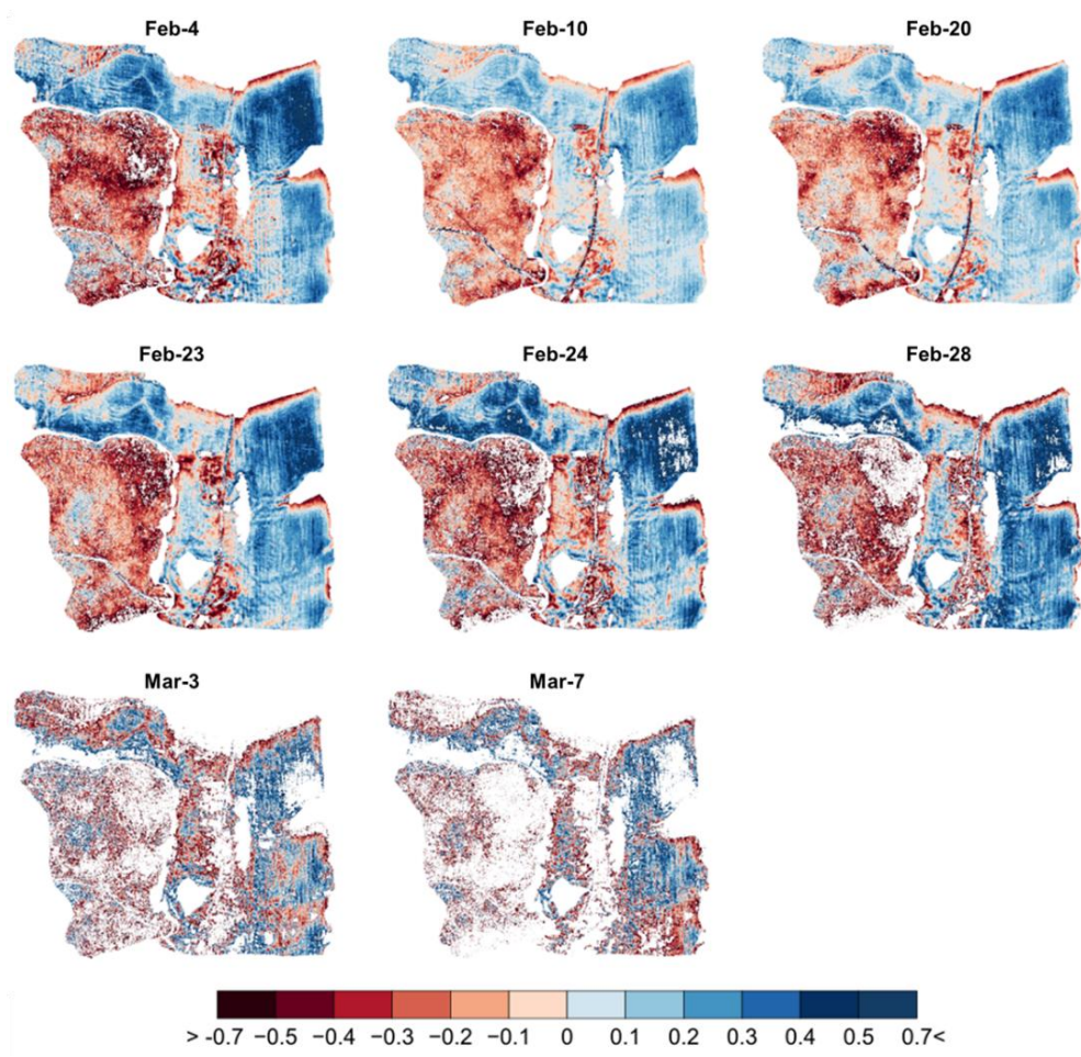
Figure 7 Relative difference maps generated from the UAS lidar-based snow depth maps from February 4th to March 7th. The white areas in the figures indicate either masked areas (e.g., ponds and facilities) or areas with no snow.
