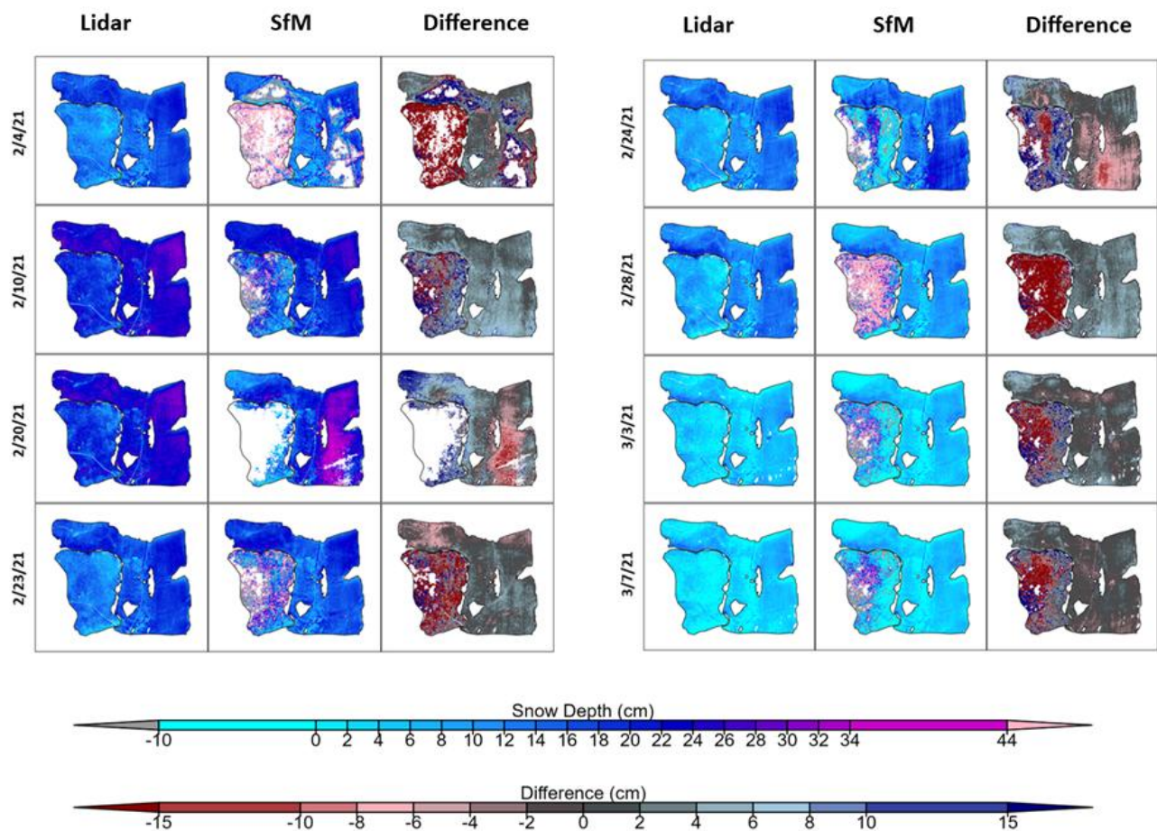
Figure 5 Time series of snow depths for UAV Lidar and SfM in the field and forest. Difference is calculated as Lidar snow depth minus SfM snow depth. All values are shown in cm.
