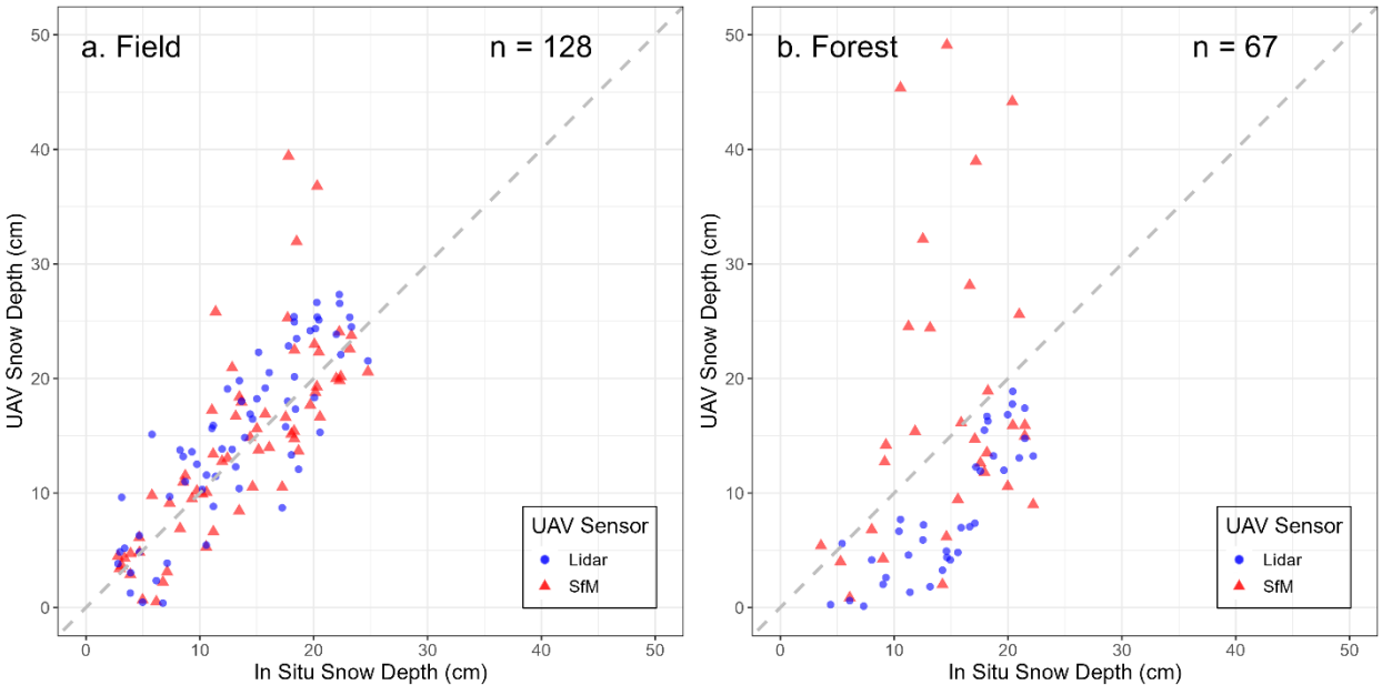
290 Figure 3 UAV-based snow depth measurements compared to in situ snow depth measurements from the magnaprobe. UAS-measured snow depths are shown for pixels overlapping the magnaprobe sample locations. Measurements collected on all dates are shown for the field (a) and forest (b). N-values indicate the number of samples shown within the plot axes. UAV-measured snow depths which exceeded 50 cm are not shown (1 SfM field, 6 SfM forest). Magnaprobe sample locations corresponding to UAS pixels with missing snow depth values are not shown (1 SfM field, 6 SfM forest, 7 lidar forest).
