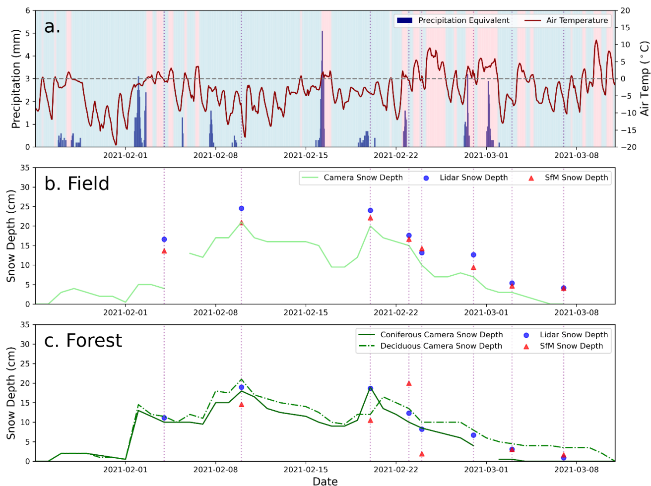
Figure 2 Time series of conditions at the Thompson Farm, Durham NH study area during the 2021 winter season including: hourly precipitation equivalent (mm) and temperature (°C) measured by a USCRN station (a) and daily camera snow depths and median UAS-measured snow depths in the field (b) and forest (c). Dates corresponding to the in situ and UAS sampling campaigns are marked by the dotted vertical lines. Periods where the temperature was colder than 0°C are indicated by the blue plot background and periods warmer than 0°C are indicated in pink in (a). Median SfM-measured snow depths in the forest on 2/4/21 and 2/28/21 exceeded 35 cm and are not shown (172 cm and 86 cm, respectively).
