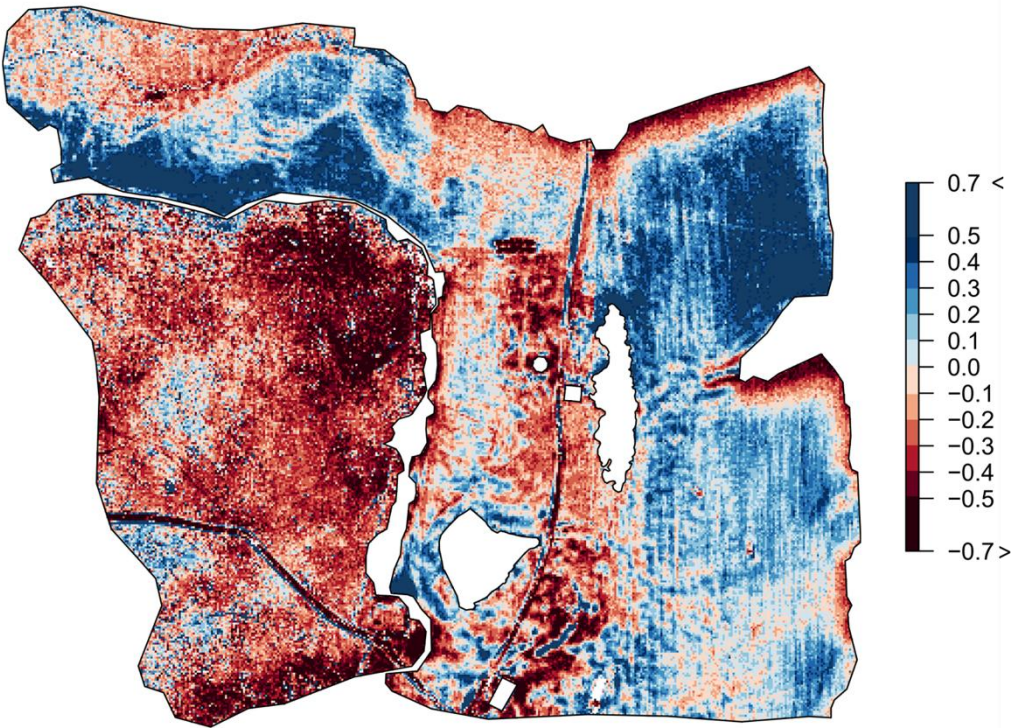
335 Figure 6 The snow depth mean relative difference (MRD) map generated by averaging the eight relative difference maps from the UAS lidar-based snow depth maps from February 4th to March 7th.
