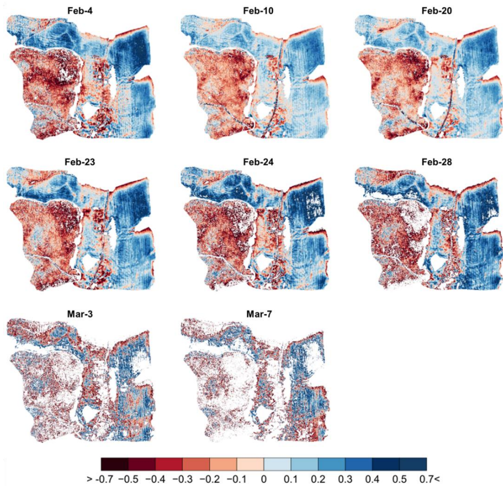
Figure 7 Relative difference maps generated from the UAS lidar-based snow depth maps from February 4th to March 7th. The white areas in the figures indicate either masked areas (e.g., ponds and facilities) or areas with no snow.
