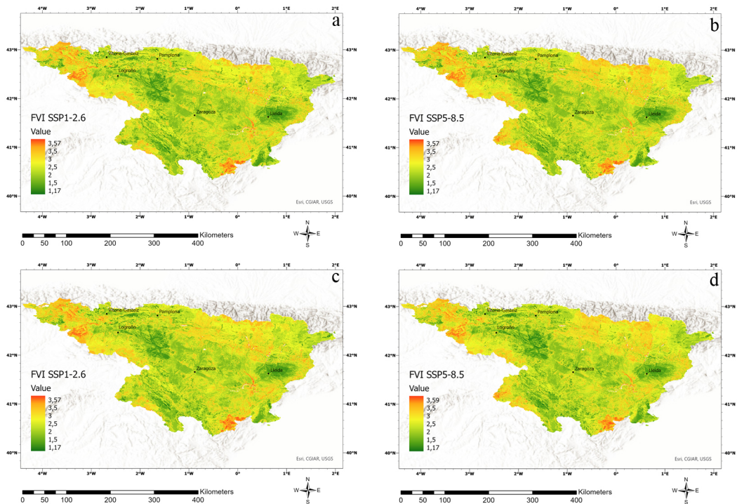
Figure S7. Spatial distribution of the FVI without wildfire effects for a) SSP1-2.6 year 2100 and b) for SSP5-8.5 year 2100, and with wildfire effects for c) SSP1-2.6 year 2100 and d) SSP5-8.5 year 2100.
