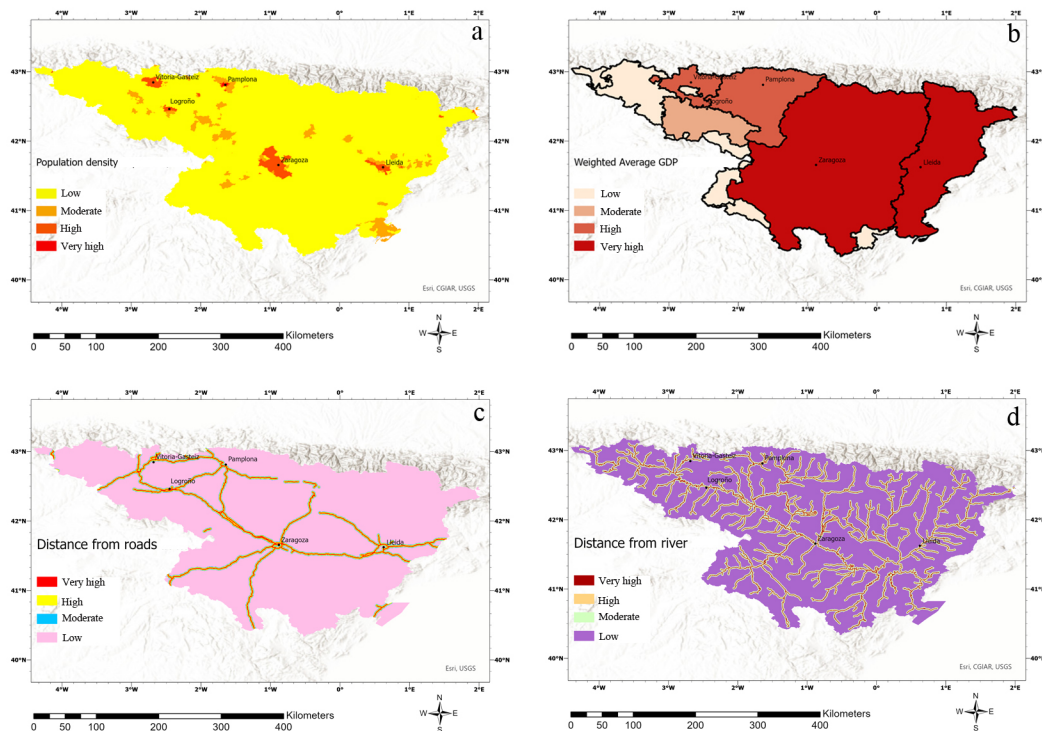
Figure S2. Spatial distribution of the classification for the exposure indicators for the baseline scenario with a) the population density, b) the total weighted average GDP, c) the distance from roads, and d) the distance from river.
