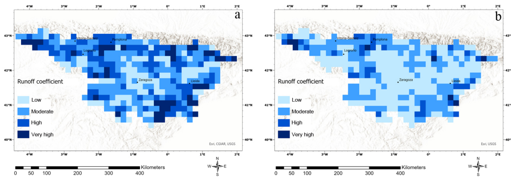
Figure S5. Spatial distribution of the runoff coefficient classification for a) SSP1-2.6 year 2100 and b) for SSP5-8.5 year 2100.
