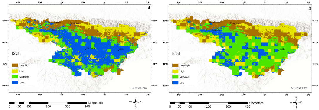
Figure S8. Spatial distribution of saturated hydraulic conductivity with wildfire effects for a) SSP1-2.6 year 2100 and b) for SSP5-8.5 year 2100.
