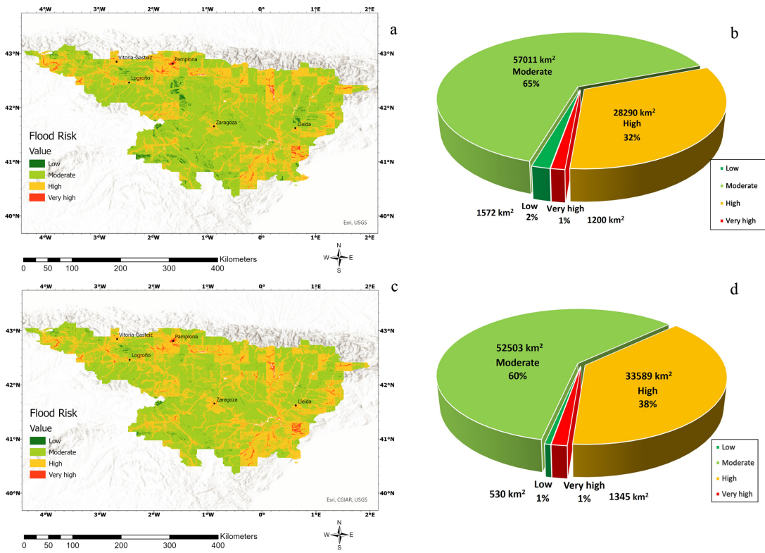
Figure S9. a) Flood risk map without wildfire effects in the Ebro River basin for SSP1-2.6 year 2100, b) distribution of flood risk classes without wildfire effect for SSP1-2.6 year 2100 corresponding to surface area in km 2 , c) same as a but with wildfire effect, and d) same as b but with wildfire effect.
