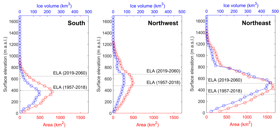
Figure 6. Glacier area (red) and volume in 50-m elevation bins in south (left), northwest (middle) and northeast Svalbard (right). ELA values for 1957-2018 and 2019-60 are taken from Van Pelt et al Van Pelt et al. (2019, 2021). (2019, 2021). Region boundaries for south, northwest and northeast Svalbard are shown in Fig. 1c.
