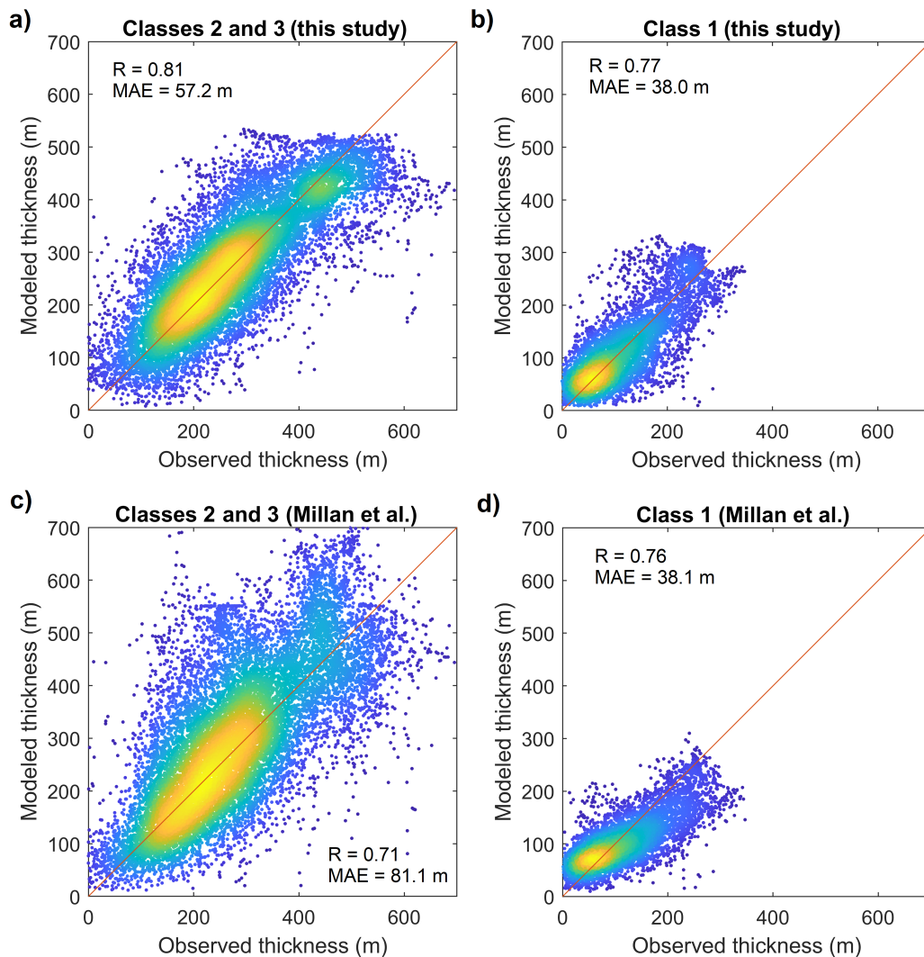
Figure 7. Comparison of modeled and observed ice thickness for glaciers modeled with PISM output from our study (a-b) and surging glaciers Millan et al. (2022) (ac-d) , and split into data for glaciers modeled with IGM in classes 2 and 3 (a and c) and class 1 (b and d) . Thickness observations are from the GlaThiDa database (GlaThiDa Consortium, 2020). The comparison comparisons in a )-is- and c are based on 500-m resolution output, whereas the comparison comparisons in b )-is- and d are based on 100-m resolution output. The dot color represents the density of data points, ranging from dark blue (lowest density) to bright yellow (highest density).
