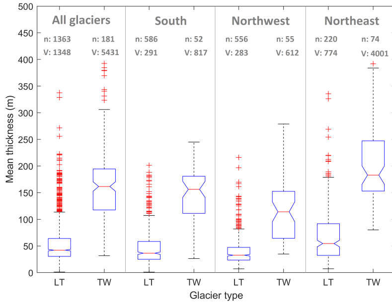
Figure 5. Boxplots Boxplot showing average glacier thickness for land-terminating (LT) and tide-water (TW) glaciers for all glaciers, and split into southern, northwestern and northeastern glaciers. In each category, n is the number of glaciers and V is total glacier volume (in km 3 ). Region boundaries for south, northwest and northeast Svalbard are shown in Fig. 1c.
