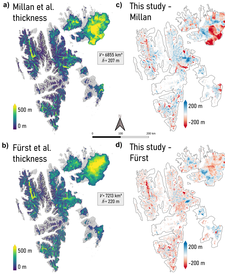
Figure 8. Previous ice thickness maps by Millan et al. (2022) (a) and Fürst et al. (2018b) Fürst et al. (2018a) (version 1.1) (b), and the corresponding differences with our results (c-d).
