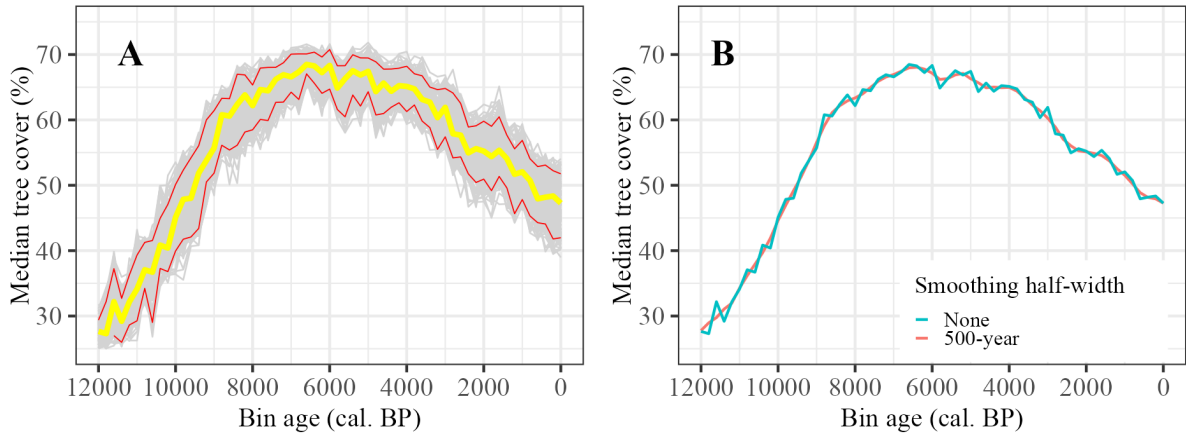
Figure 5: A - Median reconstructed tree cover for Europe from 12,000 to 0 cal. BP, with 95% confidence intervals for 1000 bootstrap resamplings of records; B - Median reconstructed tree cover for Europe from 12,000 to 0 cal. BP, with differing LOESS regression smoothing half-widths.
