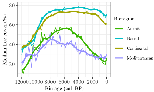
530 Figure 7: Median tree cover values, for selected biogeographical regions. Smoothed lines reflect LOESS fitted regression with 1000-year halfwidth.
