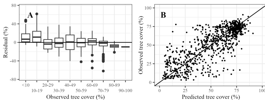
Figure 3: Evaluation of final model performance. A – Differences between predictions and observations (residual), in bins of observed tree cover percentage; B – Predictions of tree cover compared to observed tree cover
