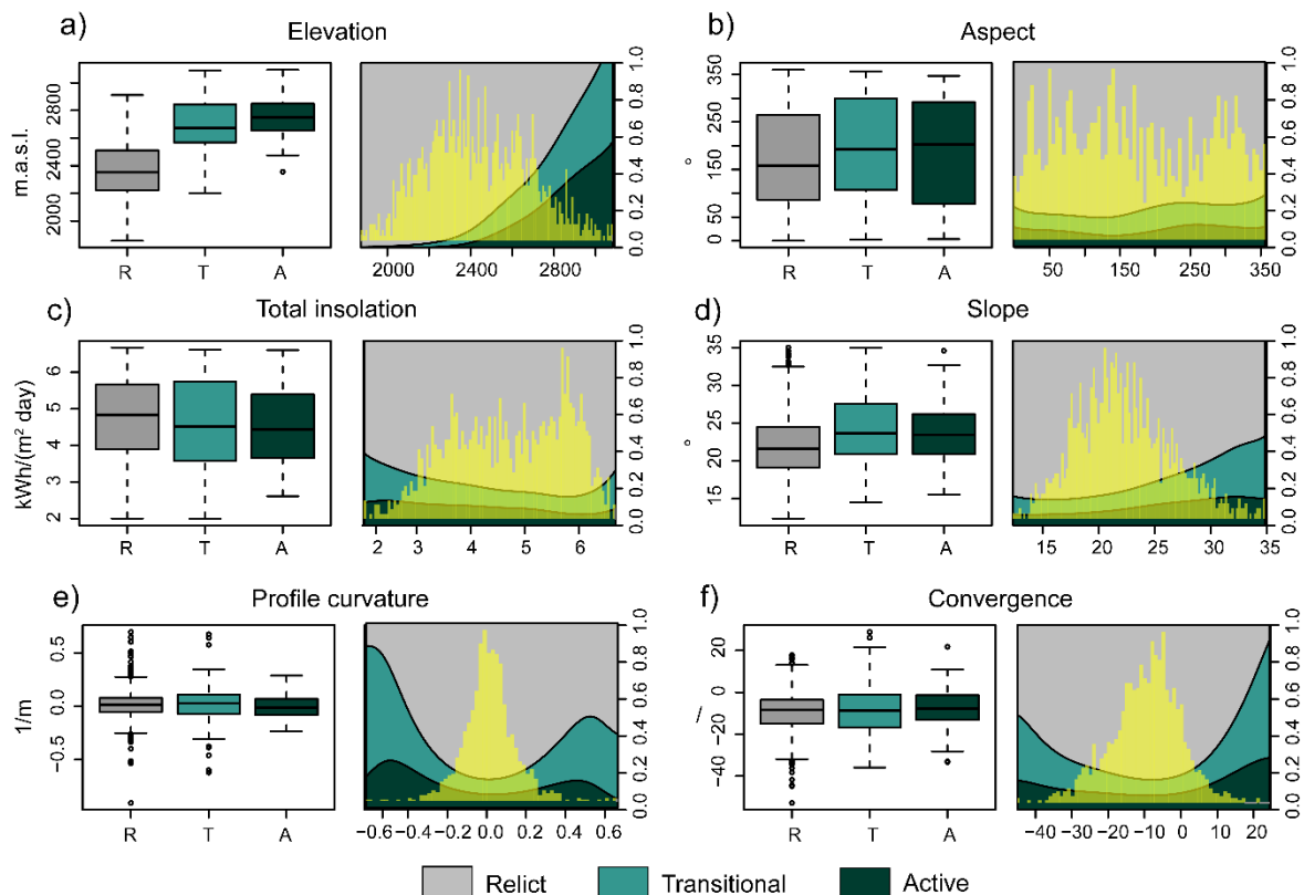
340 Figure 6: morphometric variables that were not retained in the analysis due to their little discriminant capacity between activity classes: a) elevation; b) aspect, computed as mean direction towards north; c) total insolation coming from the combined contribution of direct and diffuse insolation; d) slope angles; e) profile curvature: positive values indicate concave structure of the landform, negative values convex shapes; f) convergence: positive values indicate divergent areas, negative values convergent areas.
