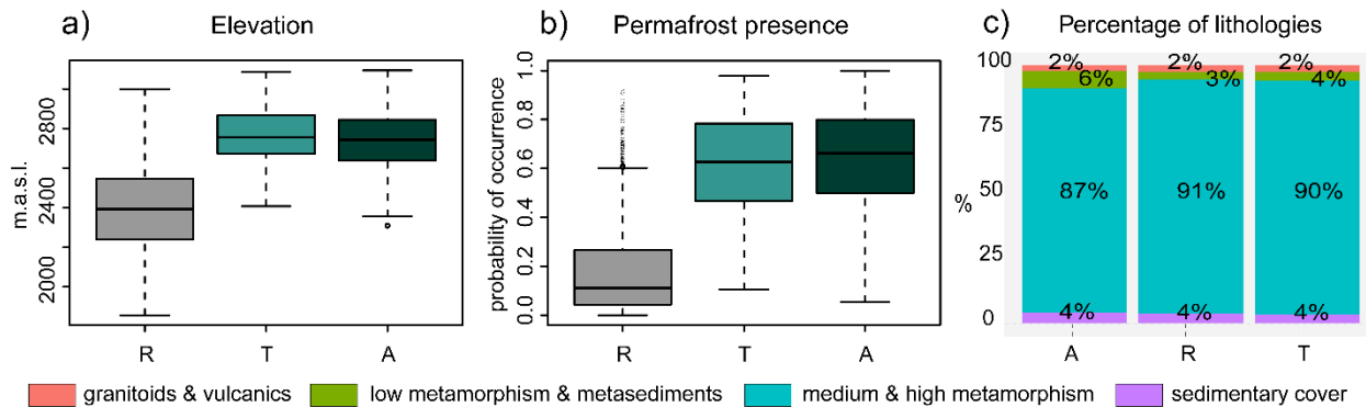
Figure 113: distribution of elevation (a), permafrost presence (b) and percentage of lithologies (c) in the three activity classes: A (active), T (transitional) and R (relict). The lithology names indicated on the line at the bottom of the figure are referred only to the (c) panel.
