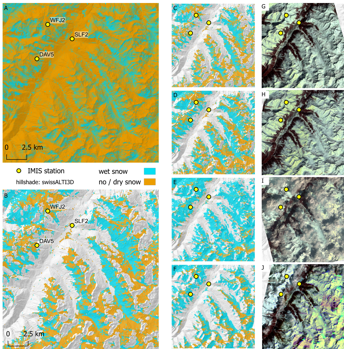
Figure A10. Example case (31.03.2021-03.04.2021) of wet snow detection on a visual comparison. The outline of all the images is the same as the research site displayed in Figure 1.B. A) Based on our processing using LRW, whereas B shows pixels usable from SWS layer on the first acquisition day (Copernicus land monitoring service, 2025). C-F show SWS product for the four acquisitions which were used for creating the LRW based product (C (same as B in different scale): 31.03. D: 01.04., E: 02.04., F: 03.04.2021) and G-J show the corresponding optical imagery from ©Planet Labs PBC. Imagery using false colour infrared (Red: NIR, Green: red, Blue: green). Image contains modified Copernicus Sentinel-1 data (2021).
