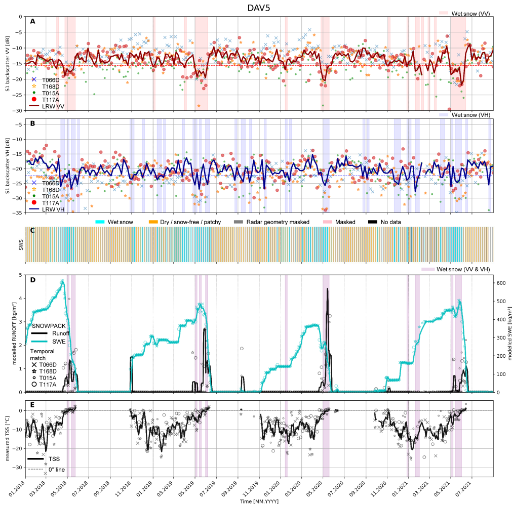
Figure A2. Time series of wet snow evolution over four melting seasons from January 2018 until August 2021 at DAV5 station. A) and B) show the time series extracted from the pixel within which the IMIS station is situated in co- (A) and cross-polarised (B) S1 data. The horizontal line indicates the time series median including the 2 dB threshold and the shading background displays the times during which the backscatter falls below this and wet snow is detected. C) SAR Wet Snow classified layer from Copernicus per each track over the station area. D) Modelled time series of virtual lysimeter (MS SN RUNOFF) and snow water equivalent (SWE) from SNOWPACK data with markers indicating the corresponding time of S1 acquisition and the line being the mean between those four times. Similar E) shows the local measured snow surface temperature (TSS) from IMIS, masked to when snow height as non-zero. In D) and E), the applied purple shading corresponds to our wet snow combined polarisation product.
