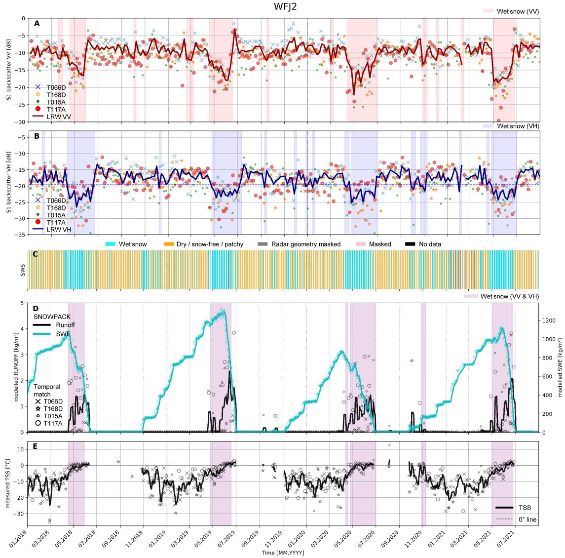
Figure 2. Time series of wet snow evolution over four melting seasons from January 2018 until August 2021 at Weissfluhjoch (WFJ2). A) and B) show the time series extracted from the pixel within which the IMIS station is situated in (A) co- and (B) cross-polarised S1 data (contains modified Copernicus S1 data). The horizontal line indicates the time series median including the 2 dB threshold and the shading background displays the times during which the backscatter falls below this and wet snow is detected. C) SAR Wet Snow classified layer from Copernicus per track over the station area. D) Modelled time series of virtual lysimeter (MS RUNOFF) and snow water equivalent (SWE) with markers indicating the corresponding time of S1 acquisition and mean values indicated via connecting lines. Similarly, E) shows the local measured snow surface temperature (TSS), masked to when snow height at IMIS station was measured non-zero. In D) and E), the applied purple shading corresponds to our wet snow combined polarisation product.
