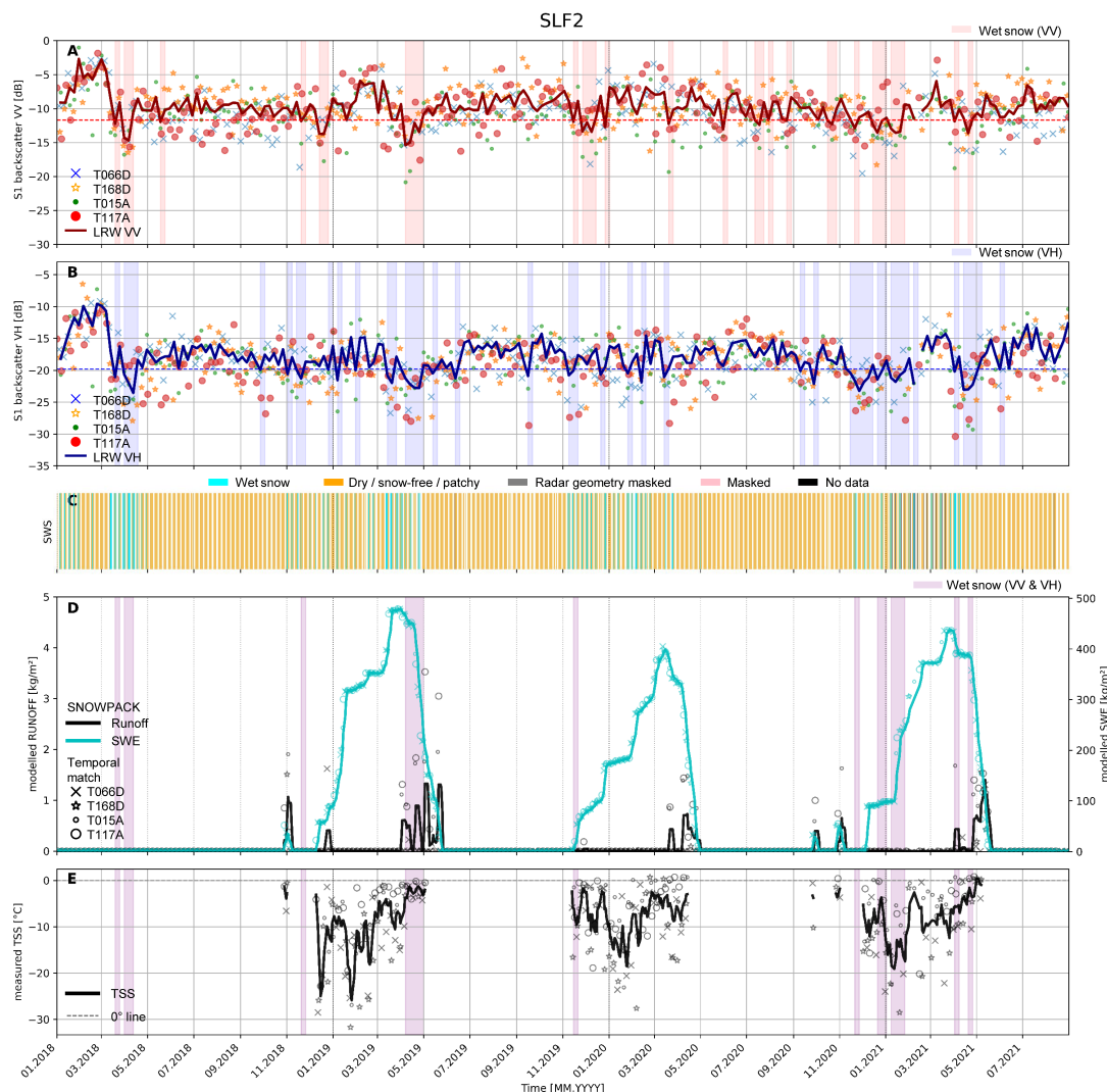
Figure A3. Time series of wet snow evolution over four melting seasons from January 2018 until August 2021 at SLF2 station. A) and B) show the time series extracted from the pixel within which the IMIS station is situated in co- (A) and cross-polarised (B) S1 data. The horizontal line indicates the time series median including the 2 dB threshold and the shading background displays the times during which the backscatter falls below this and wet snow is detected. C) SAR Wet Snow classified layer from Copernicus per each track over the station area. D) modelled time series of virtual lysimeter (MS SN RUNOFF) and snow water equivalent (SWE) from SNOWPACK data with markers indicating the corresponding time of S1 acquisition and the line being the mean between those four times. Similar E) shows the local measured snow surface temperature (TSS), masked to when snow height as non-zero. In D) and E), the applied purple shading corresponds to our wet snow combined polarisation product. D and only available from September 2018 due to a sensor failure before.
