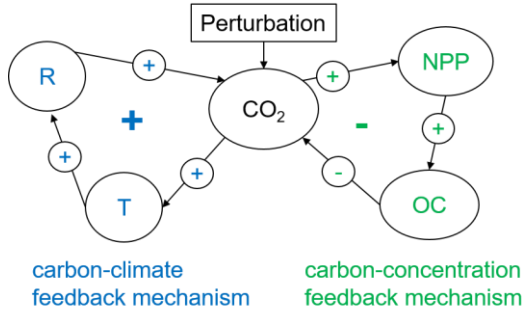
Figure 1: Feedback diagram for two main terrestrial biogeochemical feedback mechanisms. NPP: Net primary production, R: Respiration, OC: Land and organic carbon stocks, T: Global surface air temperature, CO 2 : Atmospheric carbon dioxide content.
