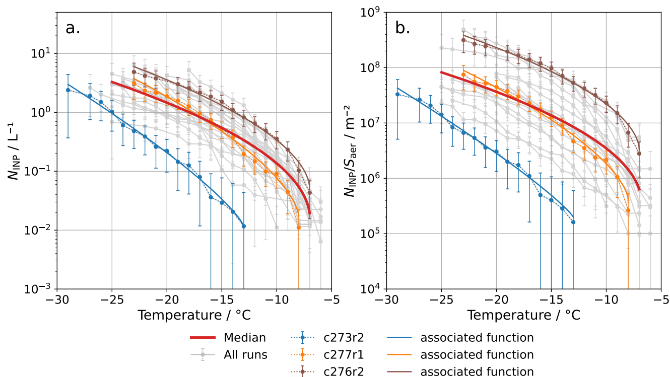
Figure 9. All measured temperature spectra for (a) INP concentration and (b) INP concentration normalised by aerosol surface area were fitted to Eq. 4 and 5 respectively. In both panels, examples of fits to a high, medium and low spectrum are demonstrated. In panel a, the red line shows the function fitted to the median INP concentration observed during the campaign, where \nu_{\text{INP}} = 1.480 \times 10^{-2} \text{ m}^{-2} , T_{\text{max}} = 266.2 \text{ K} , a = 1.271 \text{ K}^{-b} and b = 0.5 . In panel b, the red line shows the function fitted to the median active site density observed during the campaign, where \nu_{\text{S}} = 3.501 \times 10^5 \text{ L}^{-1} , T_{\text{max}} = 266.4 \text{ K} , a = 1.279 \text{ K}^{-b} and b = 0.5 .
