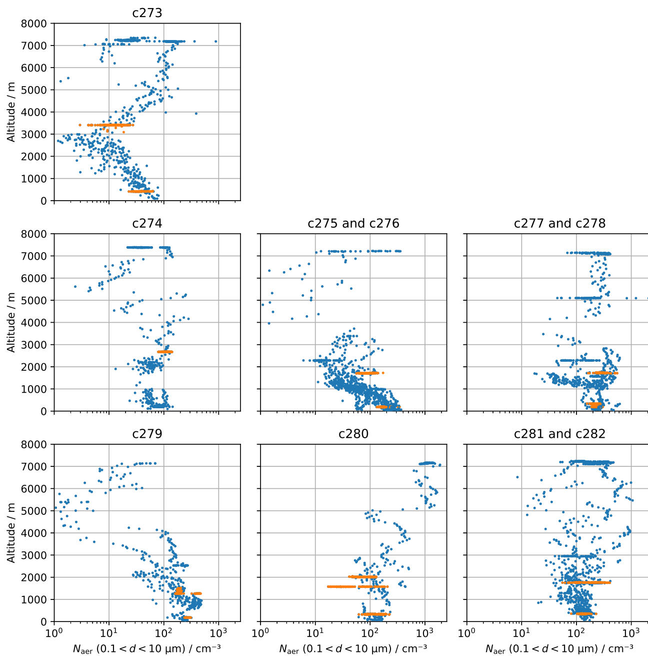
Figure 6. Out-of-cloud aerosol measurements made using the PCASP and CDP averaged every ten seconds. Measurements made during filter sampling are highlighted in orange. Measurements close to land were discarded to represent oceanic air only.
