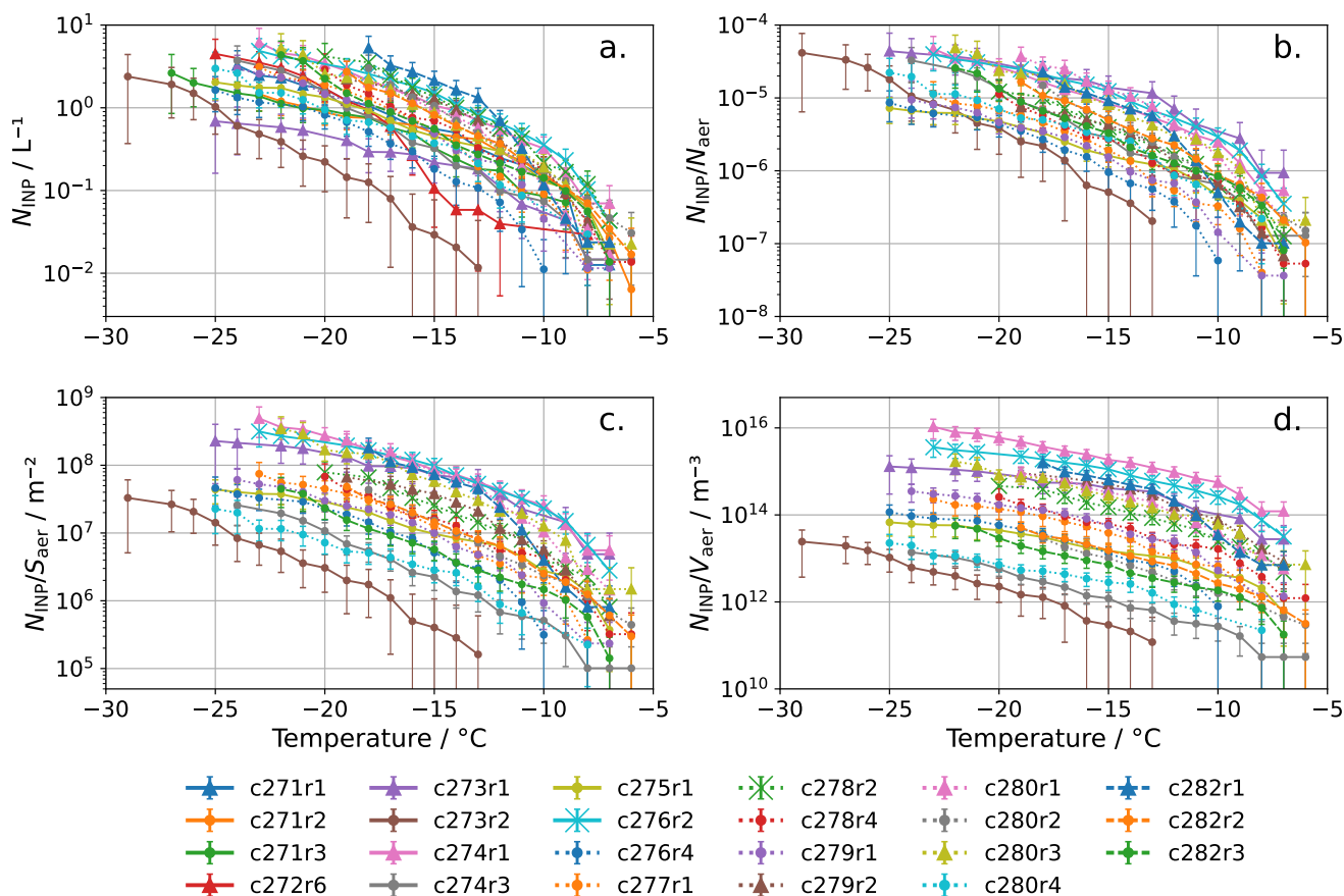
Figure 3. Panel a shows INP concentrations for each sample made during the campaign. Panels b , c and d show these concentrations normalised by the total number ( N_{\text{aer}} ), surface area ( S_{\text{aer}} ) and volume ( V_{\text{aer}} ) of aerosols with diameters greater than 0.1 \mu\text{m} . Colours and symbols of samples are consistent throughout all panels.
