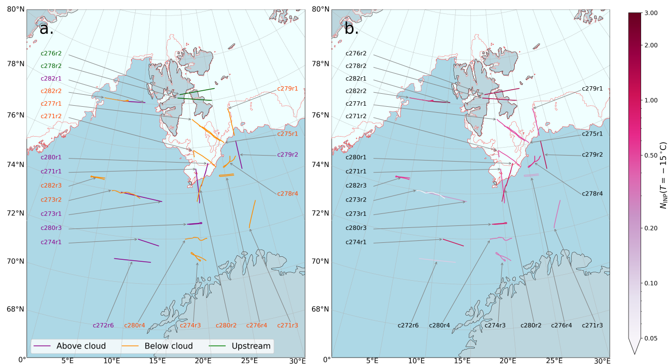
Figure 2. Locations of all filter samples taken during the ACAO campaign. Panel a displays the location of the sample relative to the cloud deck while panel b shows the temperature at which an INP concentration of 0.5 \text{ L}^{-1} was measured for each sample. All filters were taken in CAO conditions except c272r6 .
