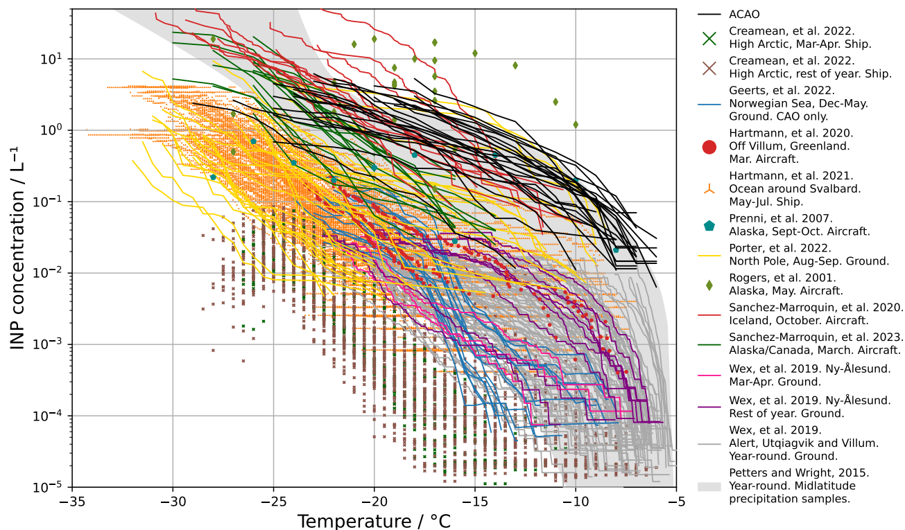
Figure 4. INP concentrations measured in a number of different field campaigns in the Arctic (Creamean et al., 2022; Geerts et al., 2022; Hartmann et al., 2020, 2021; Porter et al., 2022; Sanchez-Marroquin et al., 2020, 2023; Wex et al., 2019). These are compared to mid-latitude INP measurements from precipitation samples collated by Petters and Wright (2015).
