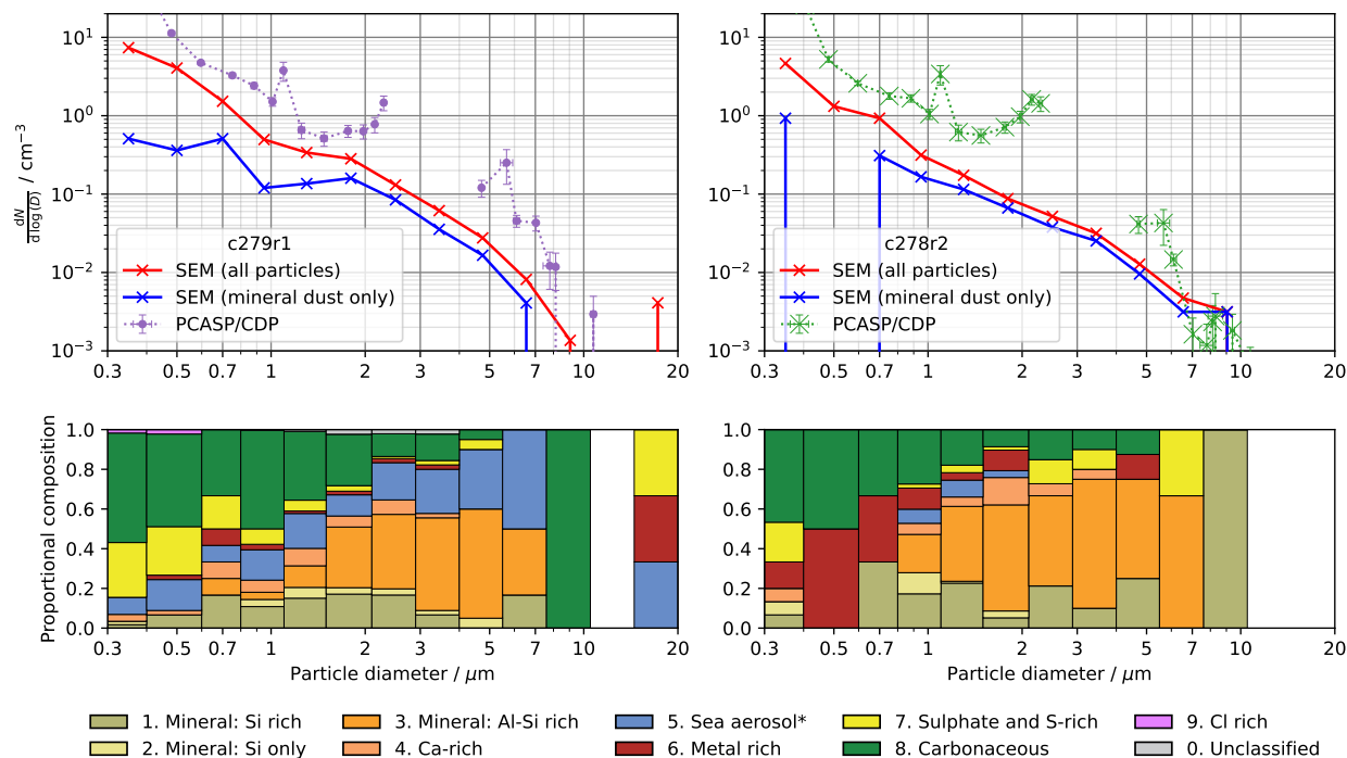
Figure 7. Particle-size distributions and particle composition derived from scanning electron microscopy for filters c279r1 (left) and c278r2 (right). Solid lines show particle-size distributions derived directly from the SEM measurements, while dotted lines show the particle-size distribution derived from the underlying probes in the diameter ranges, as in Fig. 5. Composition is shown for each size bin. Size bins with greater values of dN/d\log(D) contain more particles. White regions of the composition plots indicate that no particles were detected in this size range. Sea aerosol refers to aerosols likely to correspond to either fresh, aged or mixed sea spray aerosols.
