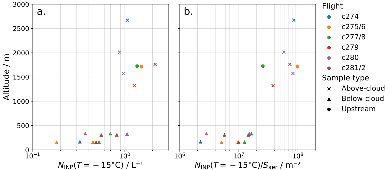
Figure 10. Variation with altitude of a INP concentration at -15^{\circ}\text{C} and b INP concentration at -15^{\circ}\text{C} normalised by aerosol surface area in northerly CAOs.
