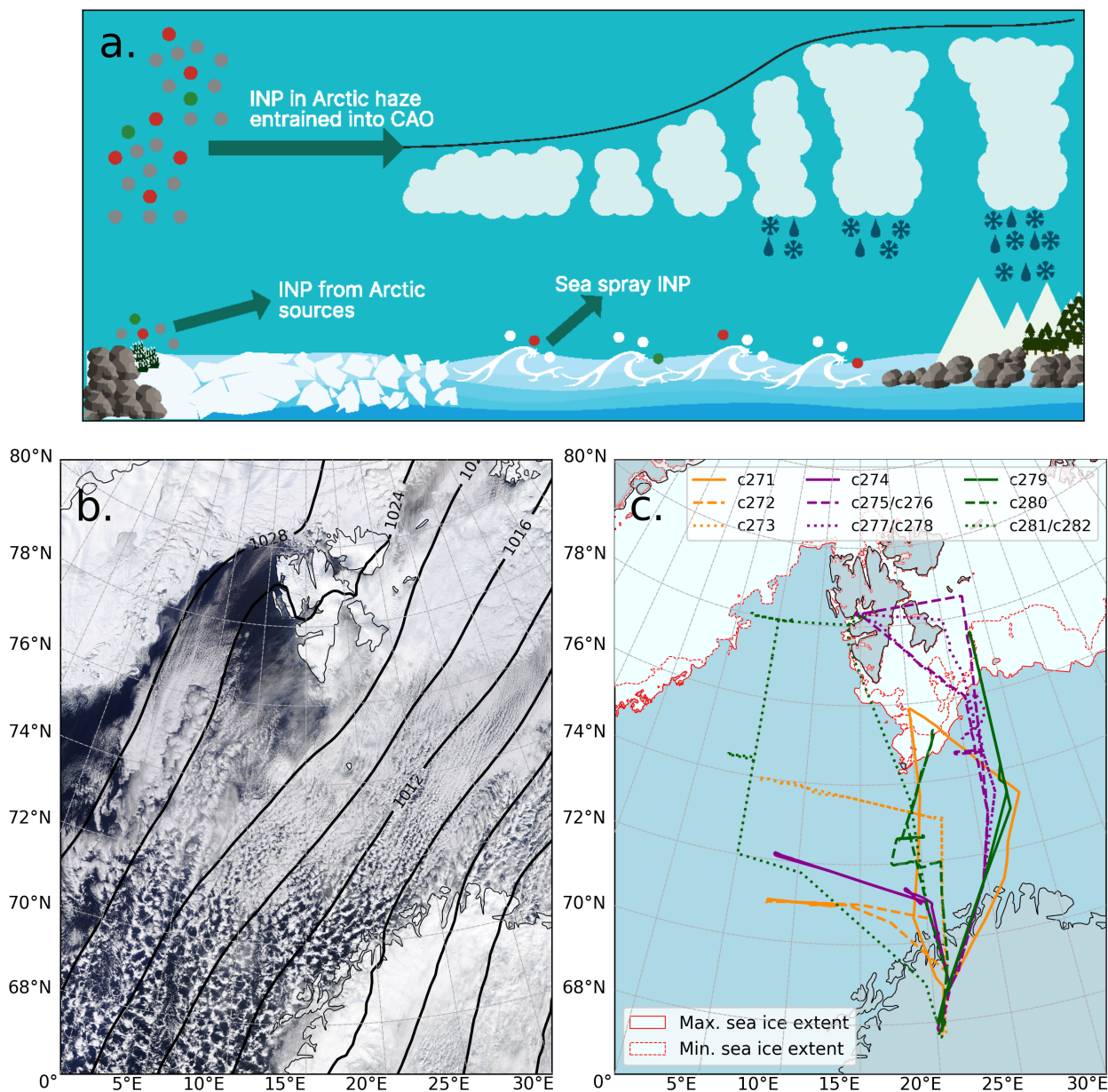
Figure 1. Panel a shows a schematic representation of an Arctic cold-air outbreak and the potential sources of aerosol to the cloud system. Stratiform cloud forms off the sea-ice edge and develops into cumulus cloud as the CAO airmass moves south. Biological and abiological INP are represented by green and red circles respectively, while aerosols that do not actively nucleate ice in CAOs are represented by grey and white circles. Panel b shows a satellite image taken on 30 March 2022 by the Moderate Resolution Imaging Spectroradiometer (MODIS) of a typical CAO measured during the ACAO campaign (MODIS Land Science Team, 2020). Sea-level pressure isobars from ERA5 reanalysis are overlaid (C3S, 2018). Panel c shows flight tracks from the nine flying days during the campaign. Sea-ice extent in this and other maps was obtained from the Multisensor Analyzed Sea Ice Extent dataset (U.S. National Ice Center et al., 2010). The flight track for flight c278 is incomplete due to equipment failure.
