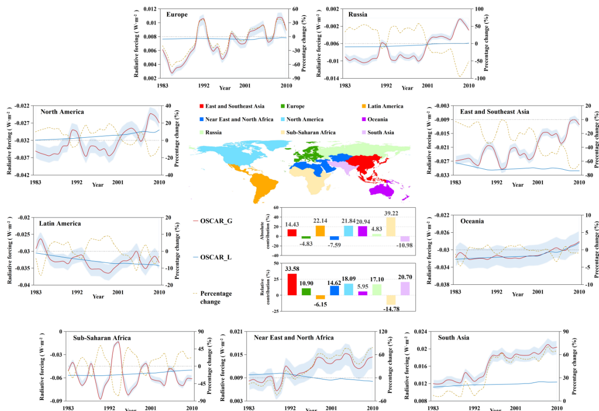
Figure 2. Annual RF ( \text{W}\cdot\text{m}^{-2} ) due to the albedo change and ARF percentage change between the two model scenarios S1 and S2 from 1983 to 2010 derived from LUH1-LUC inventory (solid blue line) and GLASS-GLC inventory (solid red line) in nine regions across the globe. The pale blue shading indicates the uncertainty interval estimated from Monte Carlo simulations. The dashed brown line stands for the percentage change in the annual \text{ARF}_{i-F} between the LUH1-LUC inventory ( \text{ARF}_{i-S1} ) and GLASS-GLC inventory ( \text{ARF}_{i-S2} ), in which i represents regions, respectively, including East and Southeast Asia, Europe, Latin America, Near East and North Africa, North America, Oceania, Russia, Sub-Saharan Africa, and South Asia. The first bar chart illustrates the absolute contribution of different regions to the global albedo-induced RF, and the second bar chart displays the relative contribution of different regions to the global albedo-induced RF changes. The nine color bars represent different regions, as indicated by the color legend above the colored sectional map.
