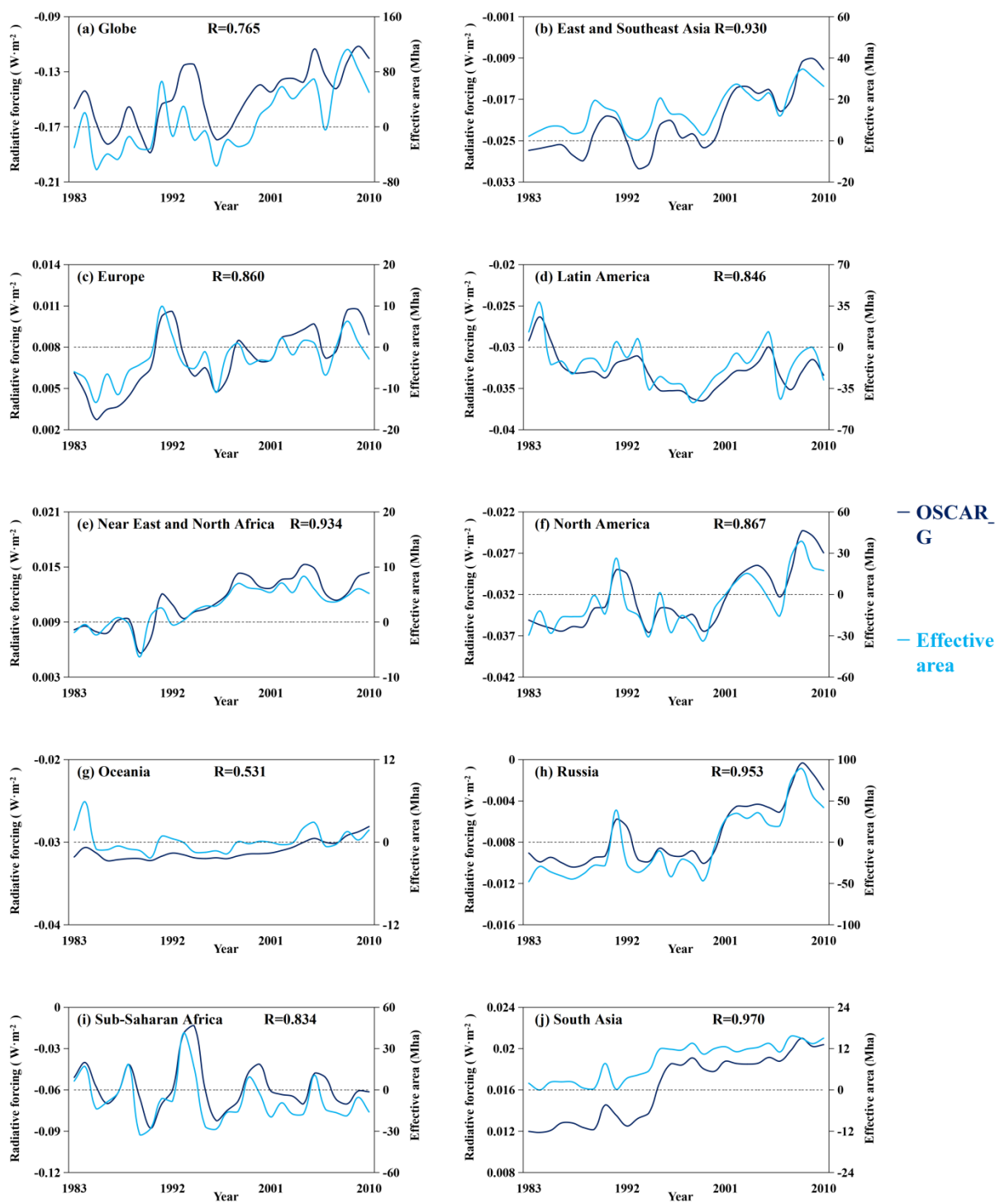
Figure 3. Annual RF ( \text{W} \cdot \text{m}^{-2} ) due to surface albedo change in model scenarios 2 from 1983 to 2010 derived from GLASS-GLC inventory (solid black line) and effective area (solid blue line) in the globe and nine regions. (a) Globe; (b) East and Southeast Asia; (c) Europe; (d) Latin America; (e) Near East and North Africa; (f) North America; (g) Oceania; (h) Russia; (i) Sub-Saharan Africa; (j) South Asia. Correlation
