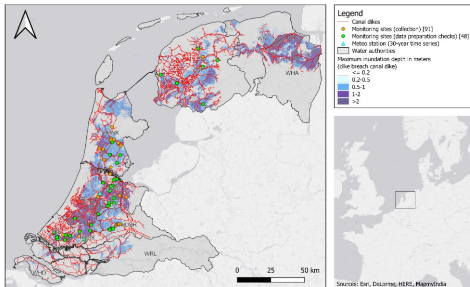
Figure 23 Overview of the study area with the canal dike system (subset within the regional flood defence system that are located in the provinces South-Holland, North-Holland, Friesland, Groningen and Utrecht). Monitoring sites are indicated by circle markers, with orange and green denoting collected data and the data checked and utilized for further analysis, respectively. Maximum inundation depths are depicted to illustrate potential flood impact in the polders.
