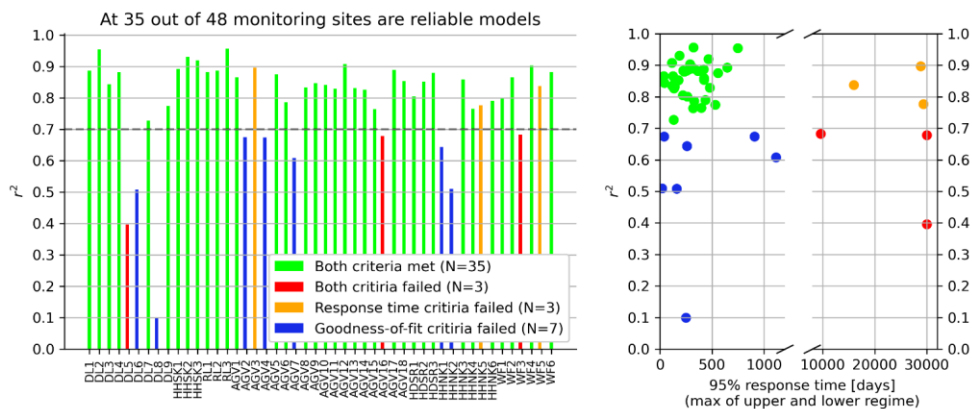
755 Figure A1. r^2 values of the best-performing TARSO models at each monitoring site, with colors indicating whether the models meet the reliability criteria. Right: Corresponding response times (maximum for both the upper and lower regimes) associated with the R^2 values.
