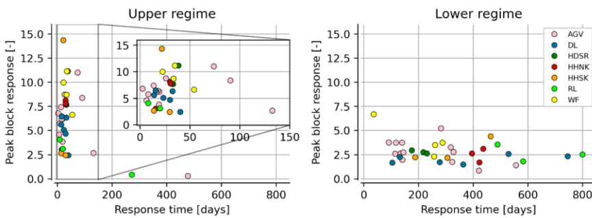
Figure 7 The characteristics of the impulse response functions at 33 canal dikes (peak of the block response and 95% response time) for the upper and lower regimes, where the colors indicate the various water authority regions where the dikes are located. The inset at the upper regime shows a zoomed-in view.
