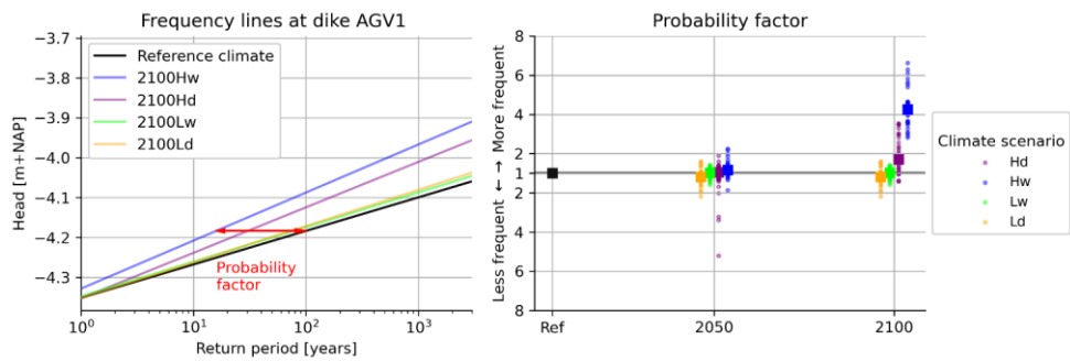
Figure 11.14 Left: The frequency lines of head levels for various climate scenarios in 2100 ( H igh/ L ow emissions; d ry/ w et regional climate response) at the dike in a polder south of Amsterdam. Right: the probability factor of all dikes (●) and the median value (■) for different time horizons and climate scenarios.
