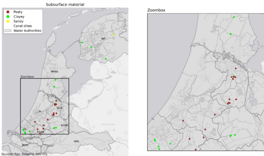
Figure A6. Mapping of subsurface material (peat, clay and sand) in the 35 canal dikes for which reliable models were developed across the Netherlands.
