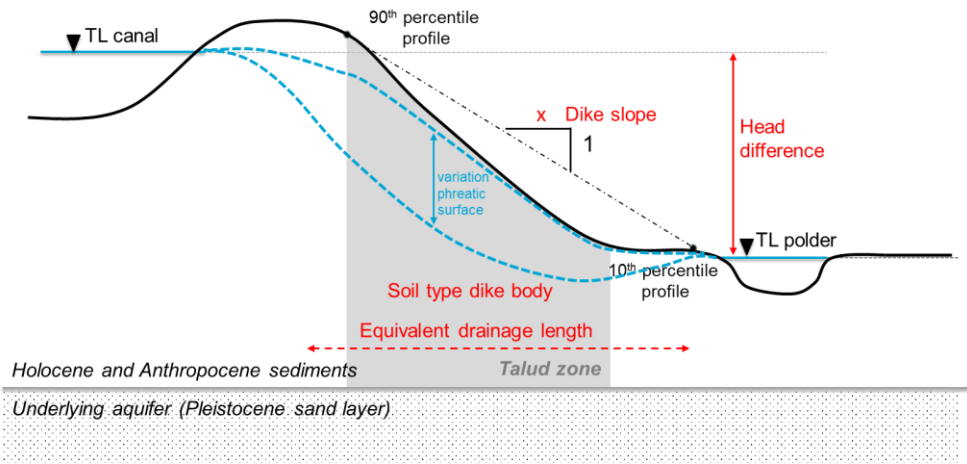
160 Figure 3-4 A simplified cross-sectional profile of a canal dike with regulated water levels (TL=target level) on both sides (canal and polder) and the variation in the phreatic surface (blue dashed lines). In this study, the groundwater levels in the talud zone of the
