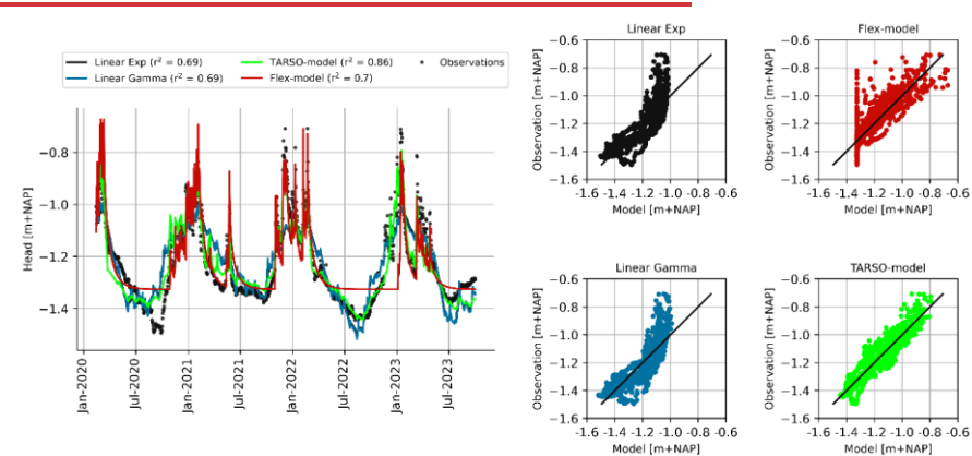
290 Figure 5 The performance of different model structures at Molenlaan (DL4). The left graph shows the simulated and observed head levels and on the right four scatterplots of the model structures showing the observed and simulated daily head levels (the black line indicates the 1:1 line).
