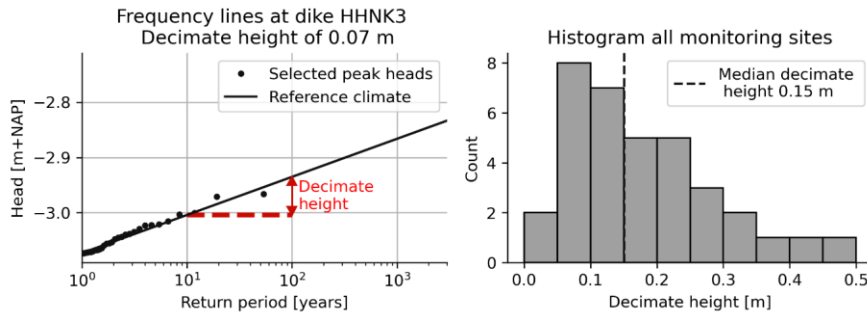
Figure 10 Left: Frequency lines of hydraulic head levels at a dike along the Beemster polder (HHNK3) based on precipitation and evaporation corresponding to the current climate. Right: a histogram of the decimate heights of all dikes considered of which the median decimate height is 15 cm.
