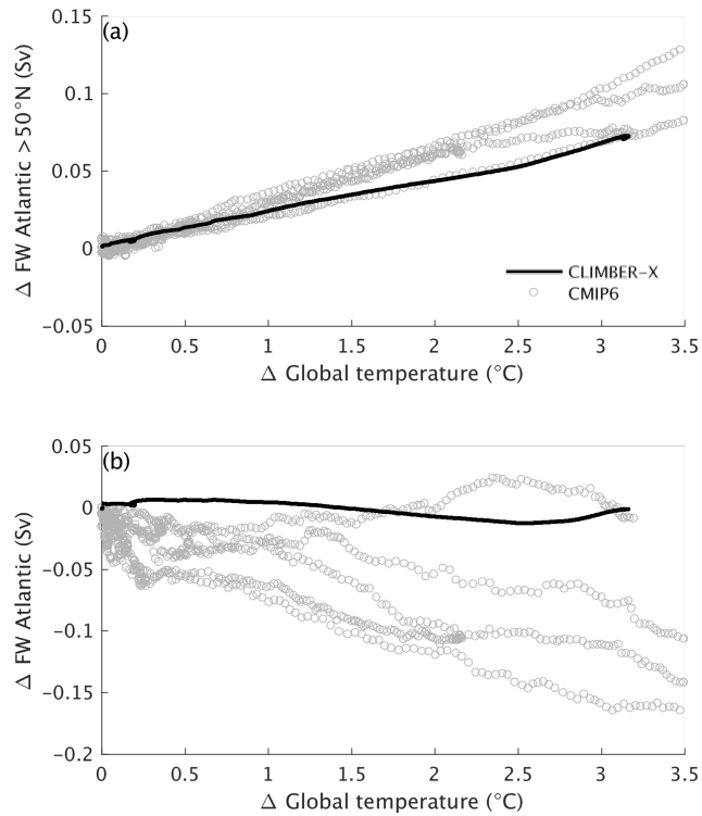
Figure B2. Change in the net freshwater flux into the ocean as a function of global temperature change in transient historical and future simulations under the SSP2-4.5 scenario until the year 2300 CE for (a) the northern North Atlantic and Arctic (north of 50^{\circ} N) and (b) the whole Atlantic ocean. The solid line is for CLIMBER-X results and the circles represent CMIP6 model results.
