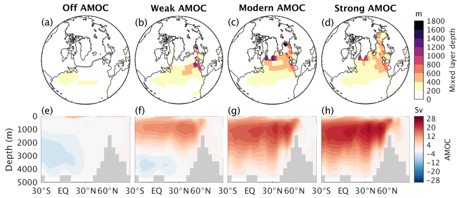
Figure 3. The different AMOC states. (a-d) Seasonal maximum Maximum monthly mean mixed layer depth of the year and (e-h) AMOC streamfunction for the different equilibrium AMOC states in the model: (a,e) Off , (b,f) Weak , (c,g) Modern and (d,h) Strong AMOC states. The grey line in (a-d) shows the seasonal maximum monthly mean sea ice extent of the year (defined as sea ice concentration >0.15 ). The shown AMOC states are all for the same boundary conditions of 400 ppm of atmospheric \text{CO}_2 and a FWF of +0.05 Sv, i.e. for the boundary conditions under which all four AMOC states co-exist in the model (Fig. 5).
