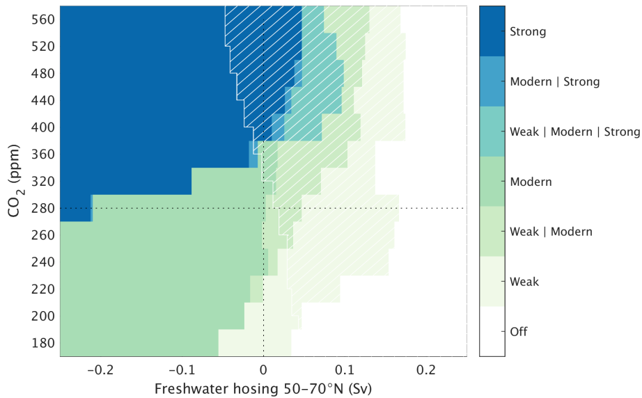
Figure 5. Summary of AMOC stability landscape in combined CO 2 and freshwater space. The colored regions indicate the on AMOC states that are stable under the given CO 2 and FWF as indicated in the legend. The crosses indicate the filled white area indicates where only the Off-Off AMOC state is stable, while the white hatched area shows the domain where the Off AMOC state and one or more of the three 'on' AMOC states coexist . Note that multiple AMOC states are stable under some boundary conditions.
