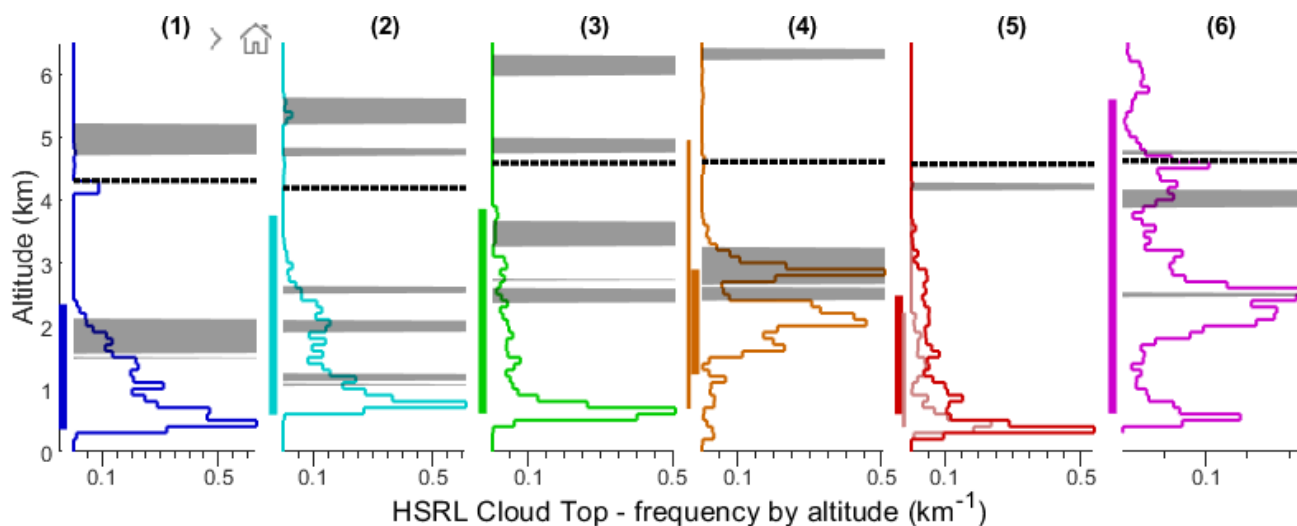
1245 Figure 6: Frequency distributions of HSRL detected cloud tops for Cases 1-6. Frequency data are normalized by the total available records within the module, such that an integration of the distribution results in the HSRL cloud fraction (Table 2). Also shown are regions where d\theta/dz exceeds 6 \text{ K km}^{-1} as an indicator of stable layers (grey shading), and the 0^\circ\text{C} level (dashed). The vertical bar adjacent to each case indicates the span of altitudes sampled in situ by the Falcon, and in panel (4) and (5), the altitude span for the secondary Falcon modules (thin bar, Cases 4B and 5A, respectively).
