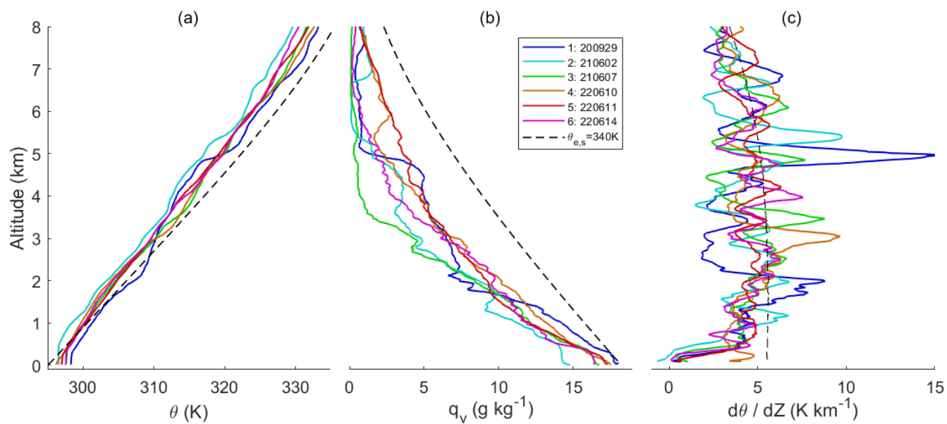
1230 Figure 4: Case-mean dropsonde profiles of (a) potential temperature, (b) water vapor mixing ratio, and (c) static stability (defined as the vertical gradient of potential temperature and smoothed over a 100 m window). The profile of a reference wet adiabat corresponding to a saturation equivalent potential temperature ( \theta_{e,s} ) at 340 K is also shown.
