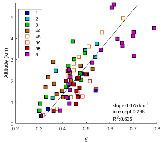
1275 Figure 10: Profiles of DSD relative dispersion, \epsilon , for Cases 1-6. Values of \epsilon are calculated locally at the measurement interval (1s, \sim 100 m) and then averaged (weighted by N_d ) across a transect.
