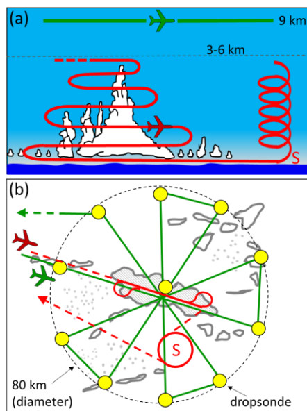
1205 Figure 1: Schematic of the nominal two aircraft flight strategy illustrating the position of the King Air (green) and the Falcon (red): (a) Cross section view of the altitude profile flown through the target cloud with adjacent clear spiral (S), and (b) plan view showing the “wheel and spoke” pattern.
