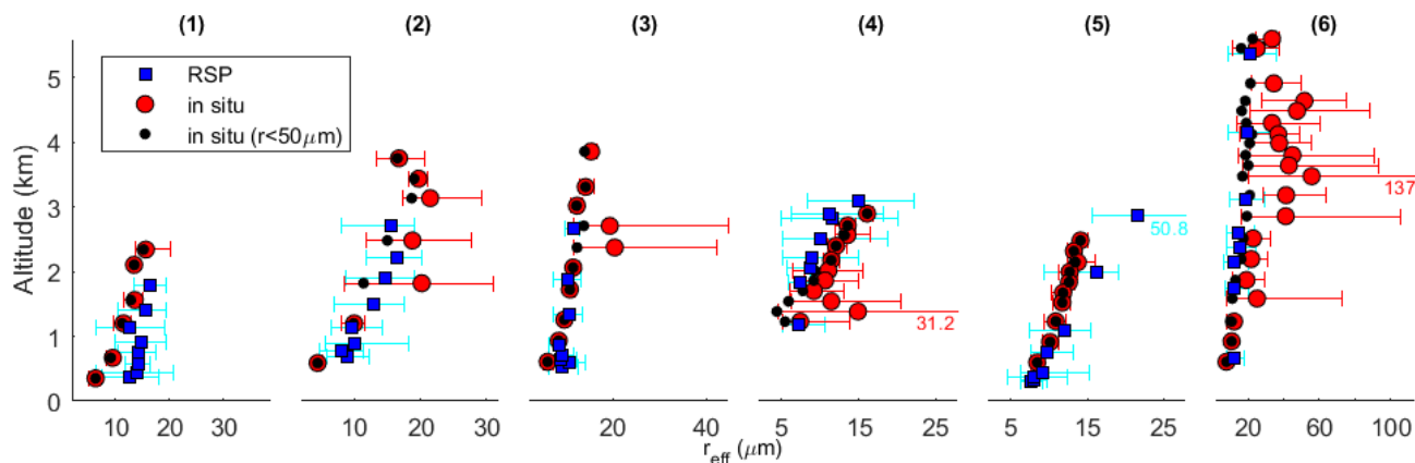
1285 Figure 12: Comparison of the vertical profile of effective radius, r_{\text{eff}} , for Cases 1-6 between Falcon in situ cloud transects and composite profiles from RSP. The composite profiles were derived by grouping RSP retrievals into eight equal frequency bins of cloud top height as determined by HSRL, with the mean altitude of each bin displayed. A comparison is made with in situ derived r_{\text{eff}} omitting contributions from rain water ( r < 50 \mu\text{m} ). For both datasets, the mean (markers) and 10-90% range (bars) are shown.
