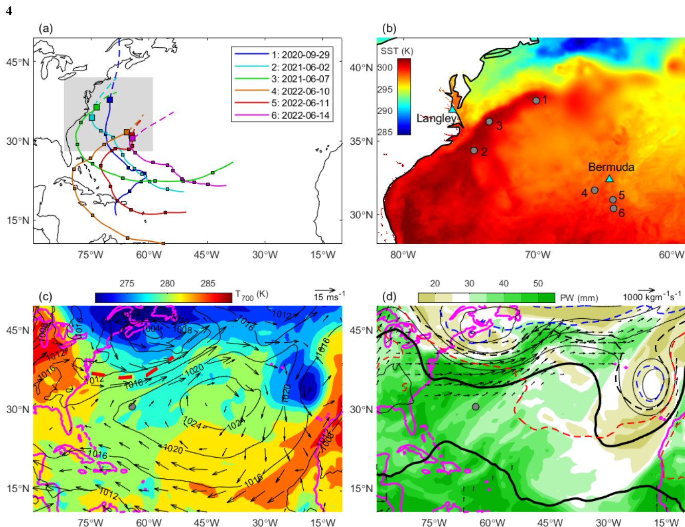
Figure 2: Large-scale meteorological environment. (a) 8-day back trajectory (solid) and 1-day forward trajectory (dashed) using MERRA-2 800-950 hPa layer averaged winds (see text) for Cases 1-6. (b) Example SST shown for Case 6 (2022-06-14) with all case locations shown for reference. The region in (b) corresponds to the grey shaded region of (a). (c) Case 6: sea-level pressure (contours), 850 hPa wind vectors, and 700 hPa temperature (colored). The location of the axis of the stationary front (see text) is shown as the thick red dash. (d) Case 6: 500 hPa geopotential height (contours at 6 dm intervals, thick contour designates the 588 dm level), 1000-500 hPa thickness (dashed contours at 6 dm intervals, black contour designates the 564 dm thickness line, red (blue) contours represent regions of higher (lower) thickness), PW (colored), and MF (vectors).
