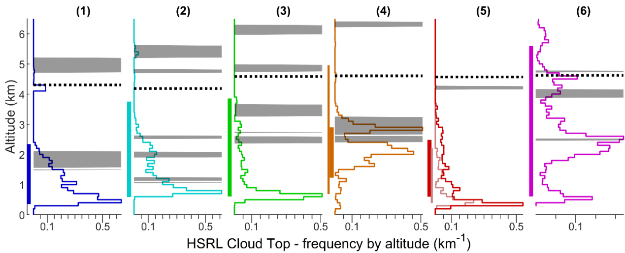
1265 Figure 6: Frequency distributions of HSRL detected cloud tops for Cases 1-6. Frequency data are normalized by the total available records within the module, such that an integration of the distribution results in the HSRL cloud fraction (Table 2). Also shown are regions where d\theta/dz exceeds 6 \text{ K km}^{-1} as an indicator of stable layers (grey shading), and the 0^\circ\text{C} level (dashed). The vertical bar adjacent to each case indicates the span of altitudes sampled in situ by the Falcon, and in panel (4) and (5), the altitude span for the secondary Falcon modules (thin bar, Cases 4B and 5A, respectively).
