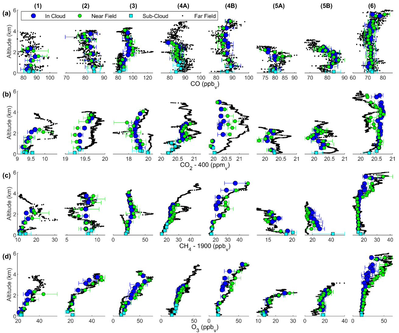
Figure 13: Trace gas vertical profiles separated into a far-field component measured during the Falcon clear spiral (black), a near-field component measured outside but in the vicinity of the cloud cluster at cloudy altitudes (green), an in-cloud component (blue), and a sub-cloud component (cyan). Data are shown for Cases 1-6 for (a) CO, (b) CO 2 , (c) CH 4 , and (d) O 3 . Note the changes in concentration scales.
