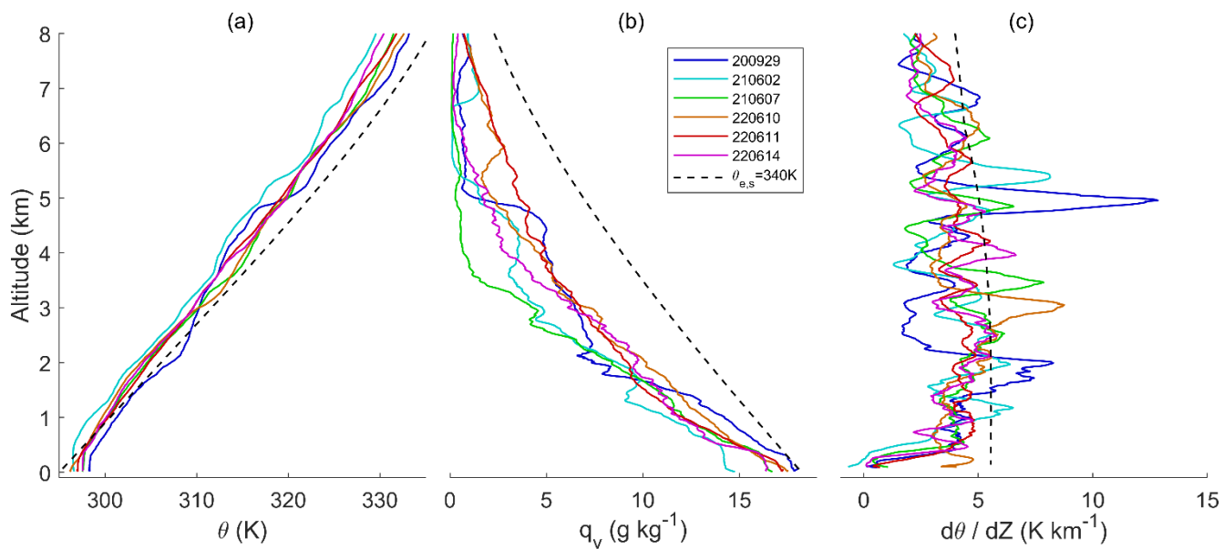
1250 Figure 4: Case-mean dropsonde profiles of (a) potential temperature, (b) water vapor mixing ratio, and (c) static stability (defined as the vertical gradient of potential temperature and smoothed over a 100 m window). The profile of a reference wet adiabat corresponding to a saturation equivalent potential temperature ( \theta_{e,s} ) at 340 K is also shown.
