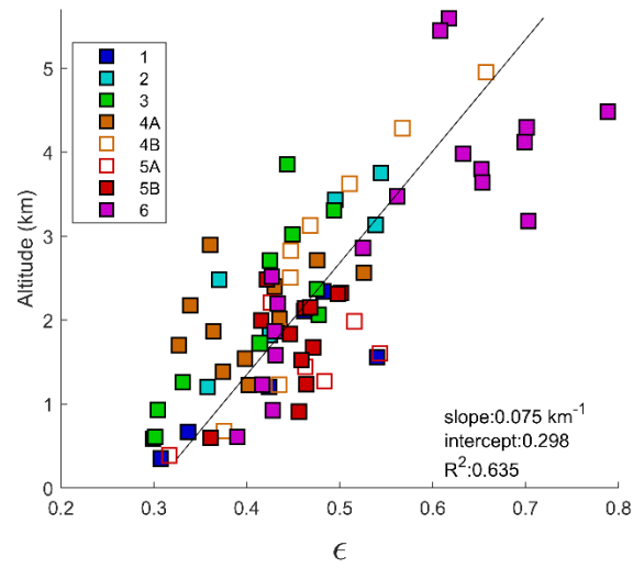
Figure 10: Profiles of DSD relative dispersion, \epsilon , for Cases 1-6. Values of \epsilon are calculated locally at the measurement interval (1s, ~100 m) and then averaged (weighted by N_d ) across a transect.
