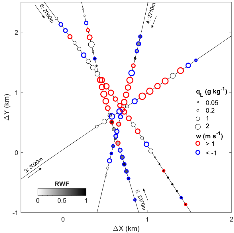
Figure 11: Four sequential Falcon in situ transects (2-3 km altitude) through cloud during Case 3. The aircraft position has been projected onto a cloud-centric coordinate where X (Y) represents the displacement along (perpendicular to) the cluster motion. The size of the markers corresponds to the total q_L with shading indicating the rainwater fraction (RWF) defined as the fraction of q_L resulting from drop diameters exceeding 100 \mu\text{m} . Red (blue) rings indicate updrafts (downdrafts).
