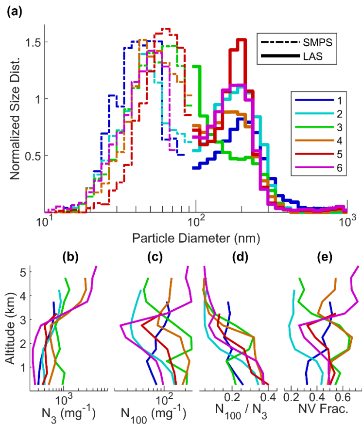
Figure 15: Aerosol microphysical properties for each case. (a) Normalized particle size distributions in the sub-cloud region, profiles of (b) total particle number concentration (>3 nm), (c) total particle number concentration (>100 nm), (d) the number fraction >100 nm, and (e) non-volatile number fraction (>10 nm).
