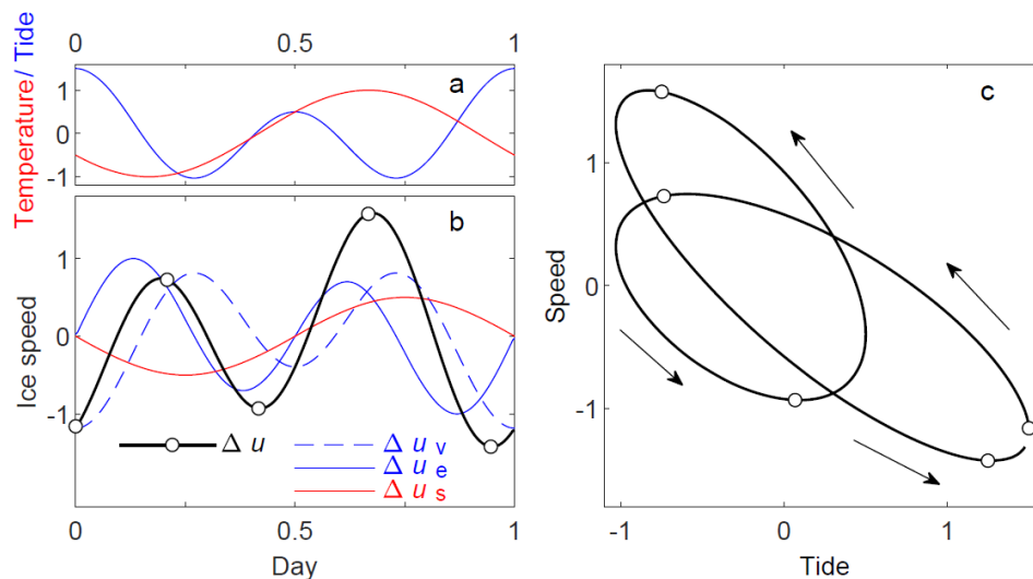
405 Figure 8. (a) Diurnal variations in tidal height (blue) and temperature (red) prescribed by Equations (1) and (2). (b) Ice speed computed by Equation (3) (black) as the sum of the perturbations due to viscous (dashed blue line), elastic (solid blue line) responses to tide, and sliding enhanced by meltwater (red). The open circles show local minima and maxima, which correspond to those indicated in (c). (c) Diurnal variations in ice speed and tidal height. The arrows indicate the time sequence of the data. The variations 410 in the tide, temperature and ice speed are in arbitrary units.
