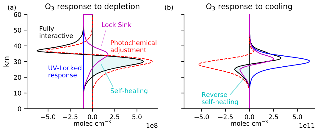
Figure 6. The Chapman+2 model response to the same perturbations as in Fig. 4, i.e. (a) ozone depletion by 10^8 \text{ molec cm}^{-3} everywhere below 60 km and (b) uniform cooling of 10 K. The Chapman+2 model reproduces the response structure calculated using the Cariolle v2.9 linear ozone model. The Chapman+2 model also permits the calculation of a Lock Sink response (magenta), for which only J_{O_3} was locked while J_{O_2} was allowed to adjust to the overhead ozone, emulating the conventional explanation for self-healing and reverse self-healing, yet failing to reproduce key aspects of the Fully Interactive response.
