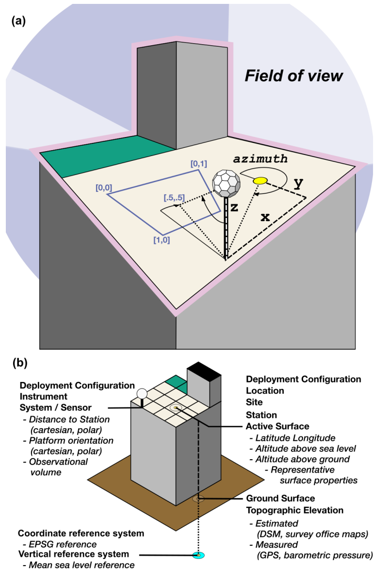
Figure A1. Deployment on a building roof with the relations between (a) a local station, platform, instrument, recorded image and related coordinate systems in polar and Cartesian coordinates, and (b) local and global coordinate reference systems as well as features in ordinance inventory and Earth Observation.
